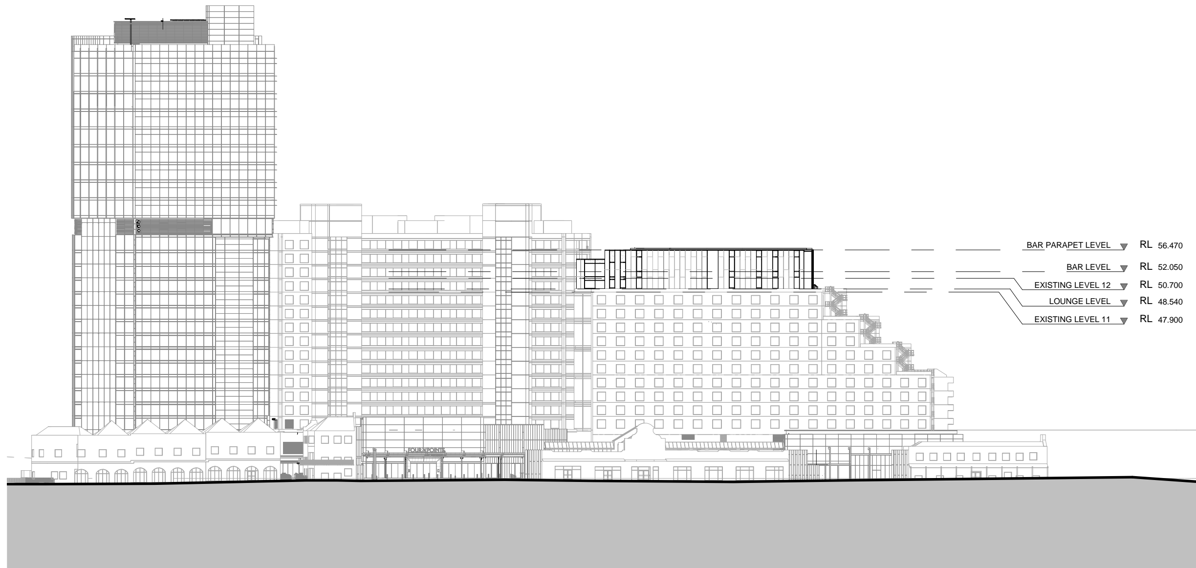
1 GENERAL ARRANGEMENT - EAST ELEVATION SCALE 1 : 750
