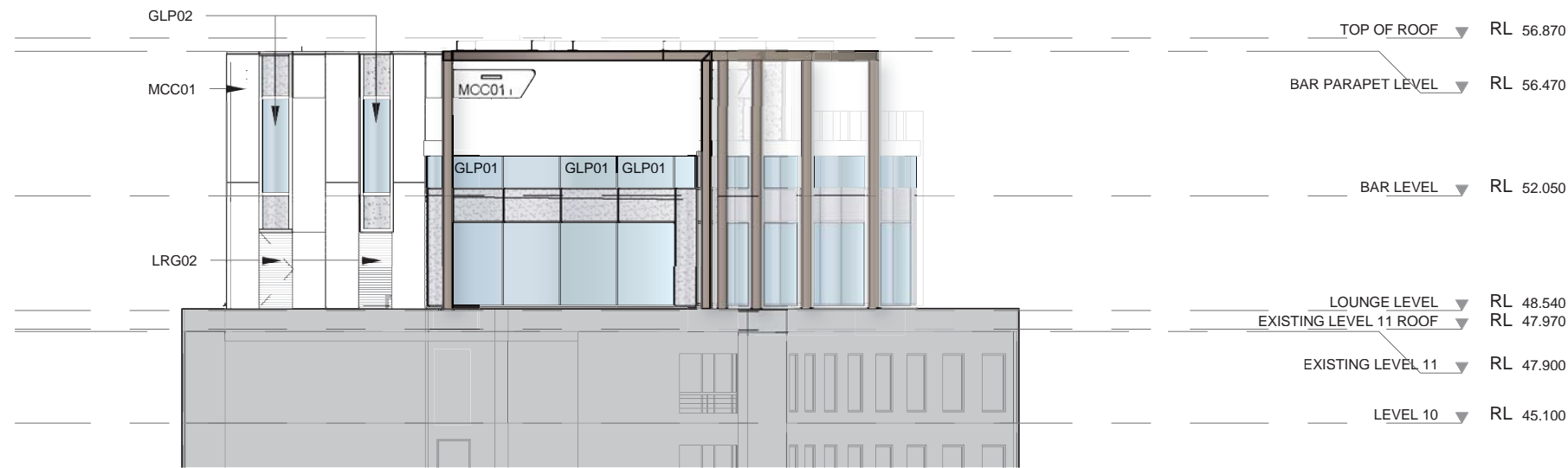
1 NORTH ELEVATION ZB-A-21-10 SCALE 1:200
