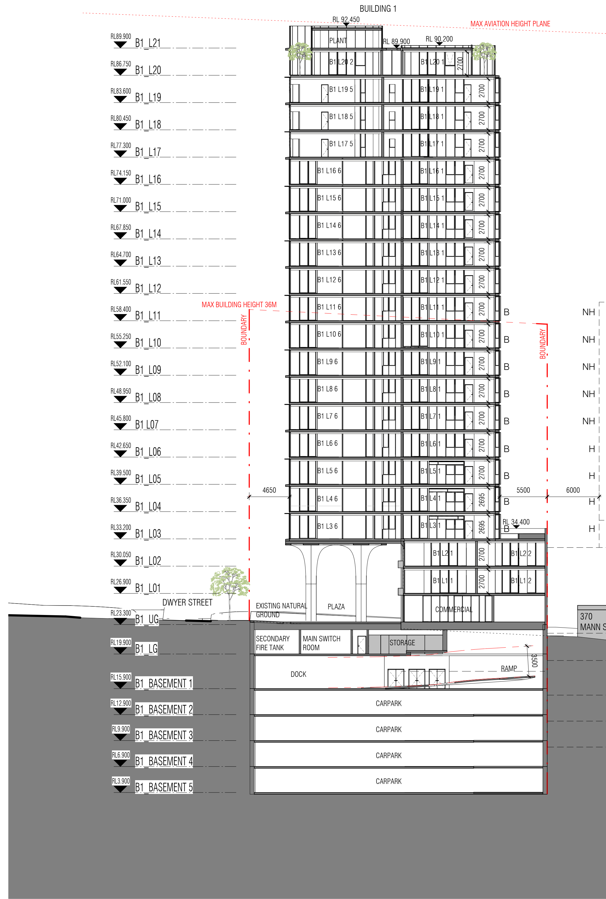
G SECTION GG SCALE 1:250
