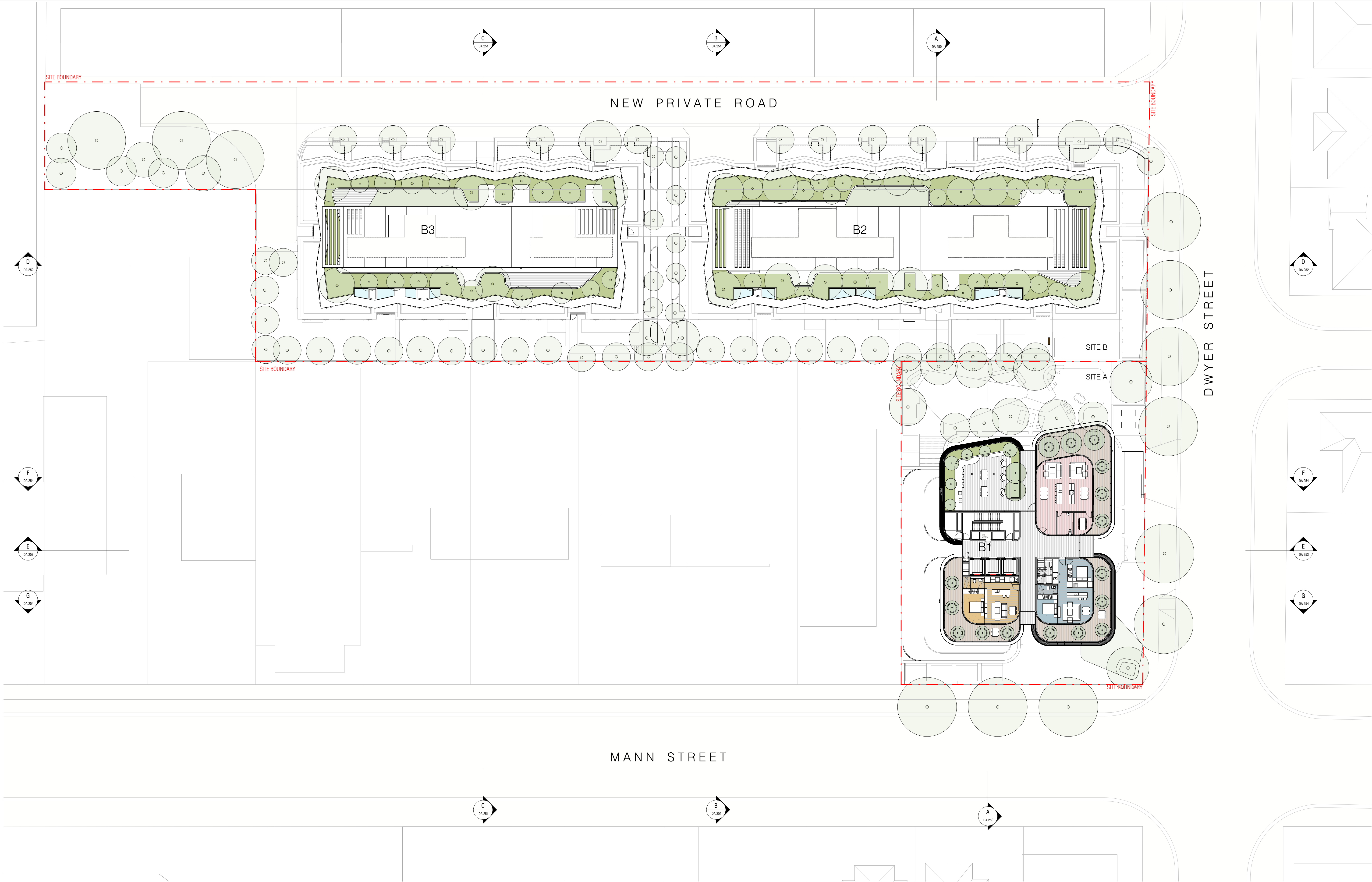
1 LEVEL 20 PLAN SCALE 1 : 250
