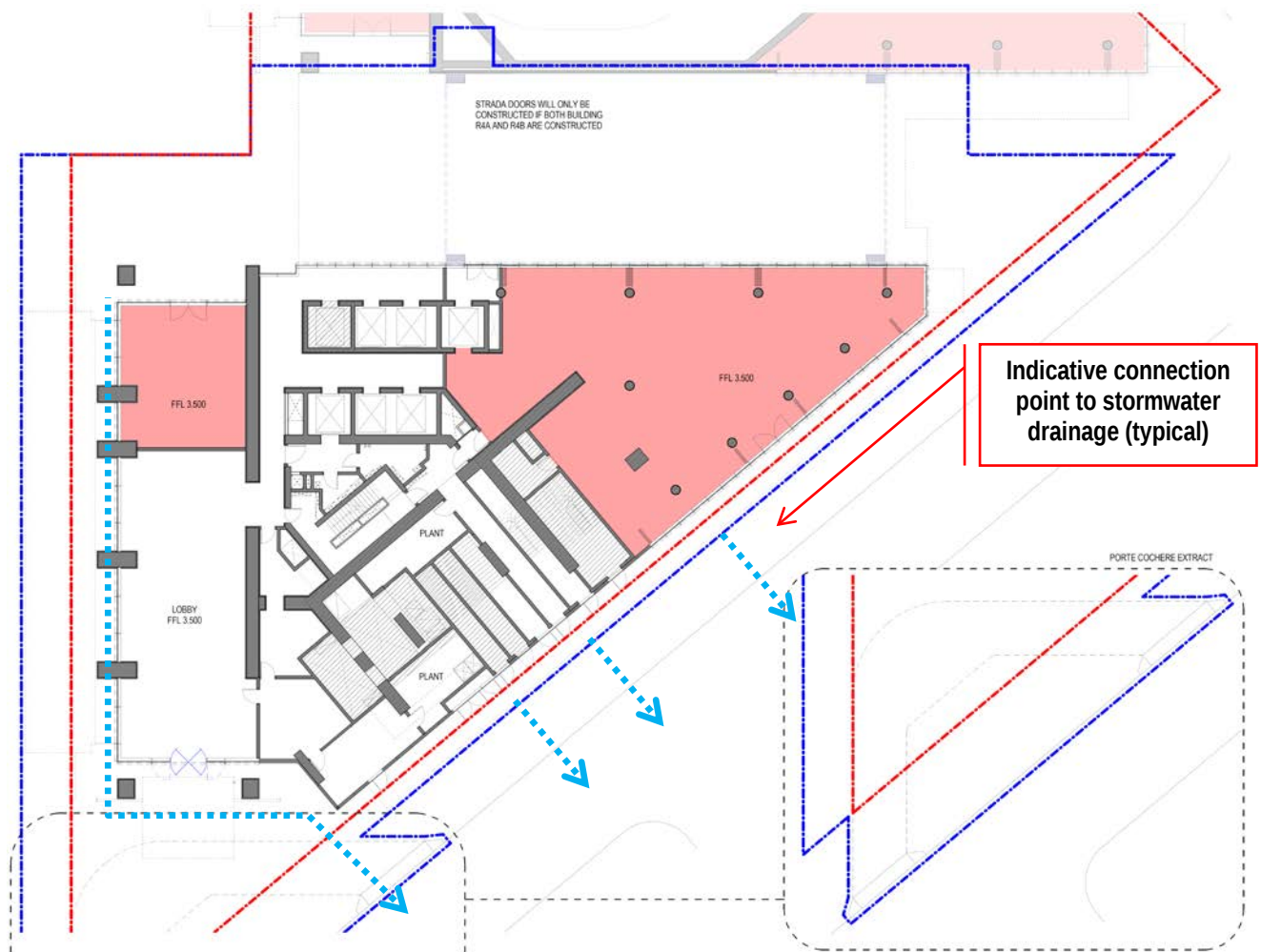
Figure 7.2: Indicative location of connections to Stage 1B internal drainage
