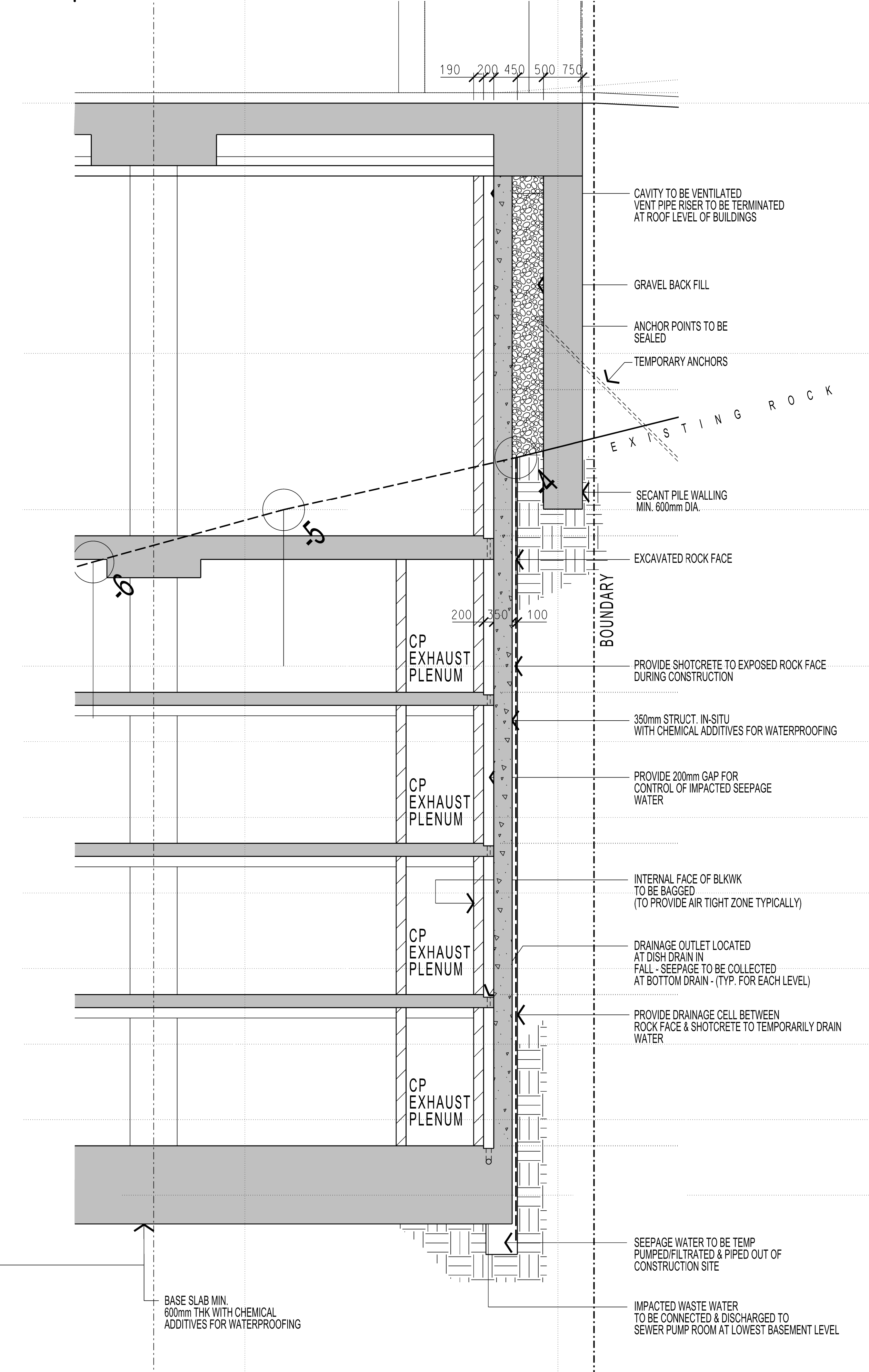
03 SECTION SCALE 1:50 REF
