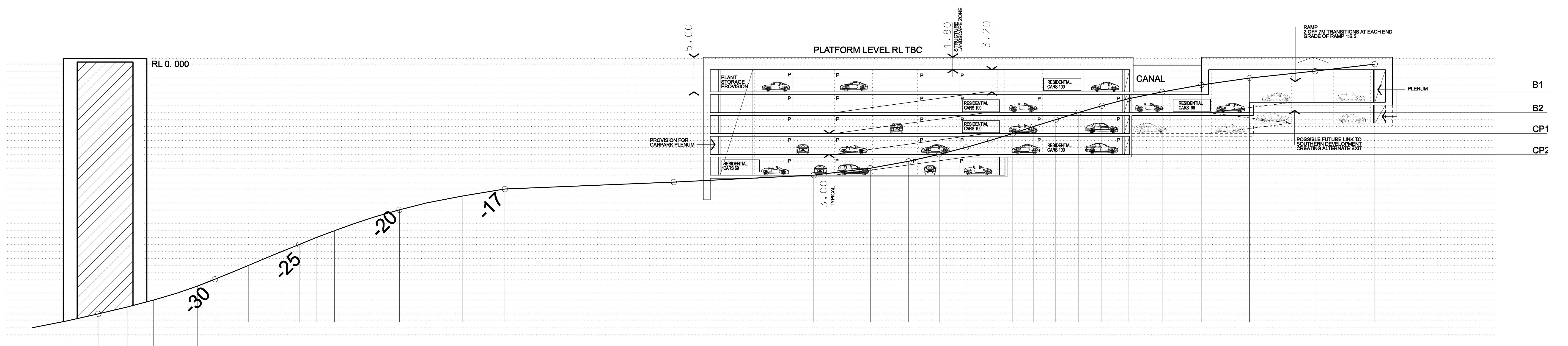
2 SECTION THROUGH BASEMENTS SK 104 SCALE 1:250 REF sxa 01
