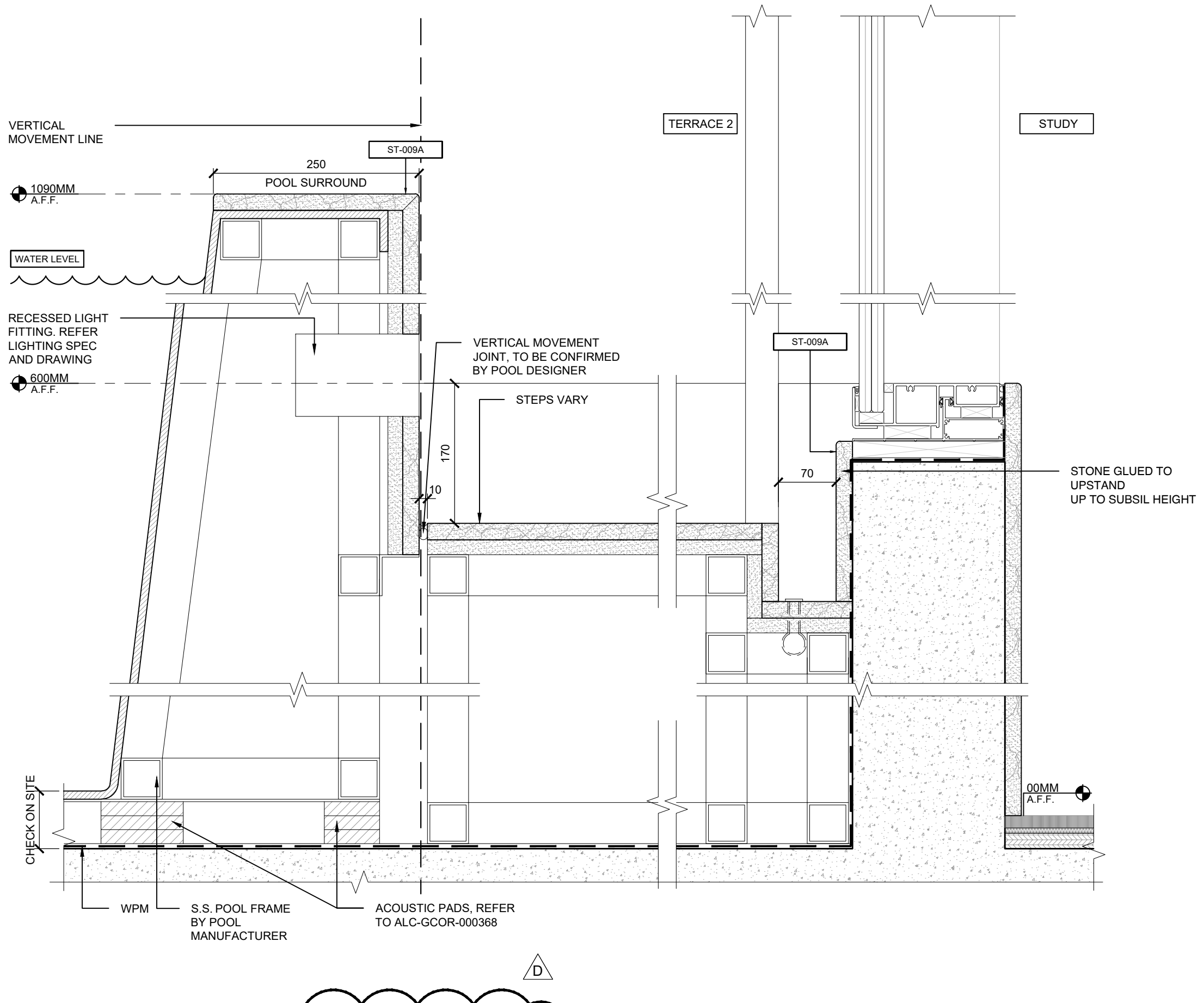
2 SECTION B-B SCALE:1:5
