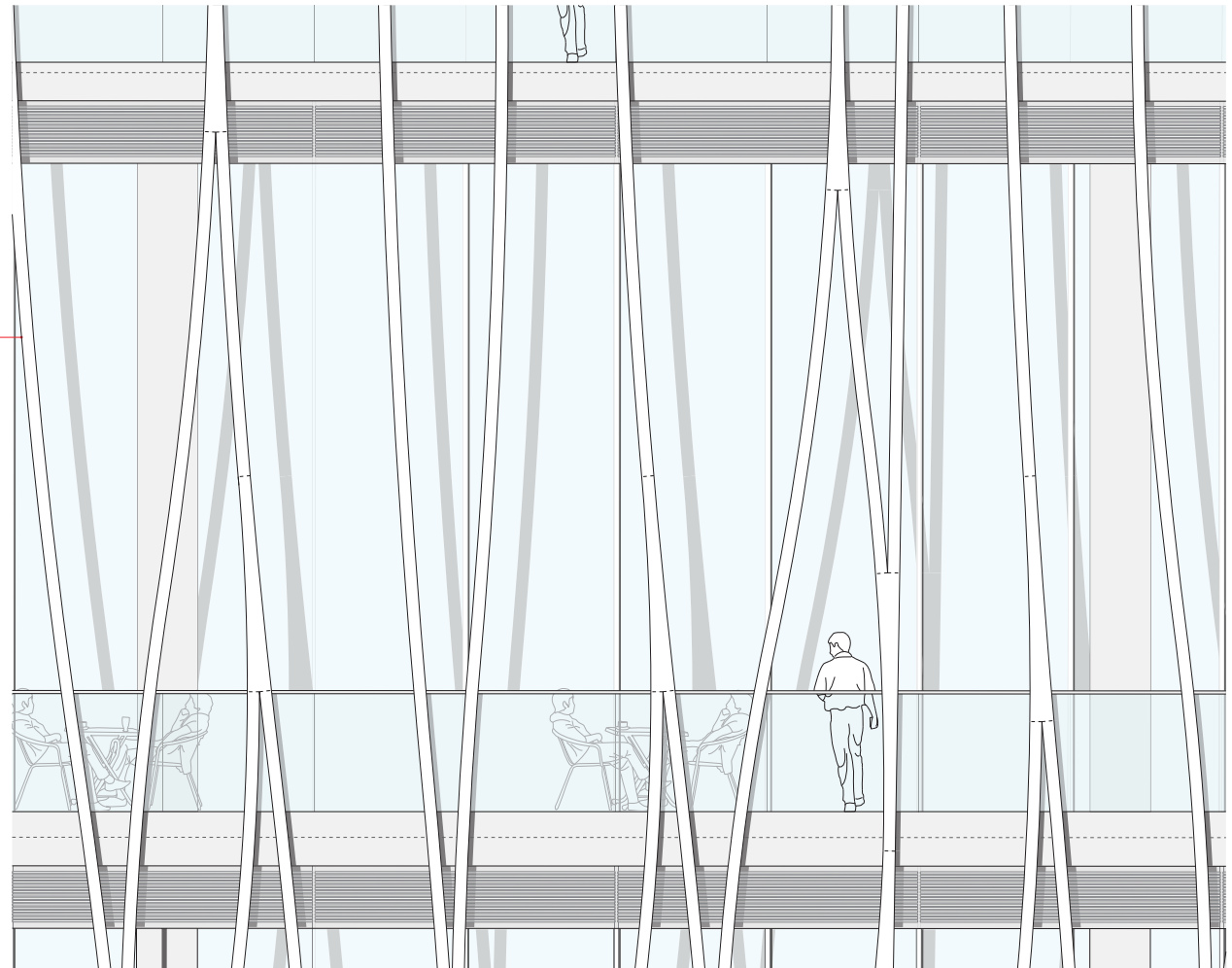
West façade partial elevation
