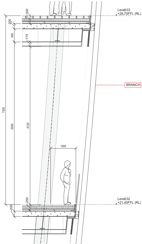
West façade partial section
