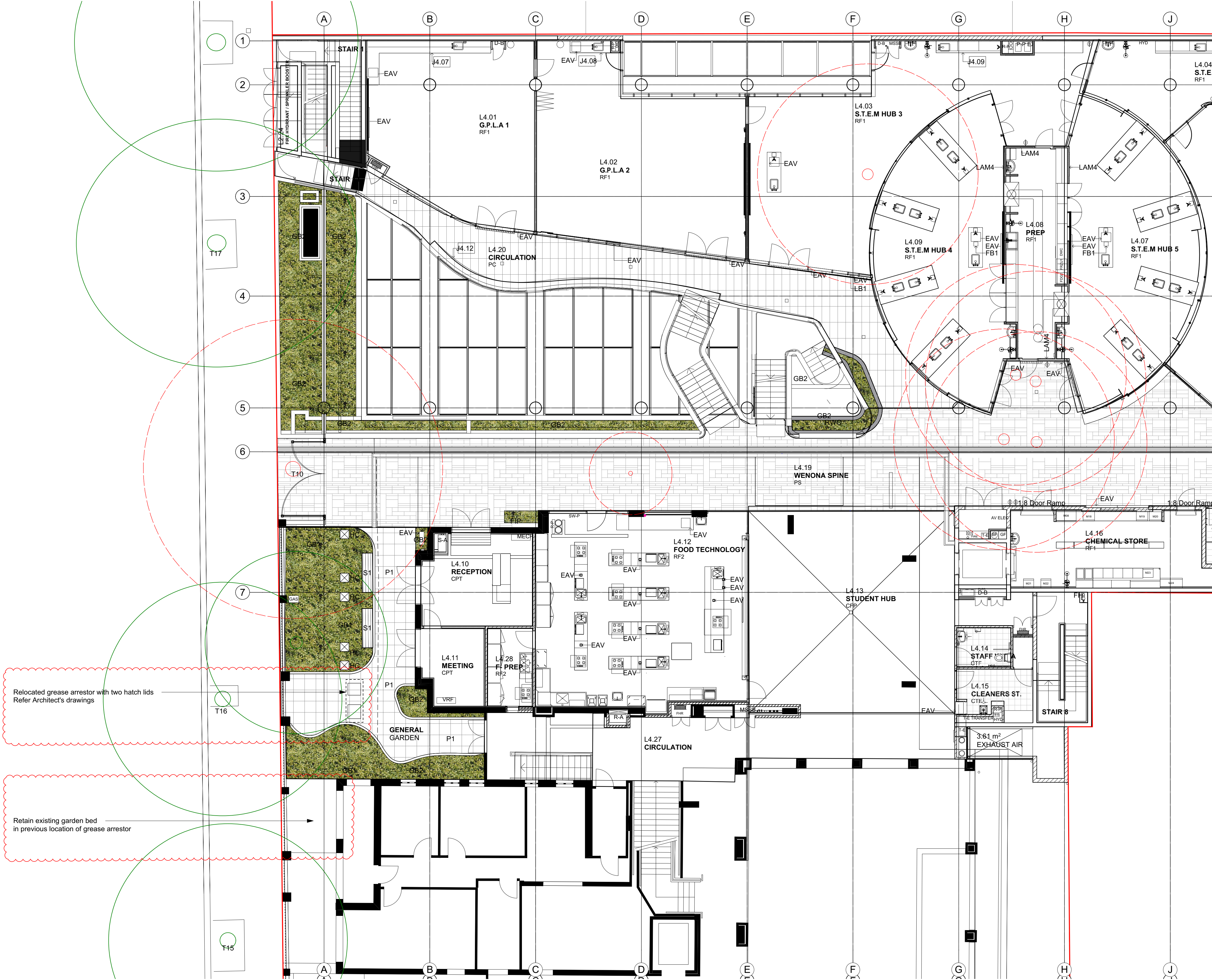
1 Plan: Level 4 Landscape Scale 1:100
