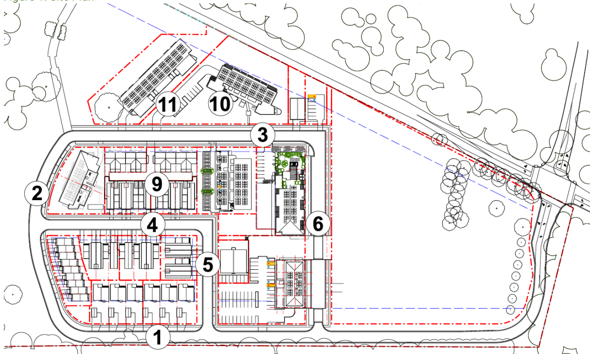
Figure 1: Site Plan
