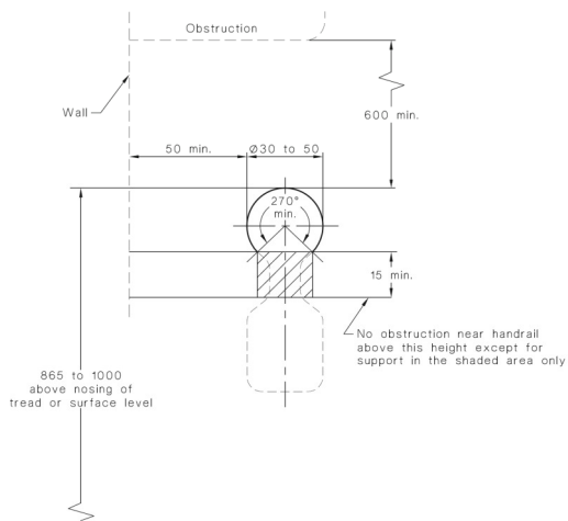
Figure 7: Handrail Details
