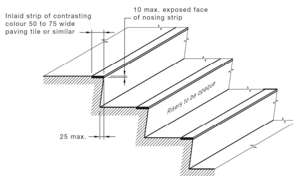
Figure 10: Nosing Details
