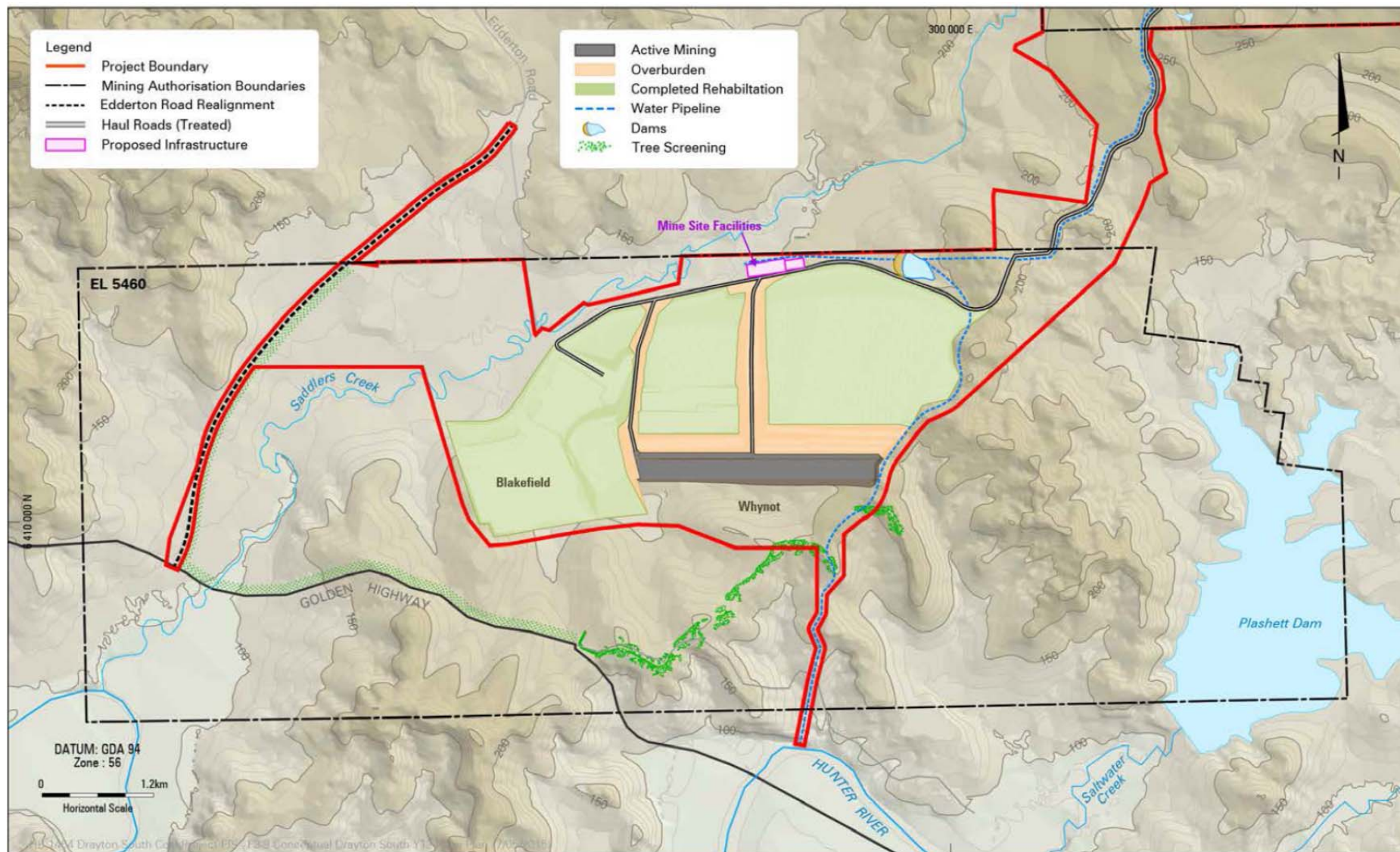
Figure 2E: Year 12 Mine Plan
