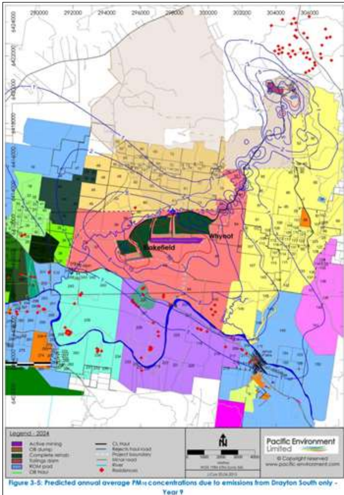
FIGURE 4 - PREDICTED ANNUAL PM 10 CONCENTRATION YEAR 9 - PROJECT ONLY
