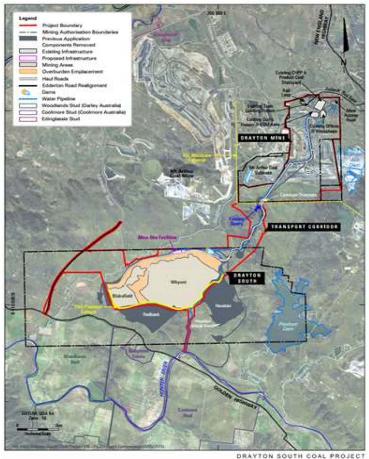
FIGURE 1 - DRAYTON SOUTH COAL PROJECT SITE
