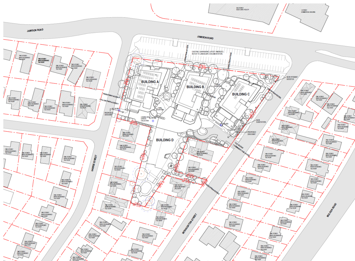
Figure 1.3 Site plan showing proposed building locations. (Source: Jackson Teece 2024)
