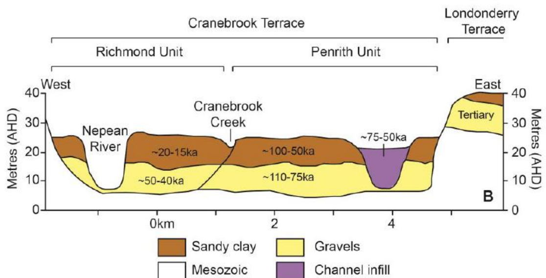
Figure 2.2 Cross-section of the Cranebrook Formation at Cranebrook, showing the spatial relationships between the Penrith and Richmond units. This figure does not include Holocene-aged deposits that can overlie these units. (Source: Williams et al. 2017, Figure 2B, 3 adapted from Stockton and Nanson 2004)
