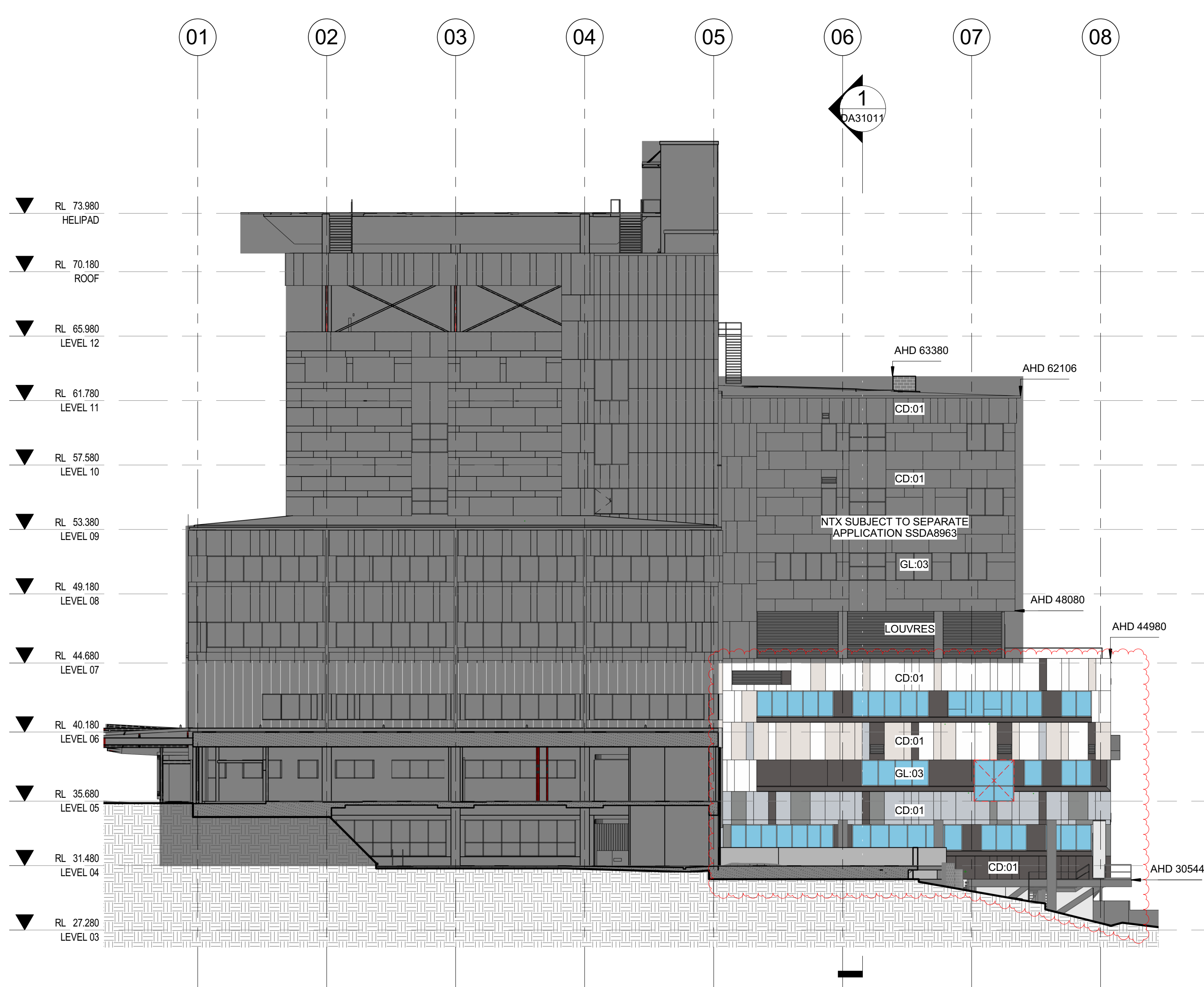
1 Building Elevation - East 3B2 1 : 200
