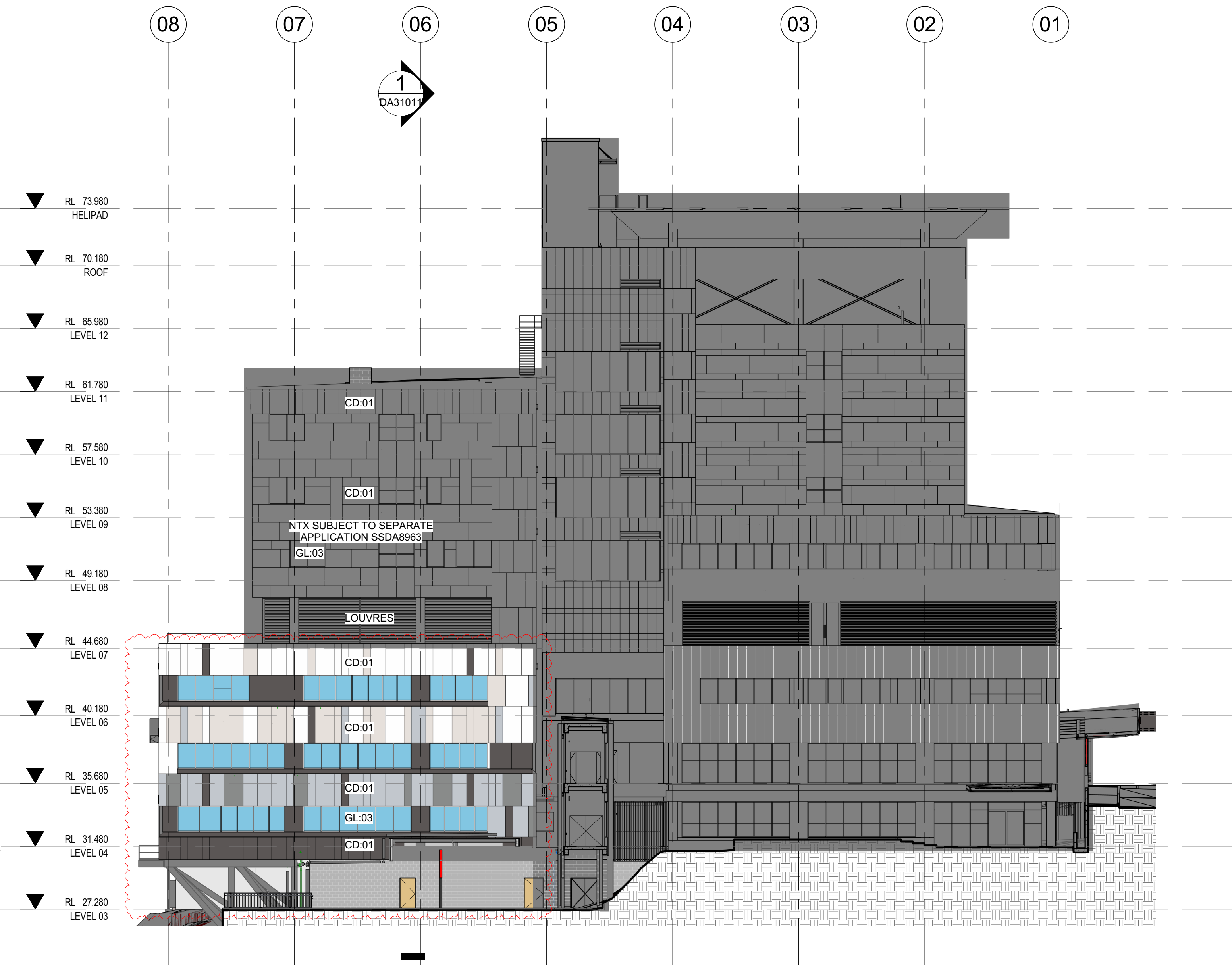
2 Building Elevation - West 3B2 1 : 200
