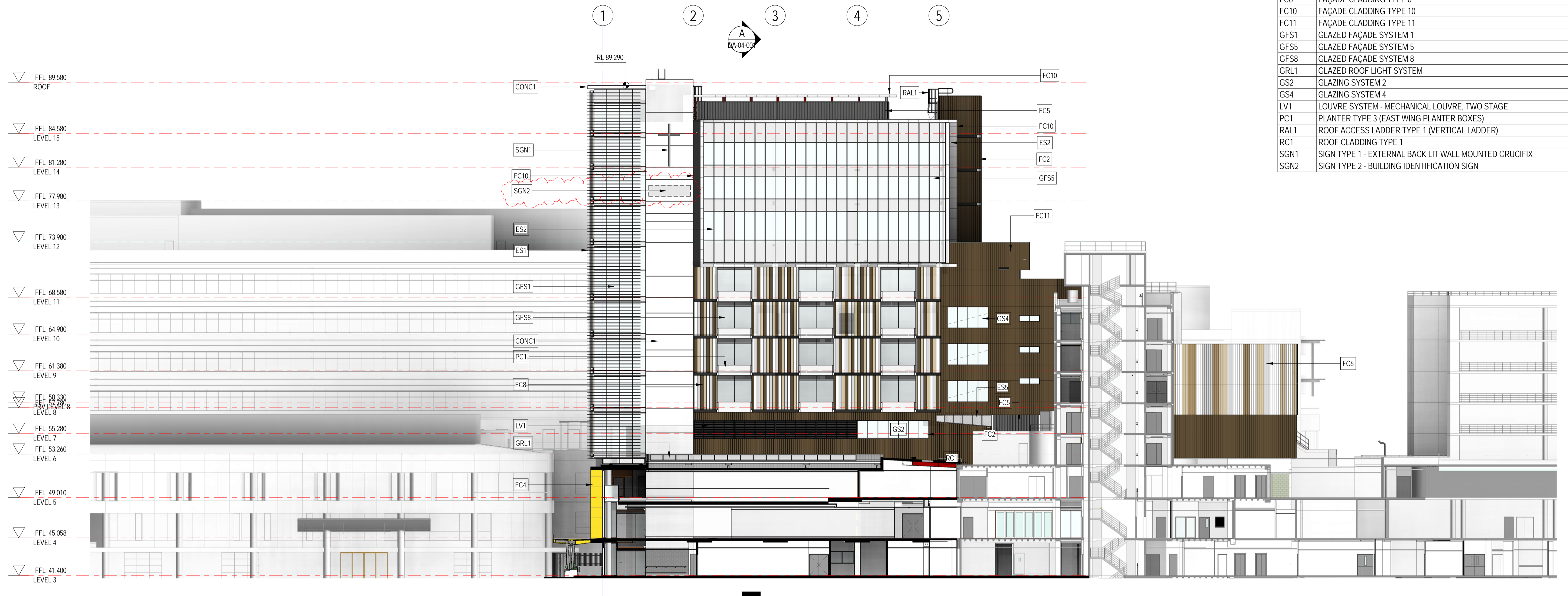
1 EAST WING - WEST ELEVATION 1:200
