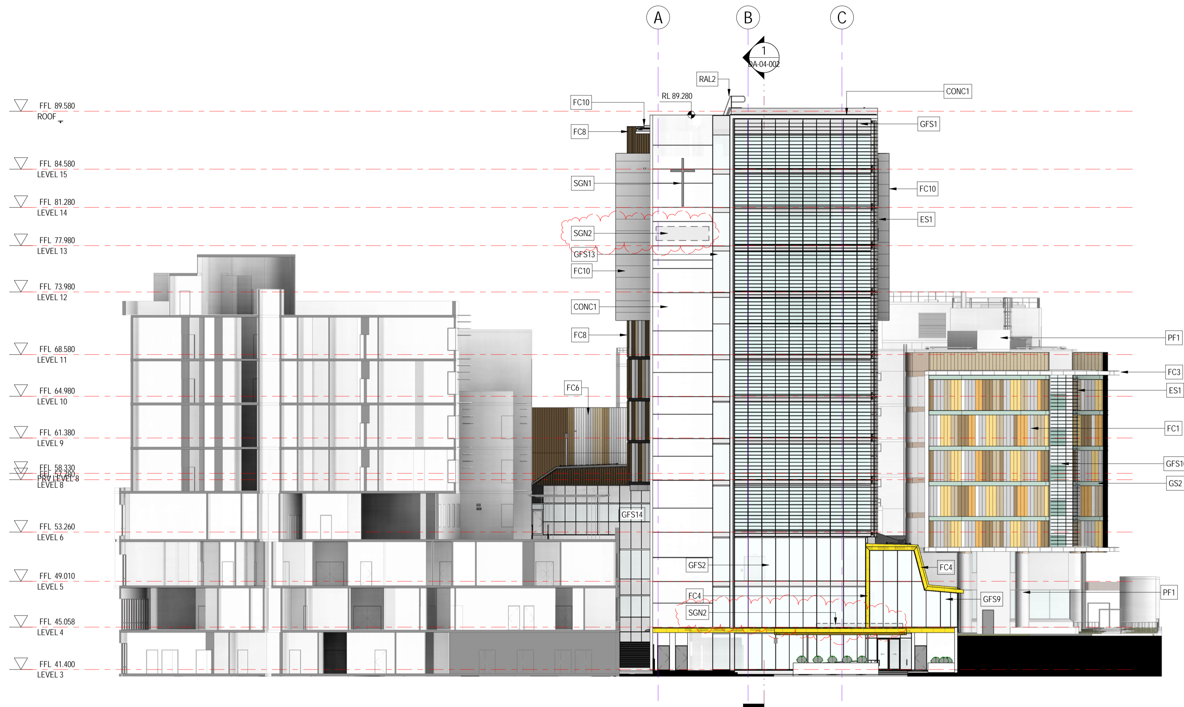
1 EAST WING - NORTH ELEVATION 1:200
