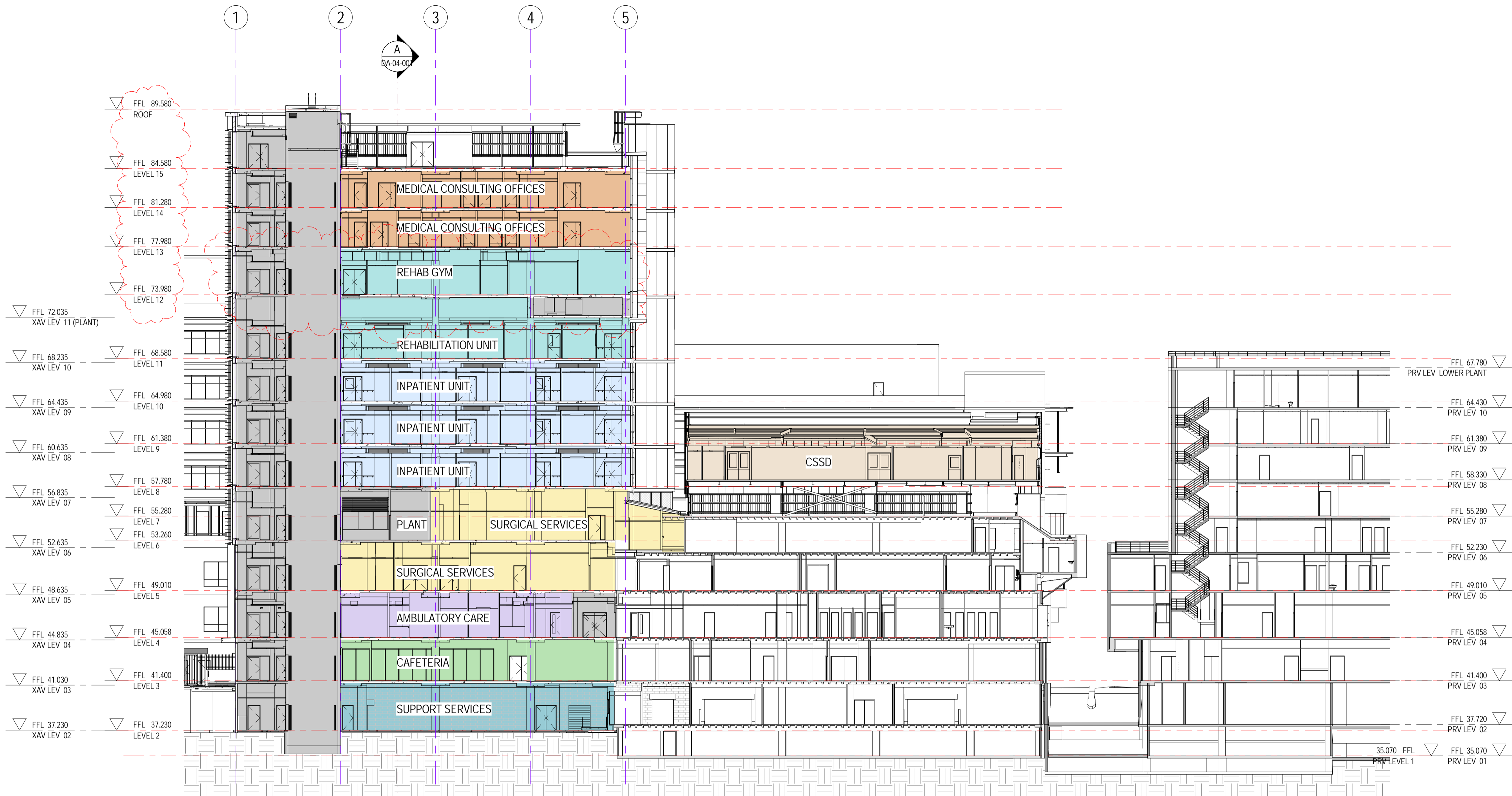
1 NORTH-SOUTH SECTION 1:200
