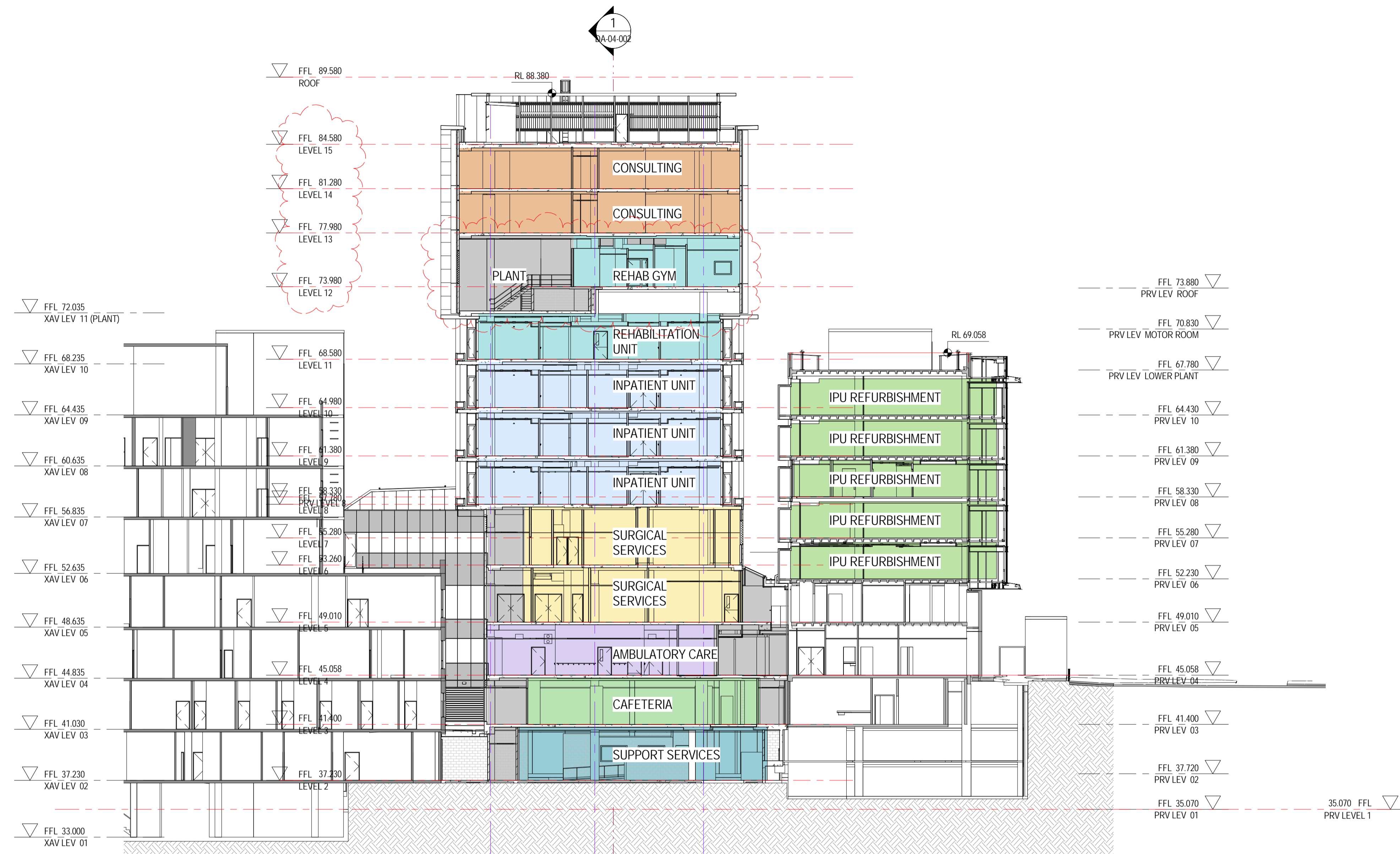
A EAST-WEST SECTION 1:200
