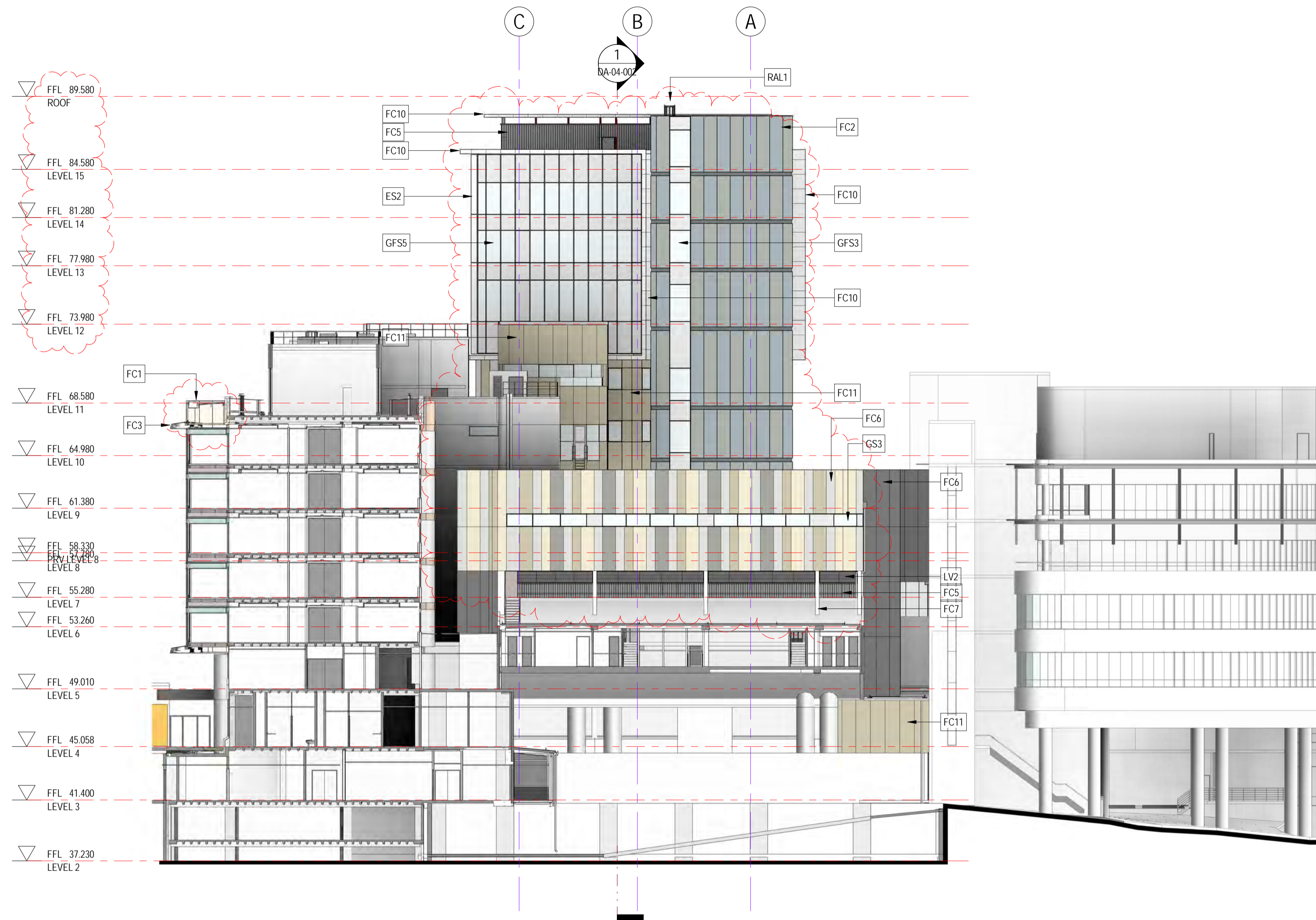
1 EAST WING - SOUTH ELEVATION 1:200
