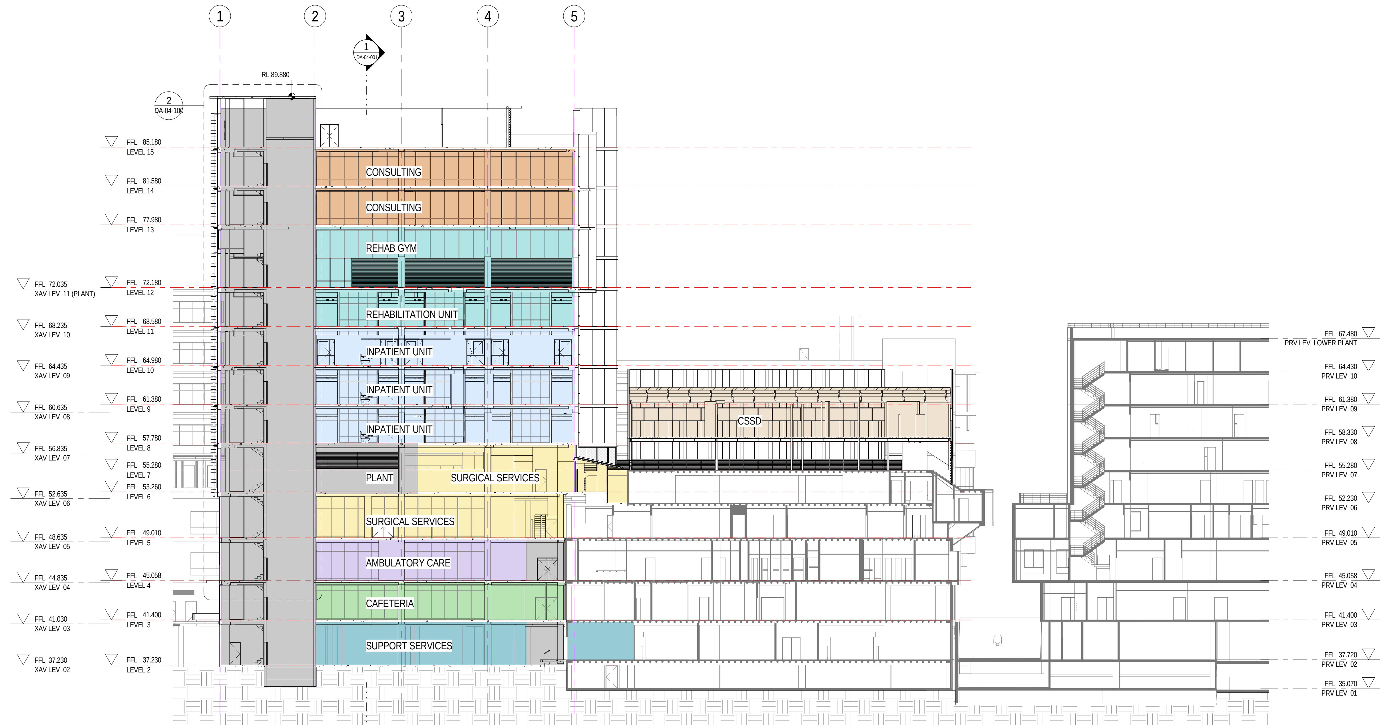
1 NORTH-SOUTH SECTION 1:200
