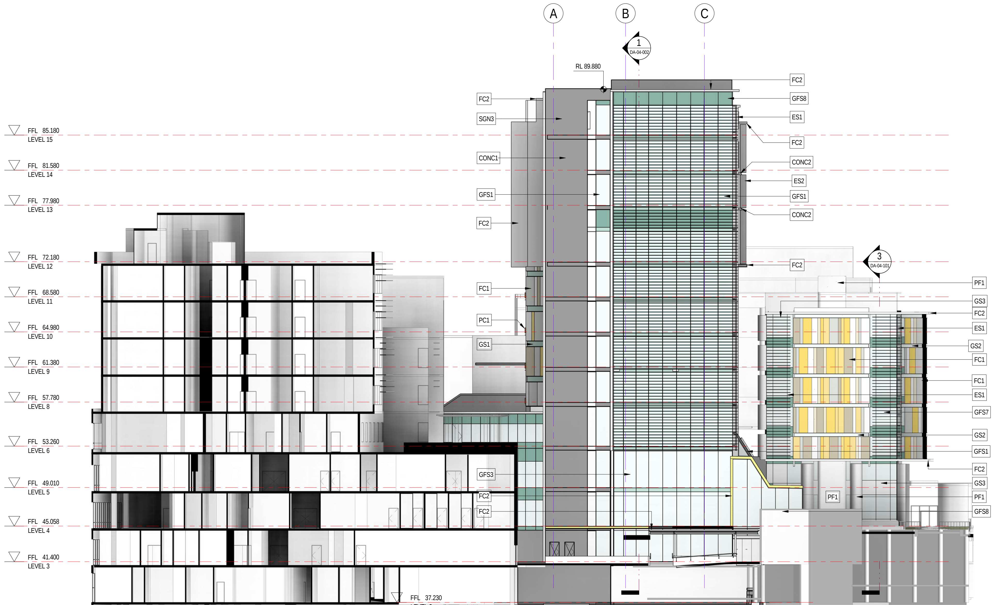
1 EAST WING - NORTH ELEVATION 1:200
