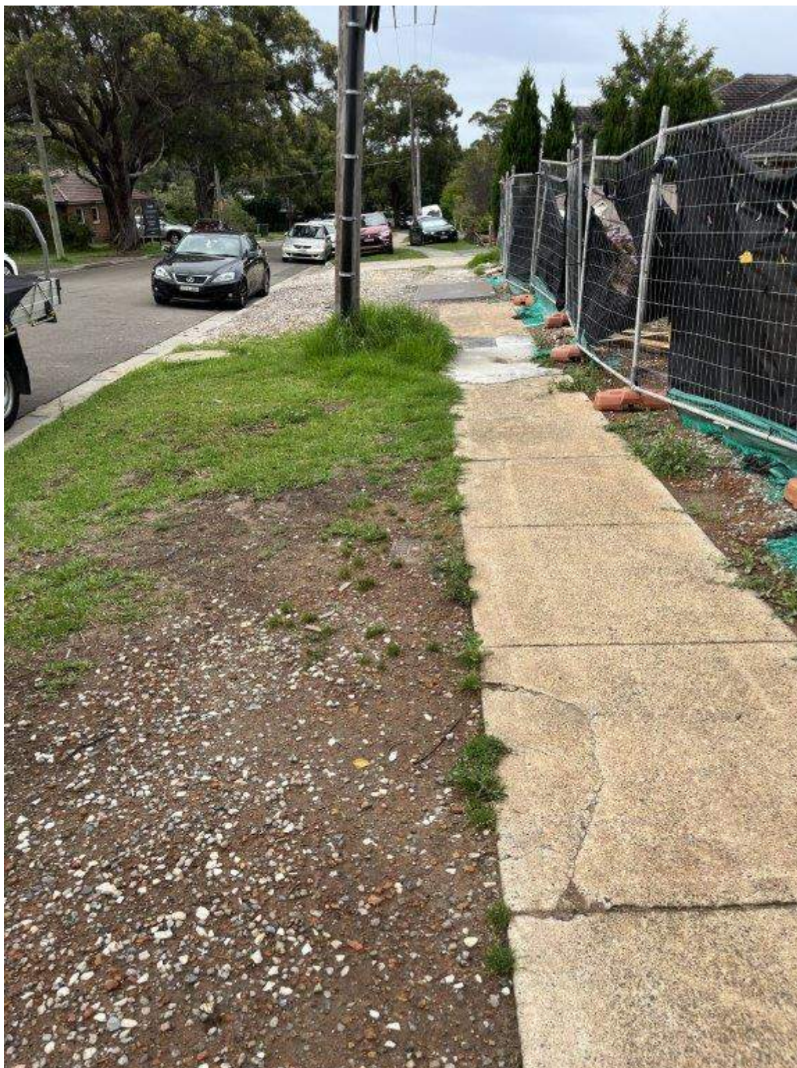
Photo 73 - Hinkler Avenue - Cracking and differential settlement of pavement
