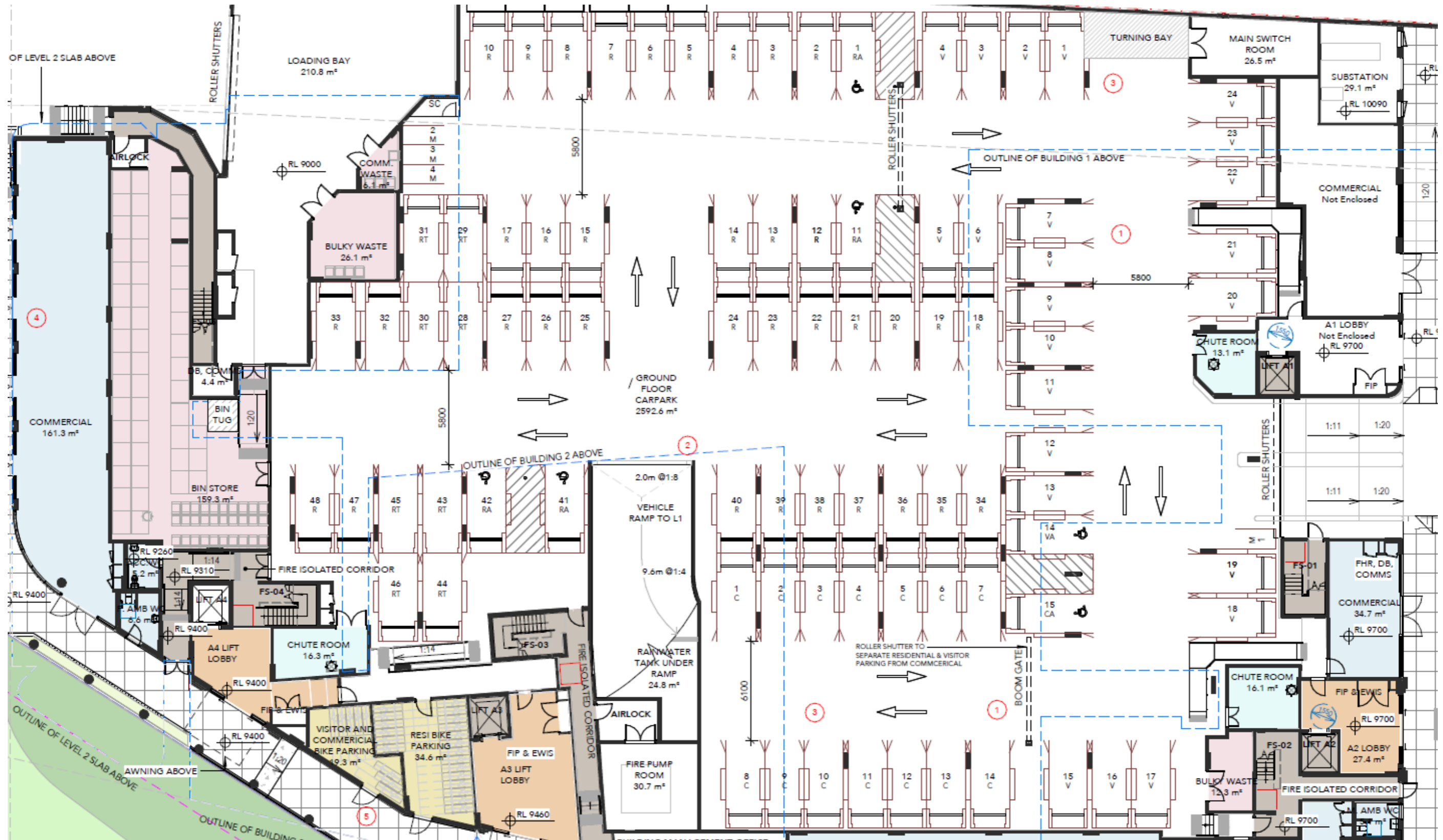
Source: Teams 2 Architects, DA-0300, Rev 5, Ground Level Floor Plan, 09.09.2025
