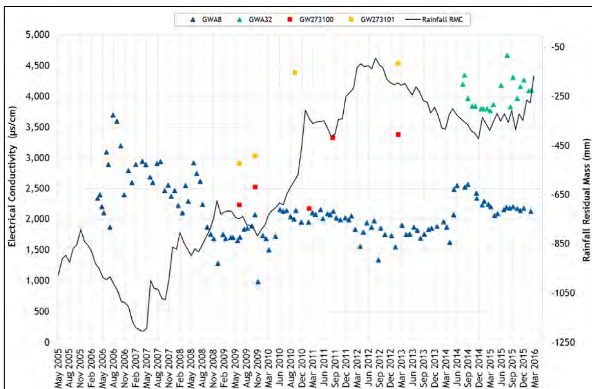
Figure 3 Electrical Conductivity in Alluvial Groundwater Monitoring Bores
