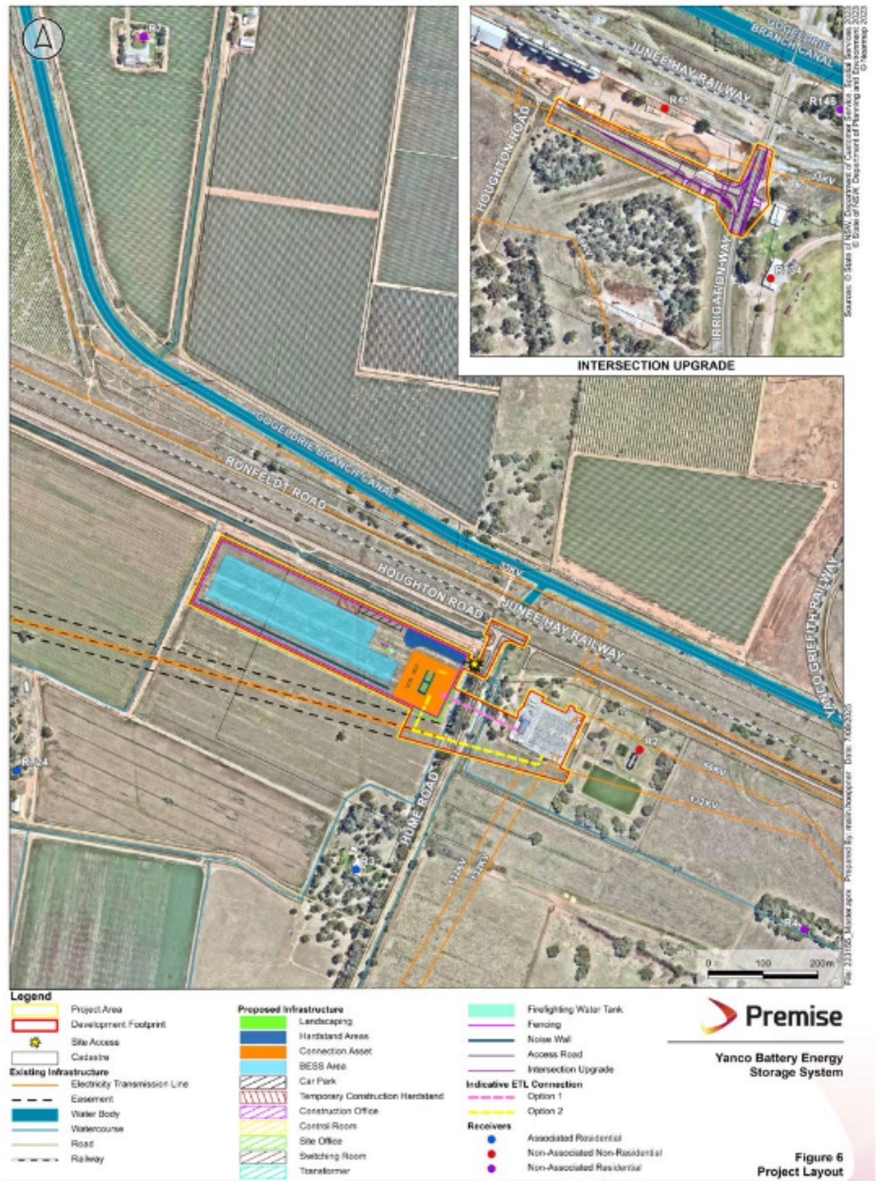
Figure 1: General Development Layout
