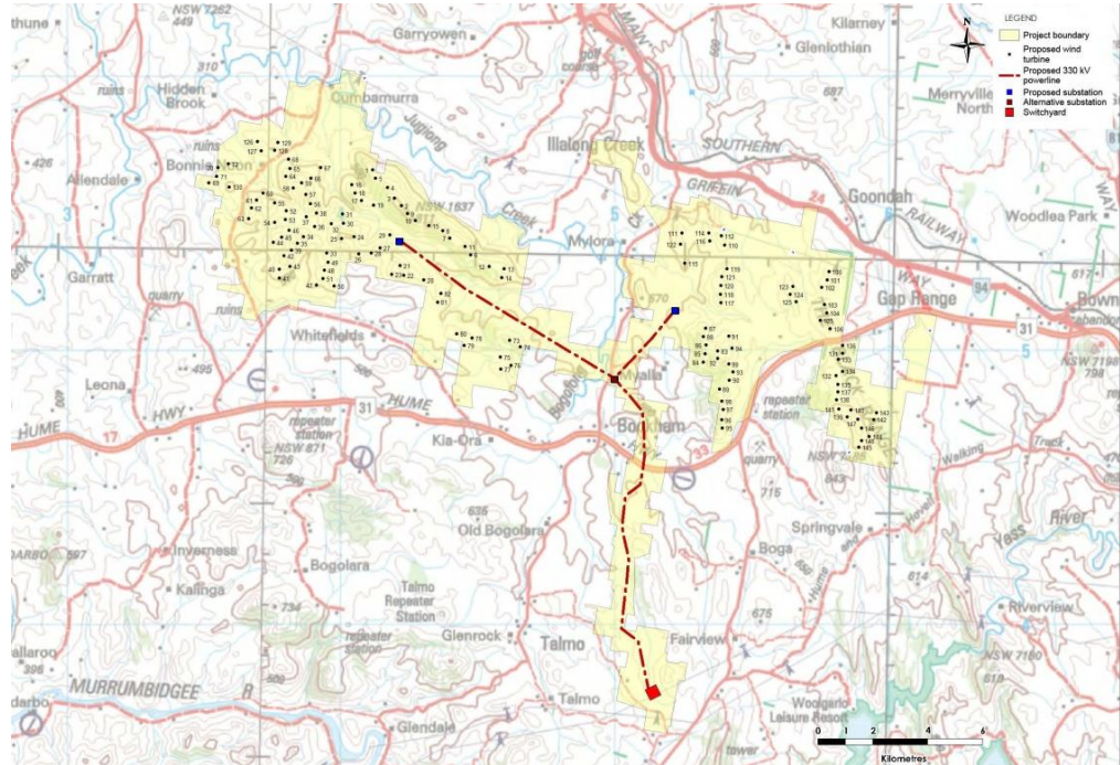
Figure 2-2 Site layout - EA Application
