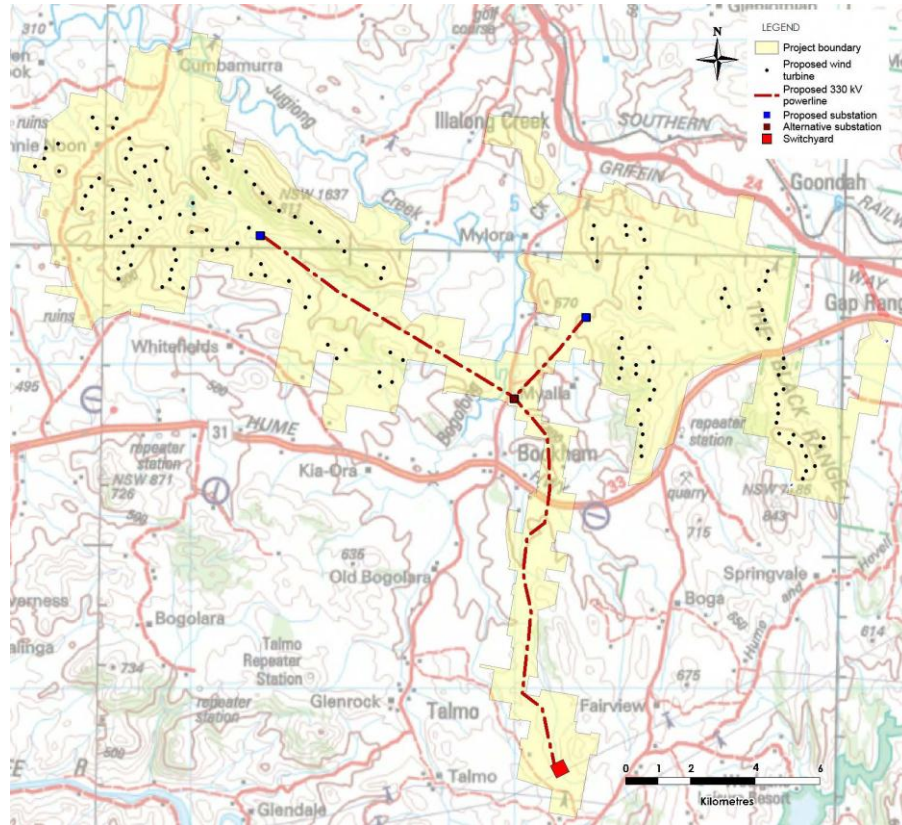
Figure 2-4 Site layout – Current Proposal
