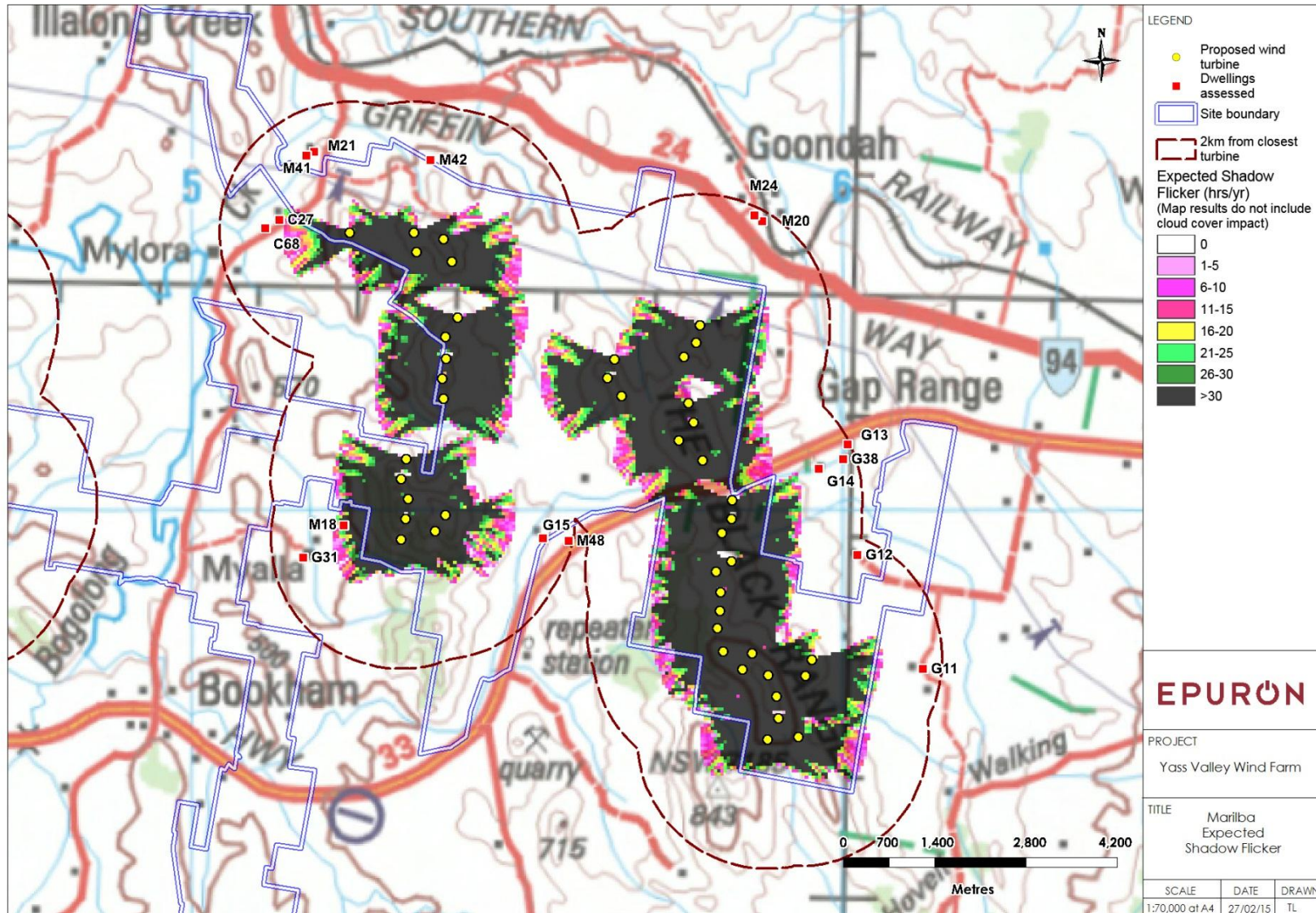
Figure 2 Results of shadow flicker assessment - Marilba
