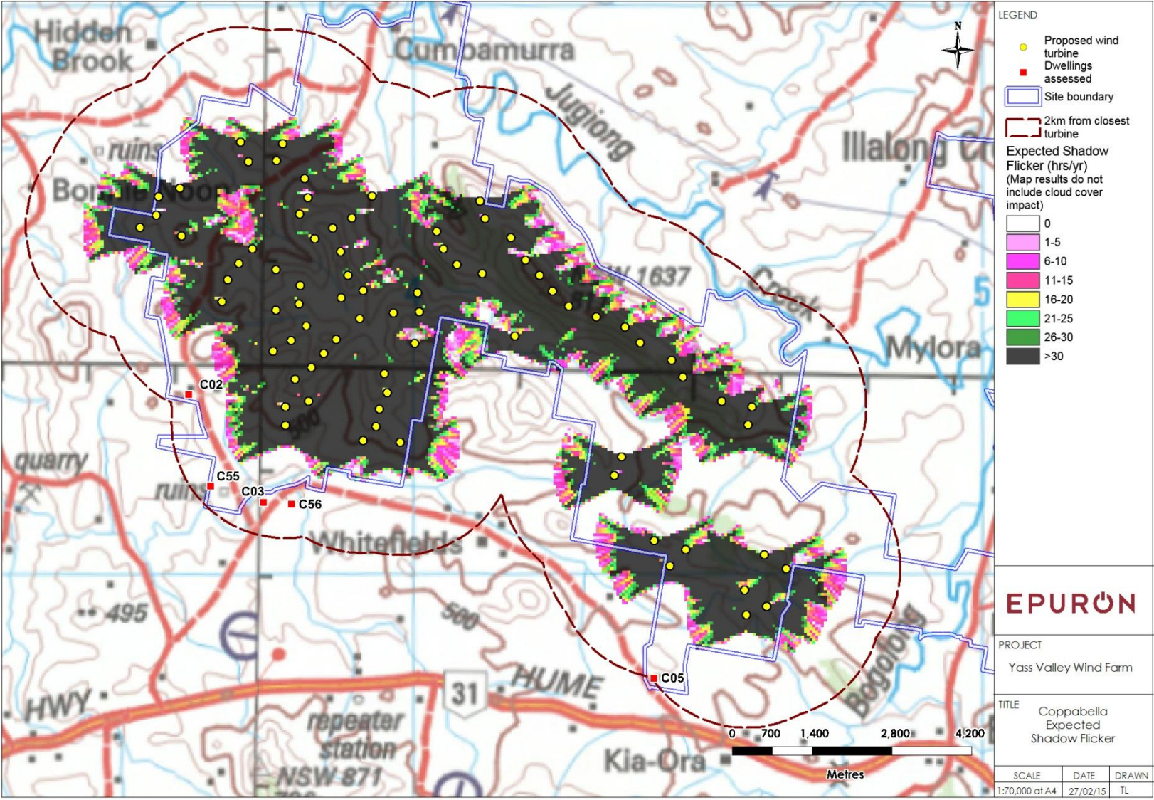
Figure 1 Results of shadow flicker assessment - Coppabella
