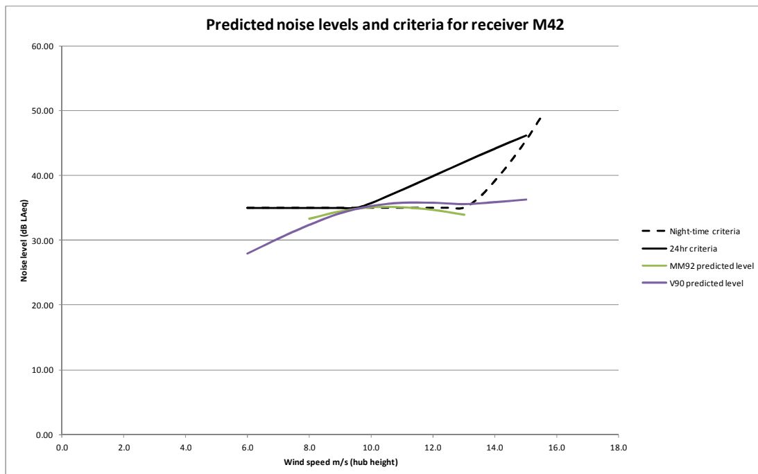
Figure K1: Predicted noise levels and criteria for receiver M42
