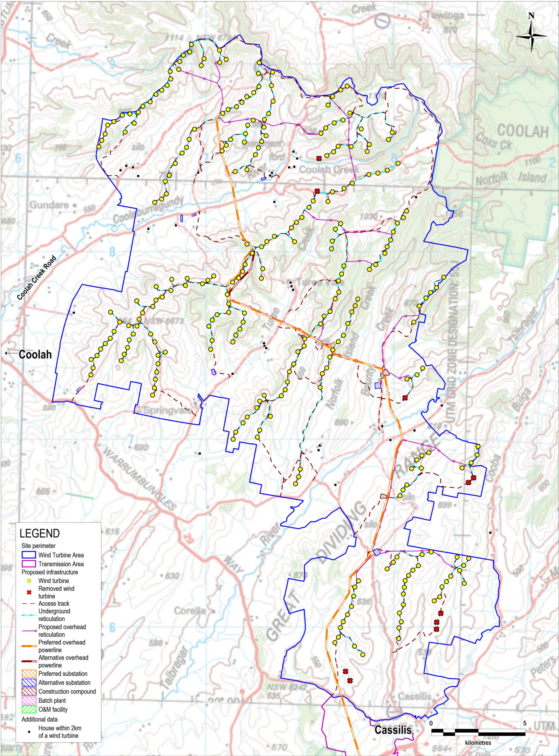
Figure 1: Proposed turbine and infrastructure layout
