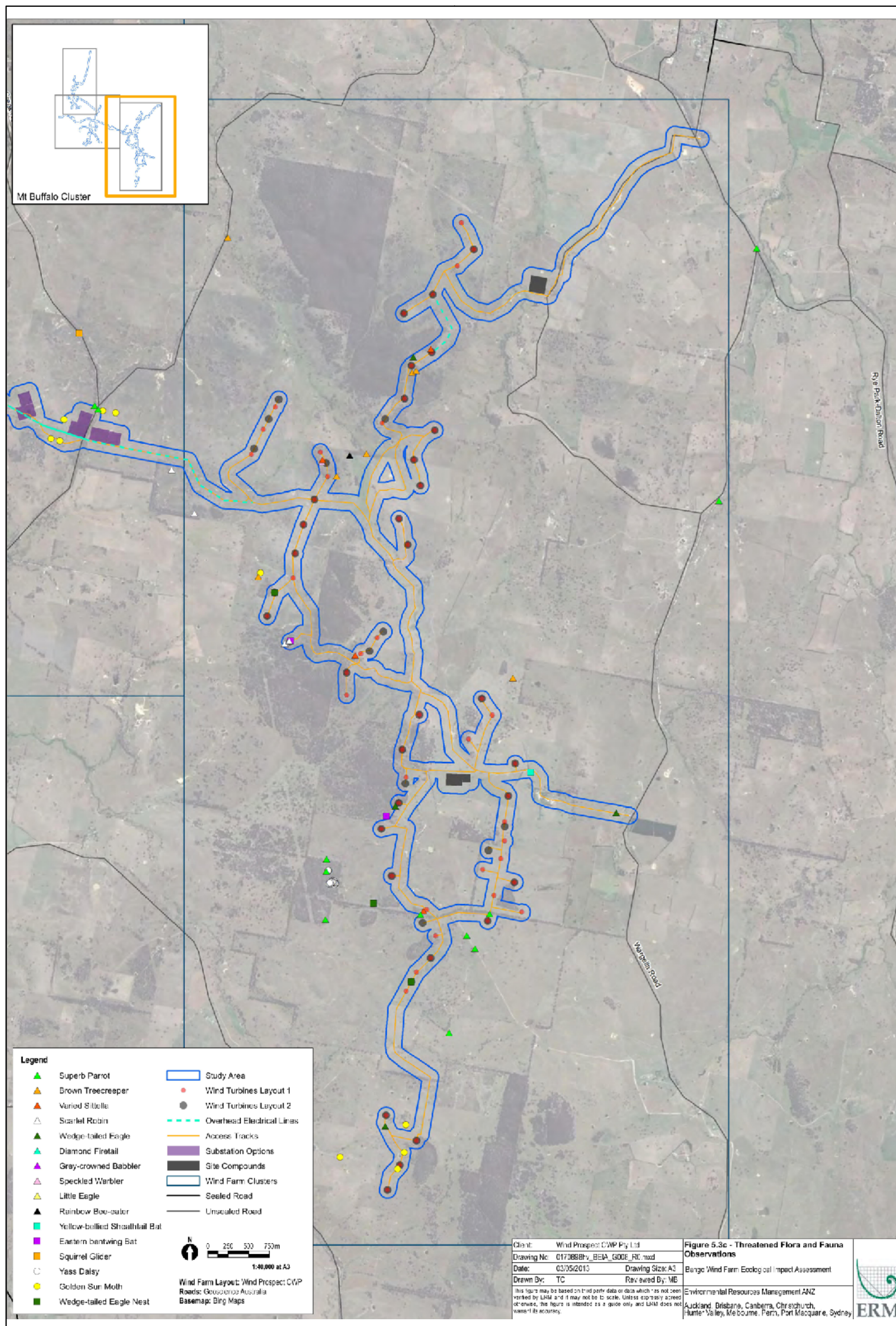
FIGURE 10.13: THREATENED SPECIES RECORDED ACROSS THE STUDY AREA - MT BUFFALO CLUSTER
