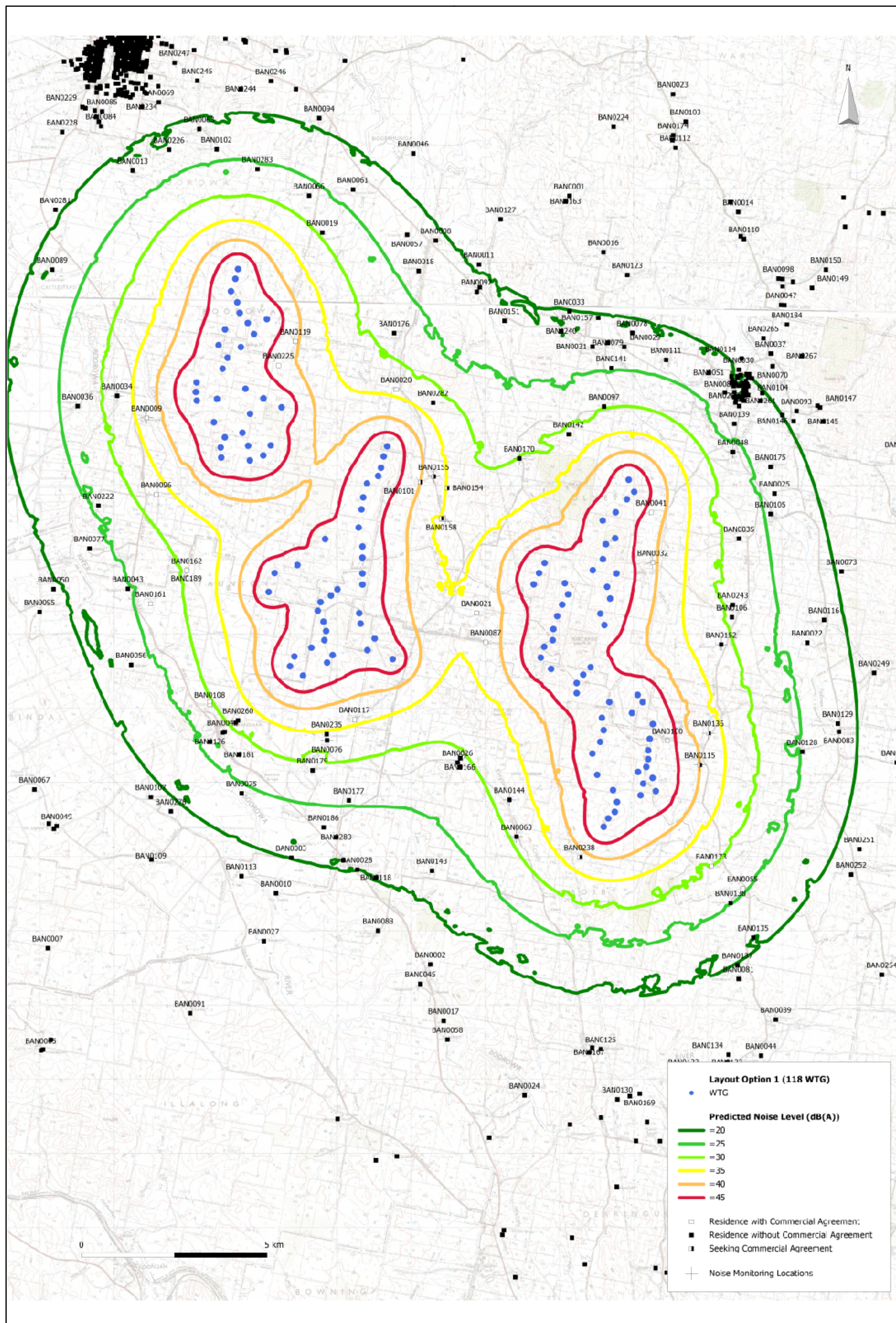
FIGURE 9.1: LAYOUT OPTION 1, NOISE CONTOUR MAP
