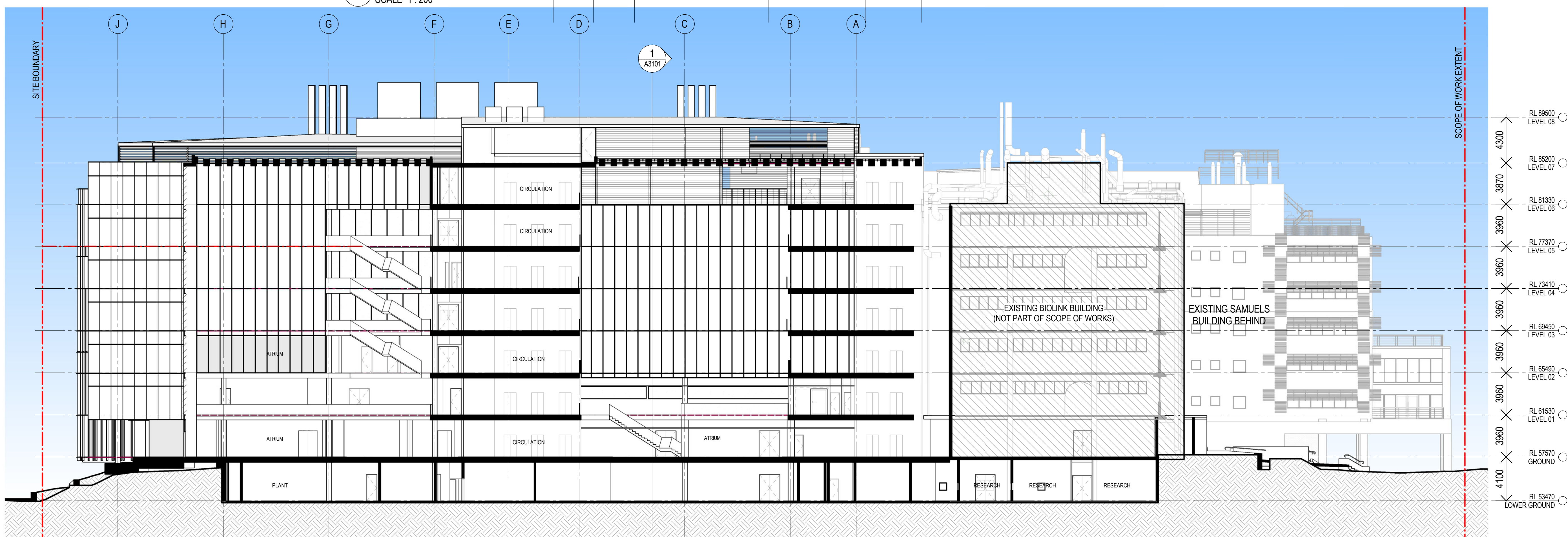
2 SECTION D SCALE 1:200
