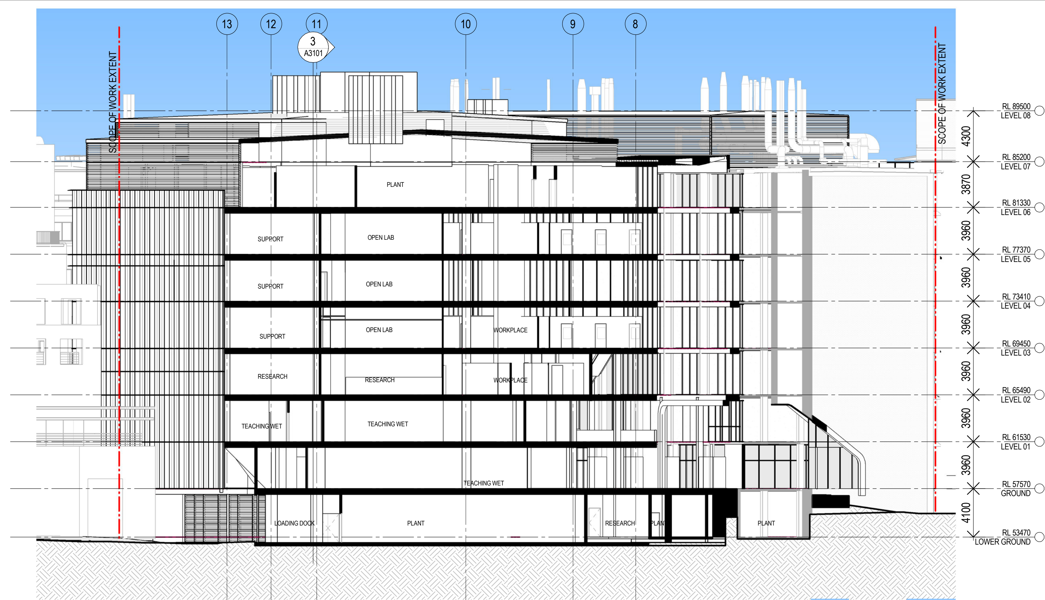
1 SECTION C SCALE 1:200
