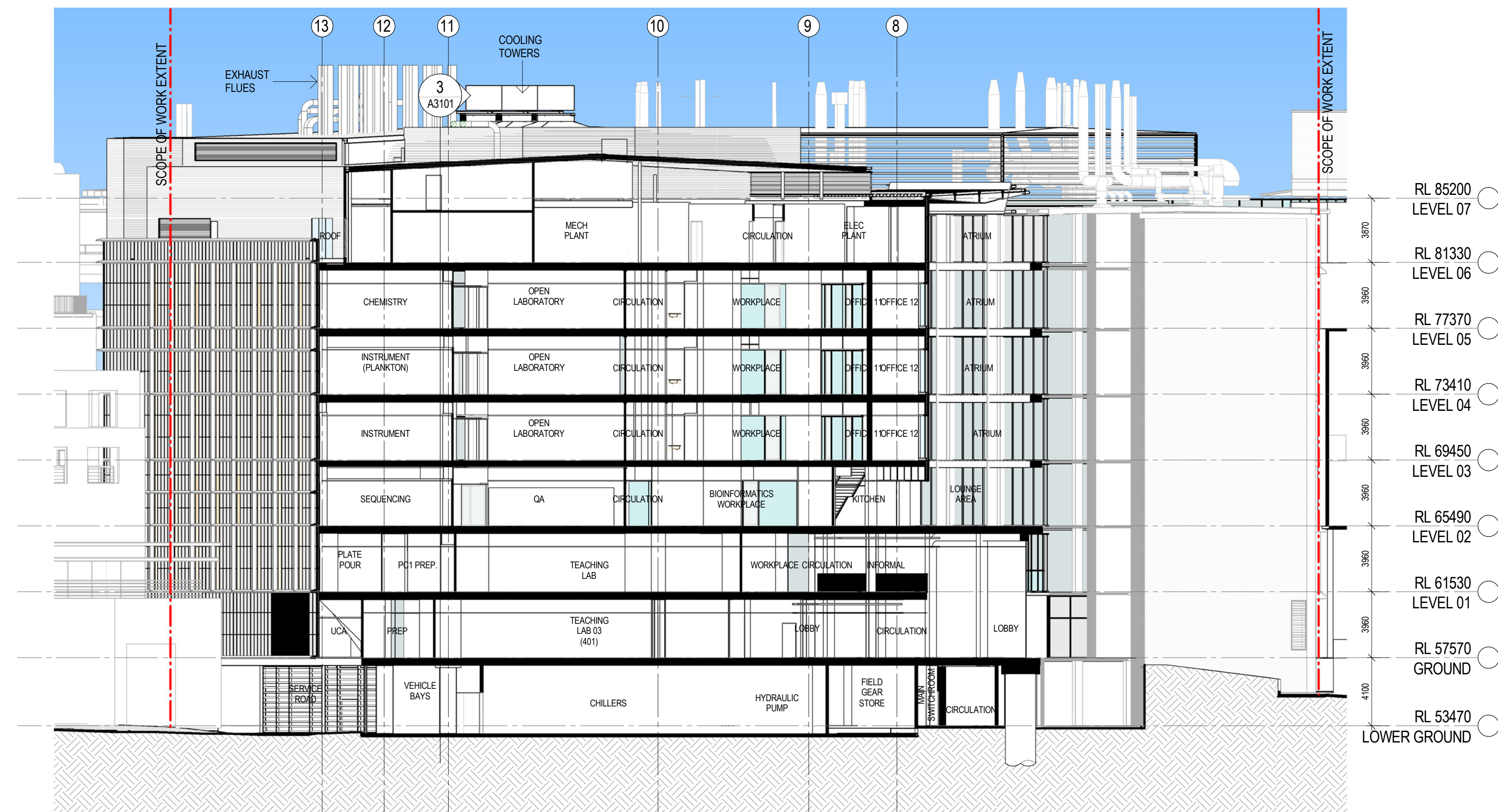
1 SECTION C (SSD) SCALE 1:200
