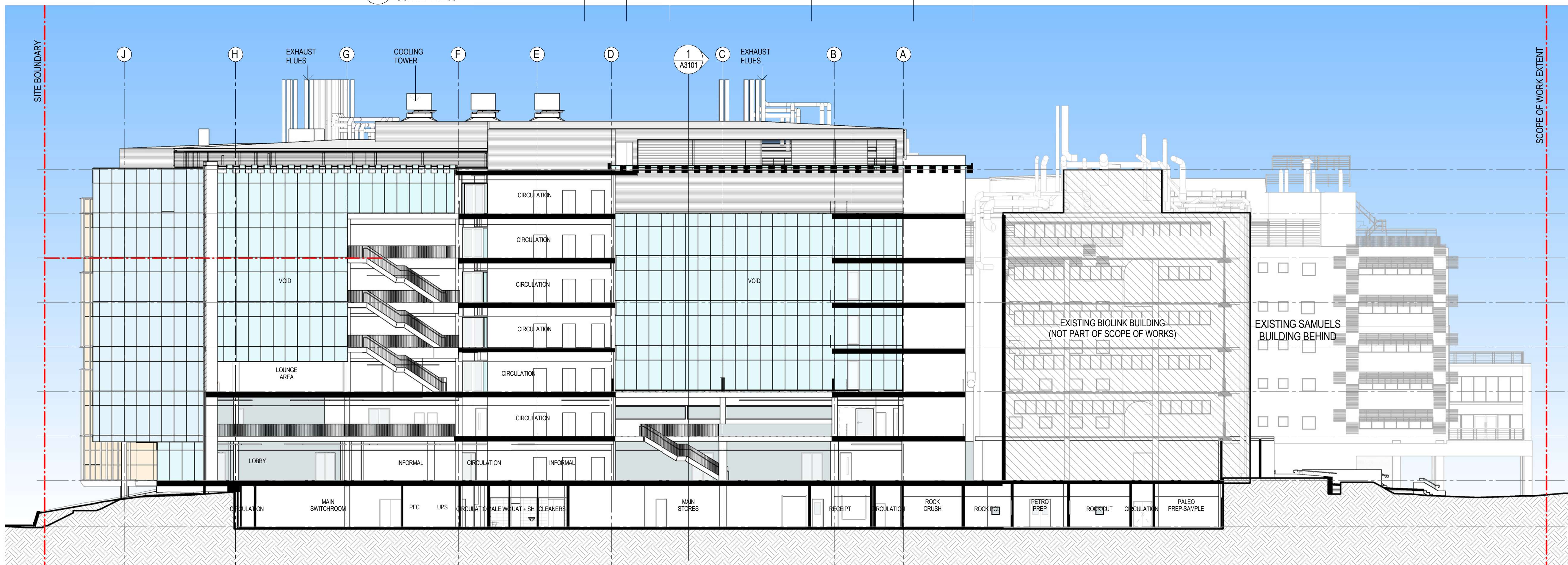
2 SECTION D (SSD) SCALE 1:200
