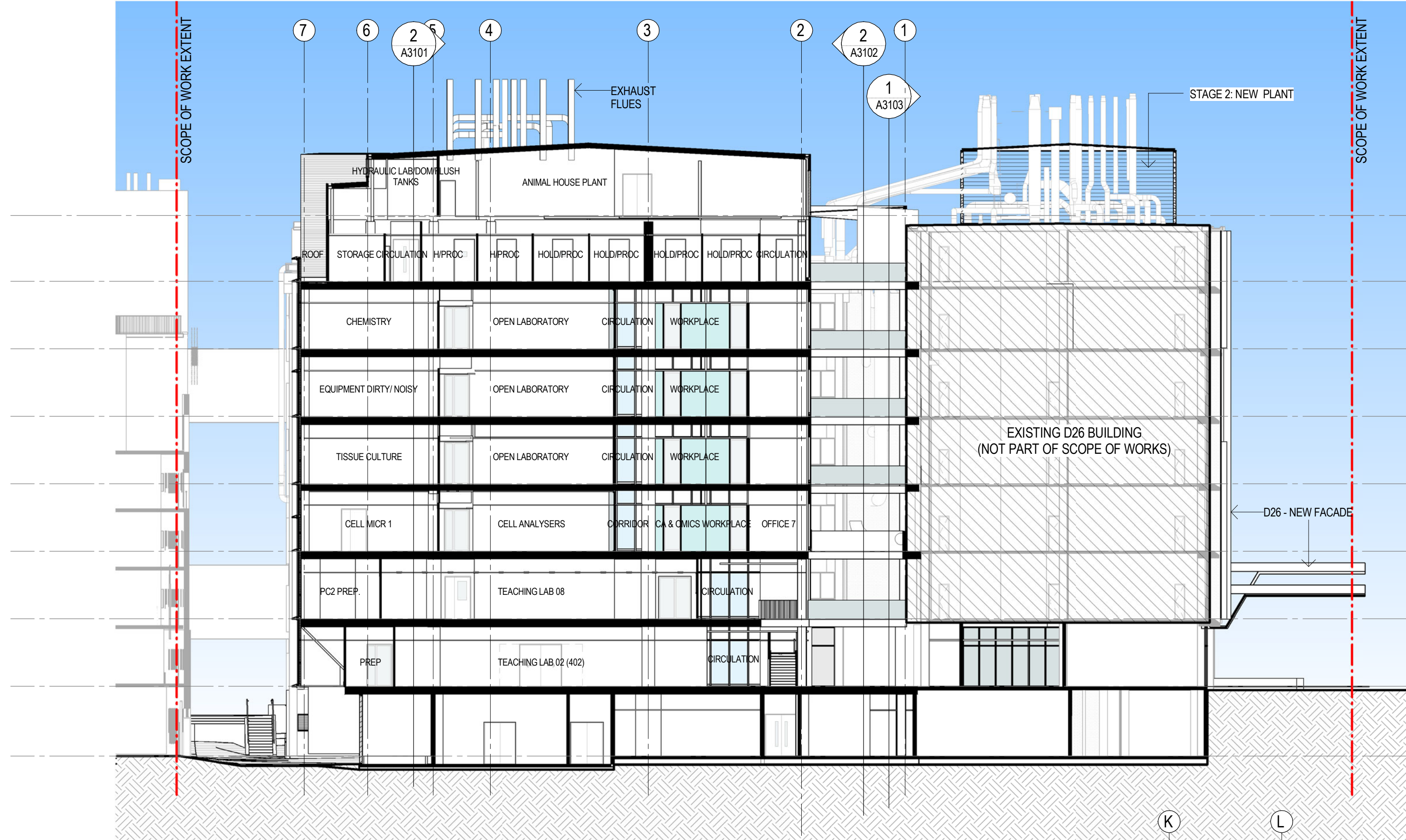
1 SECTION A (SSD) SCALE 1 : 200
