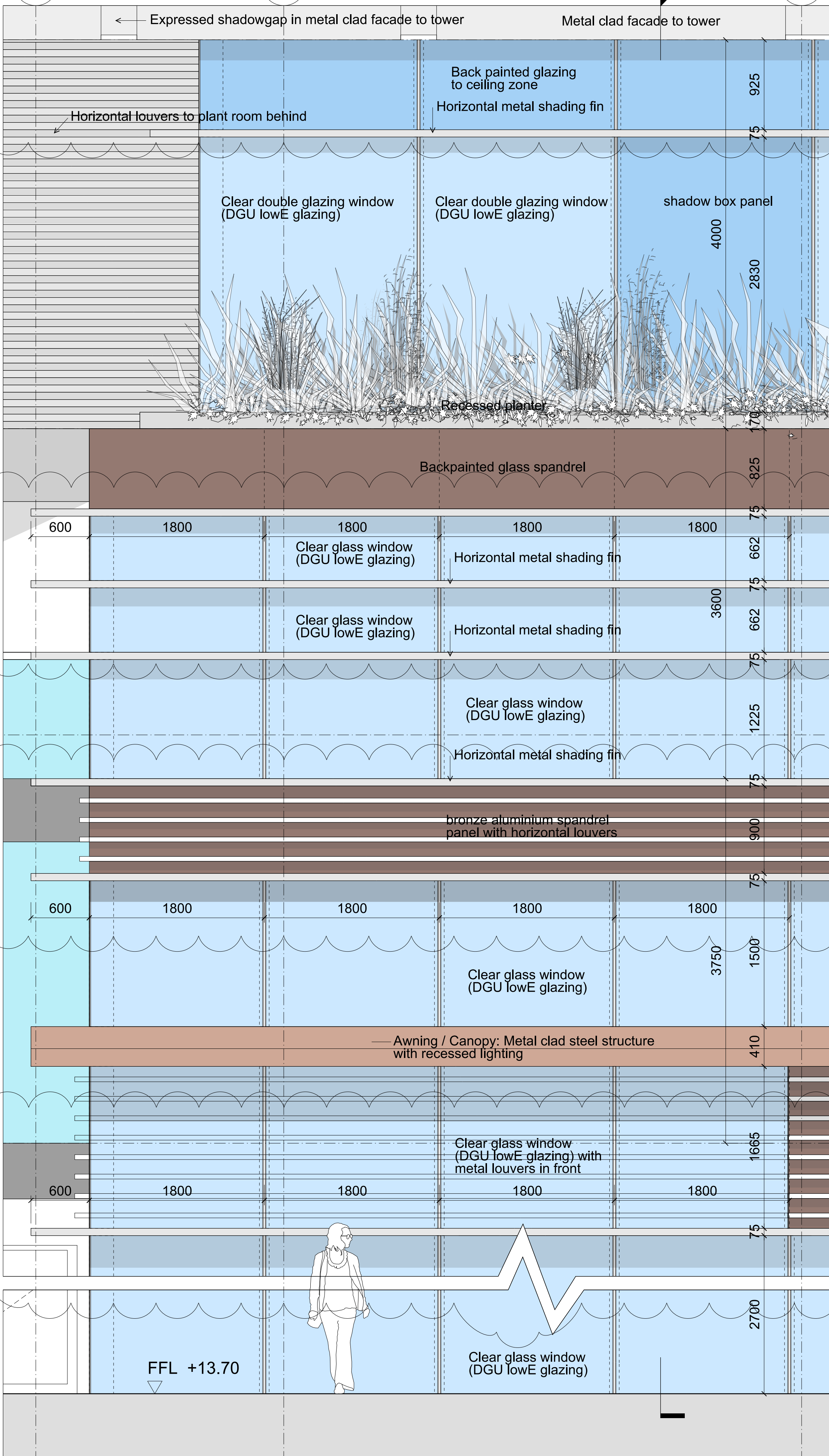
02 Typical Podium Facade - Elevation
