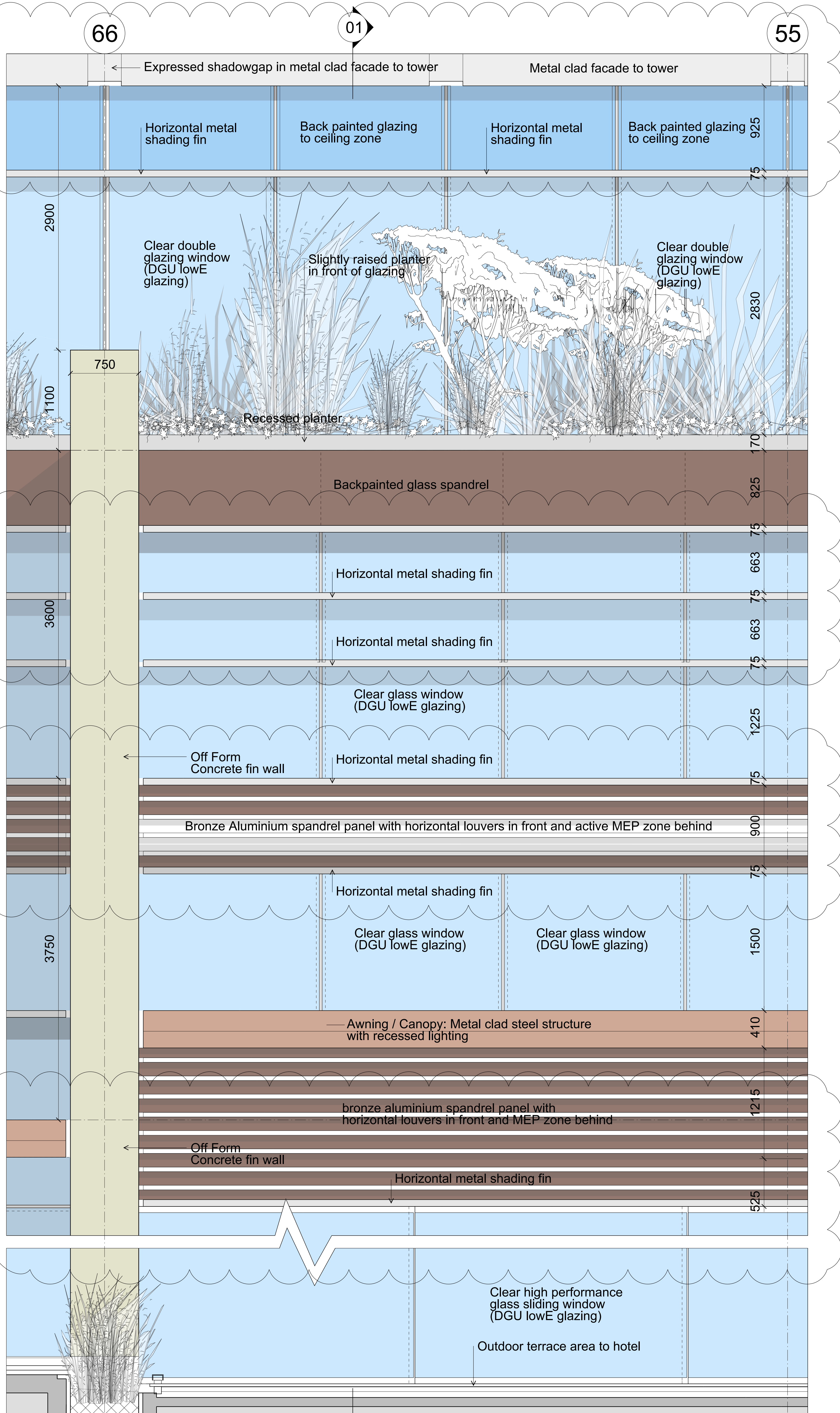
02 Typical Podium Facade - Elevation
