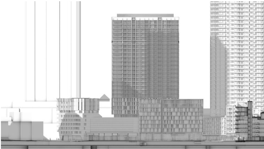
NORTH ELEVATION - 10am
