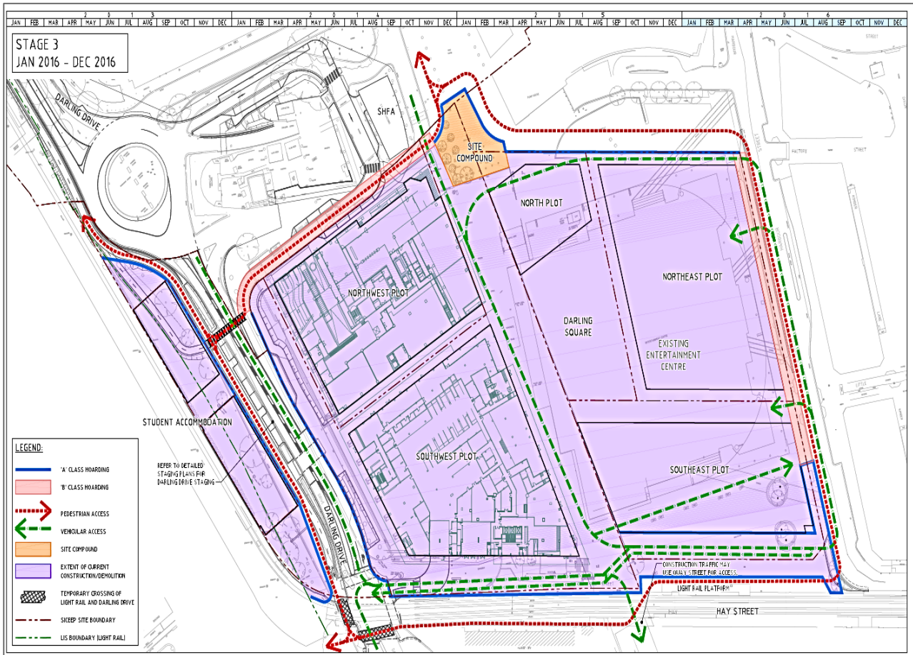
Figure 8a – Pedestrian access outlined in red and Trafficable access in green
