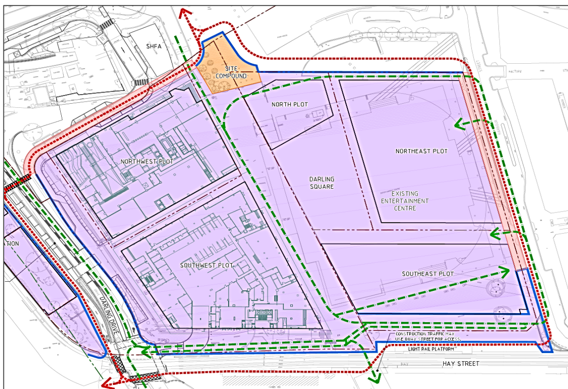
Figure 5 – A Class hoarding is outlined in blue and B Class hoarding is shaded in red
