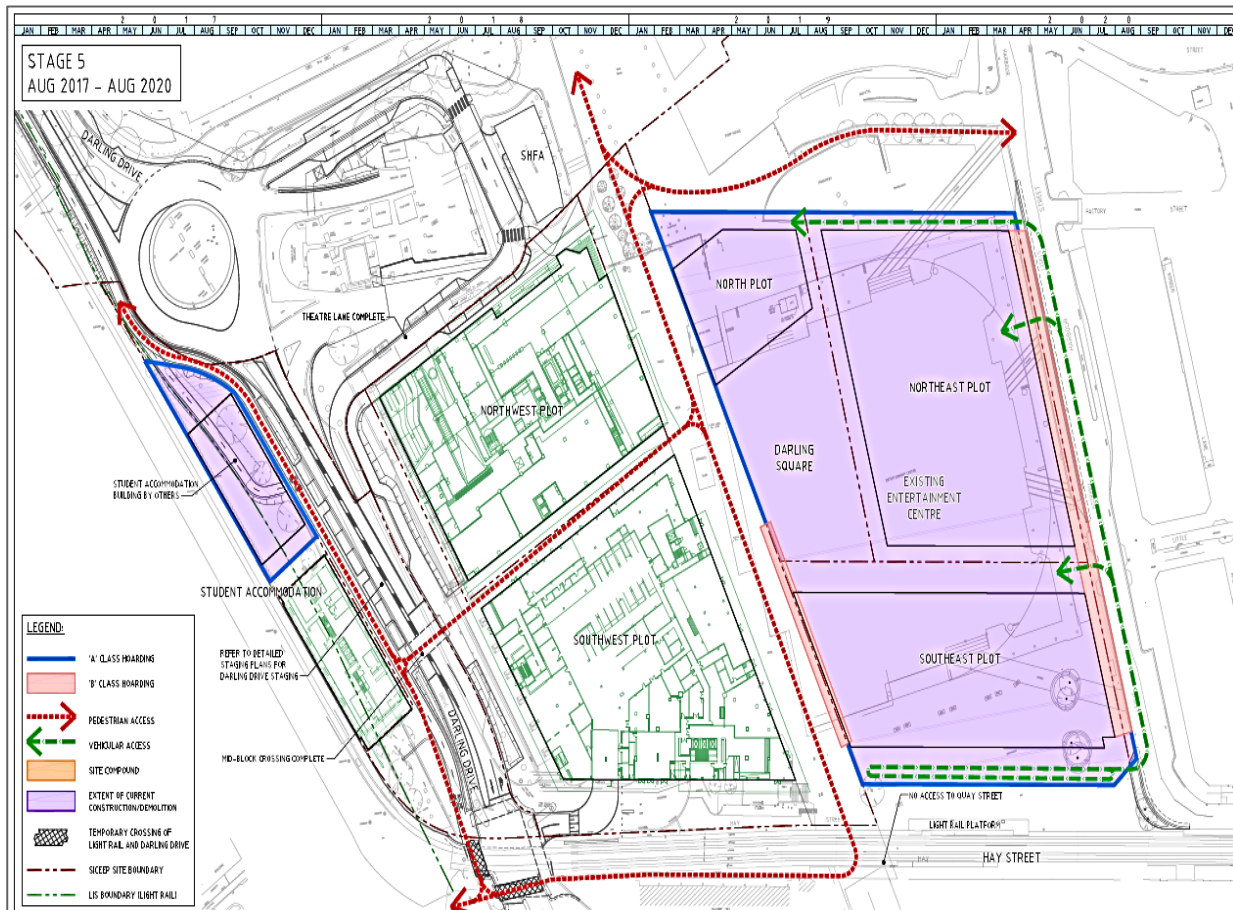
Figure 8c – Pedestrian access outlined in red and Trafficable access in green
