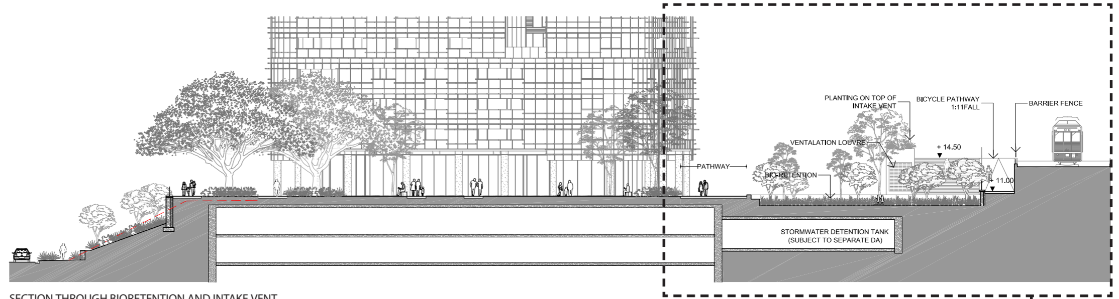
SECTION THROUGH BIORETENTION AND INTAKE VENT SCALE 1:400 @ A3
