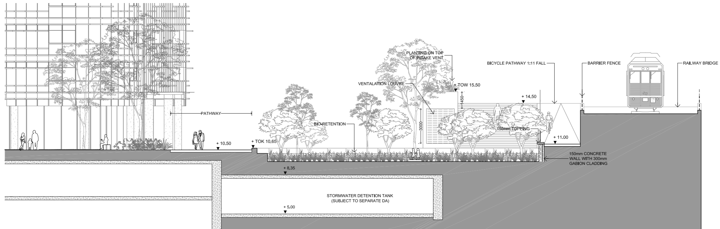
SECTION THROUGH BIORETENTION AND INTAKE VENT SCALE 1:200 @ A3
