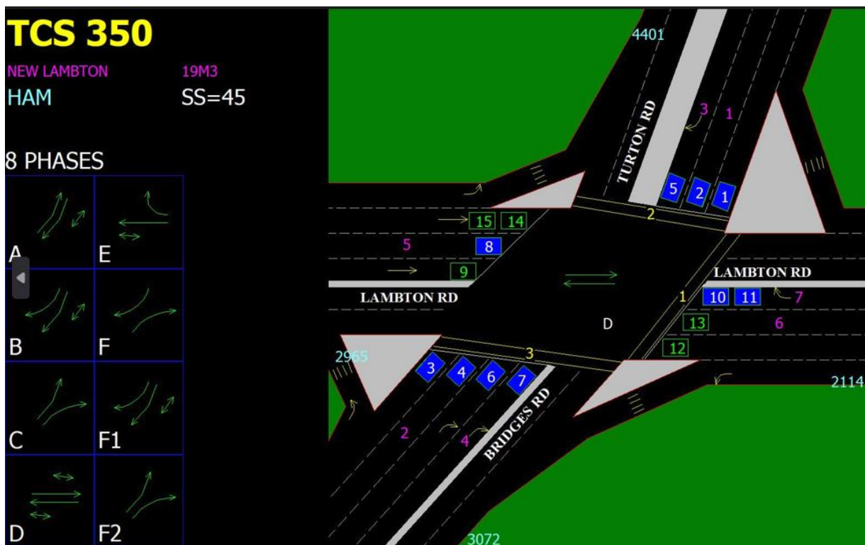
Figure 3.5: Turton Road / Lambton Road / Bridges Road - TCS 350 Signal Phasing
