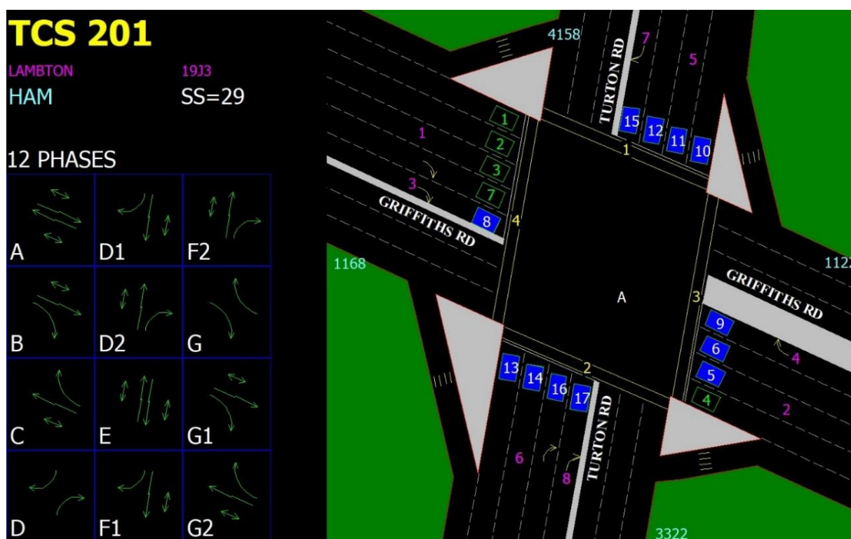
Figure 3.3: Turton Road / Griffiths Road - TCS 201 Signal Phasing
