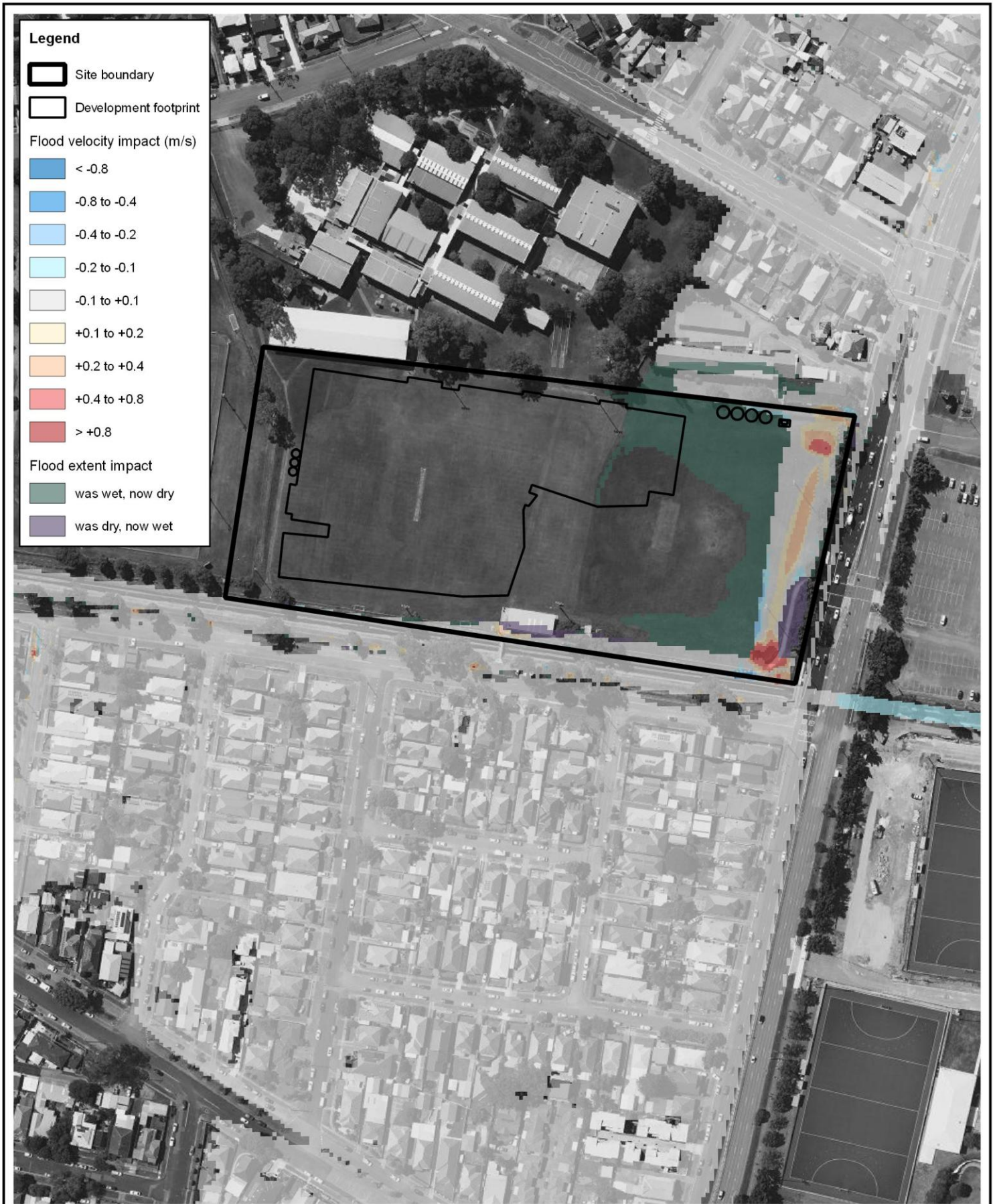
Title: Modelled 2% AEP Peak Flood Velocity Impact
