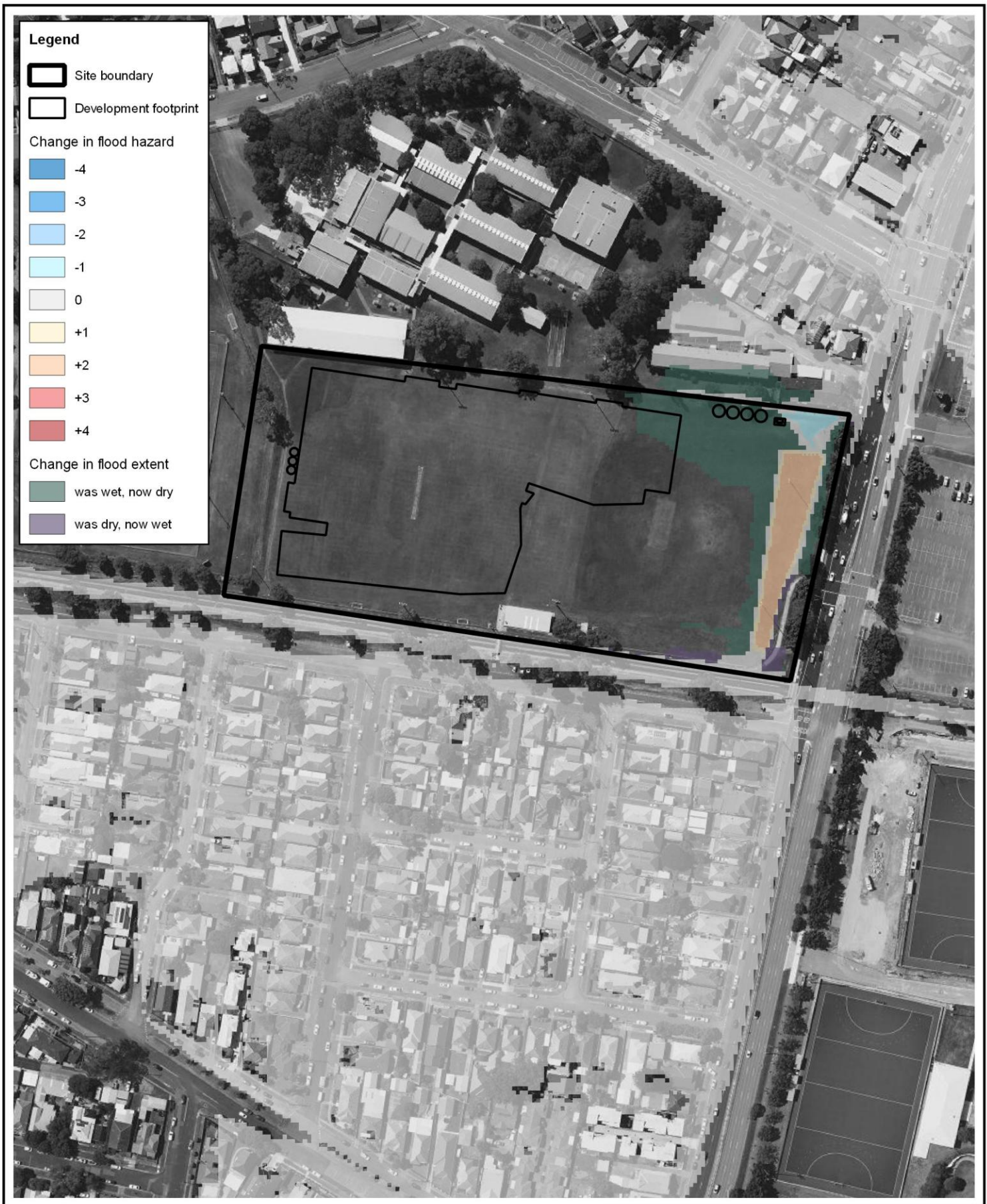
Title: Modelled Change in 5% AEP Flood Hazard Classification
