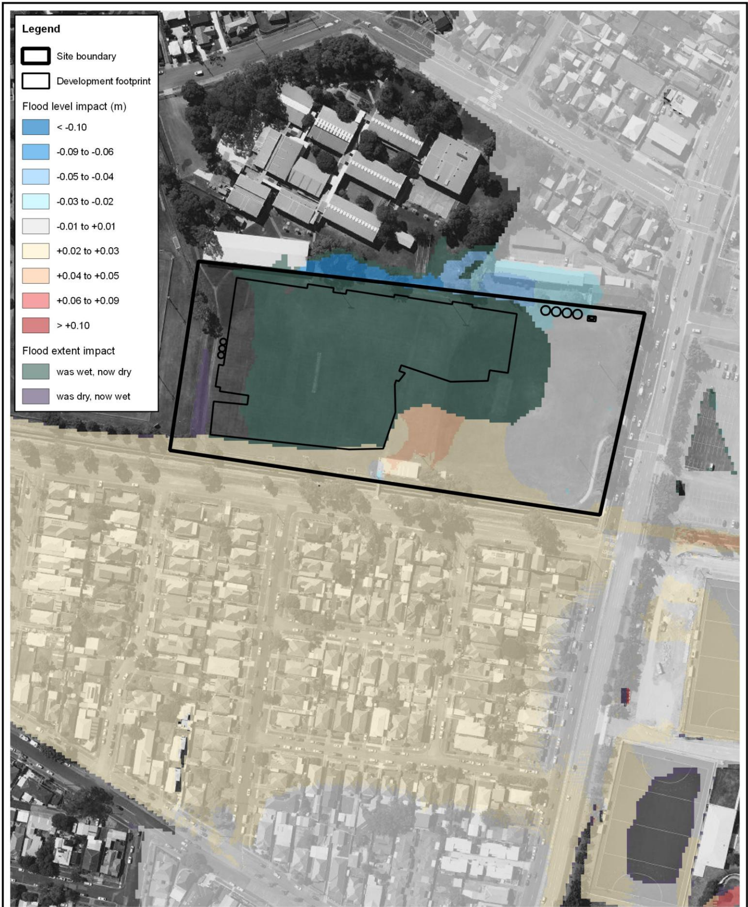
Title: Modelled 0.2% AEP Peak Flood Level Impact
