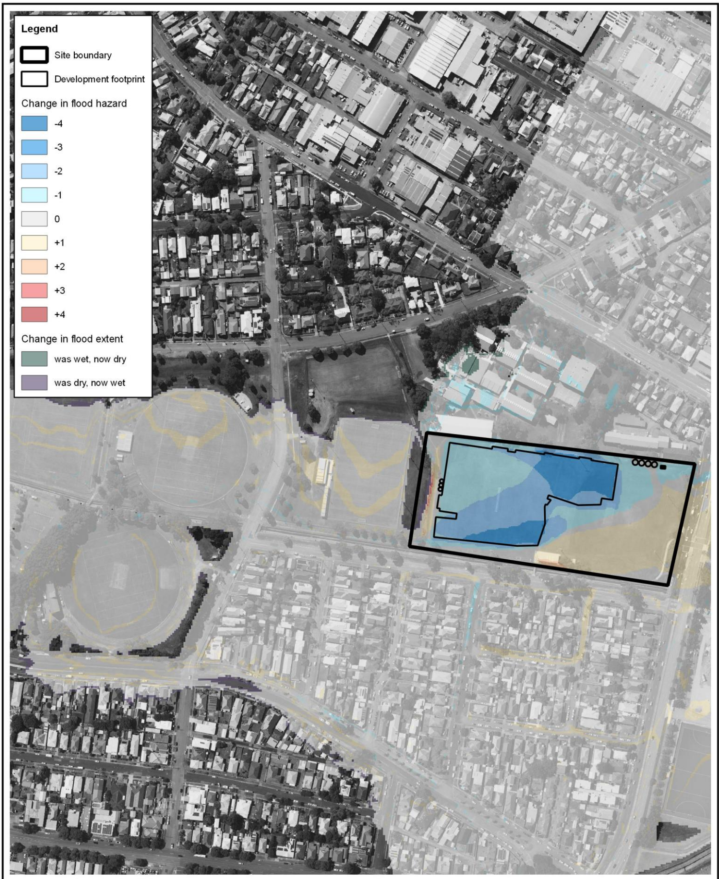
Title: Modelled Change in PMF Flood Hazard Classification
