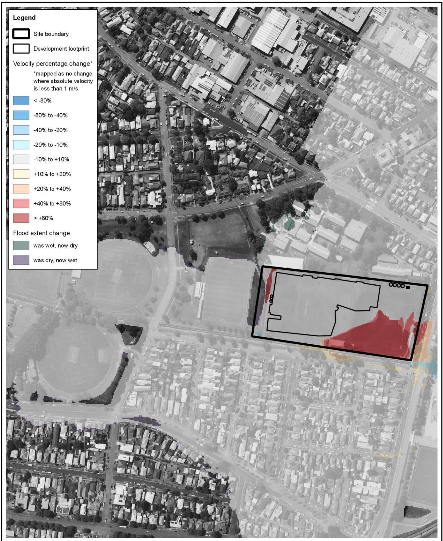
Title: Modelled PMF Percentage Change in Peak Flood Velocity
