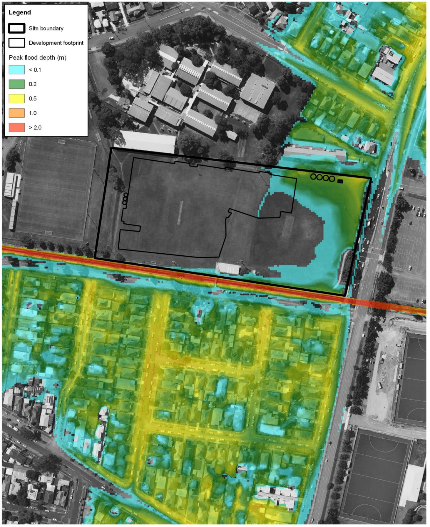
Title: Modelled 2% AEP Peak Flood Depth
