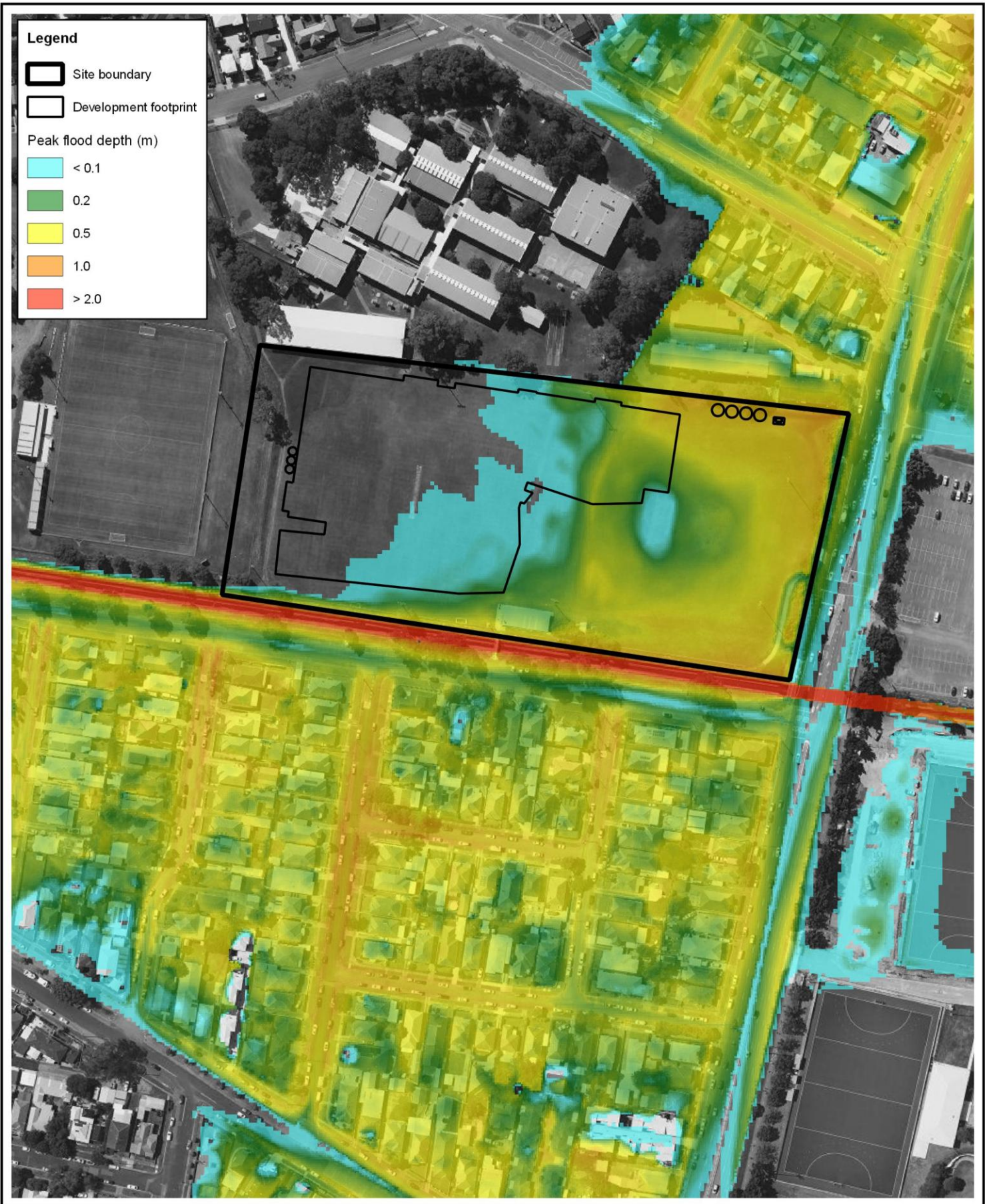
Title: Modelled 0.5% AEP Peak Flood Depth
