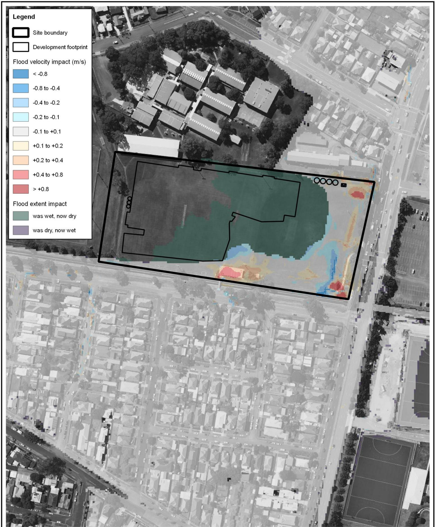
Title: Modelled 1% AEP (2050) Peak Flood Velocity Impact
