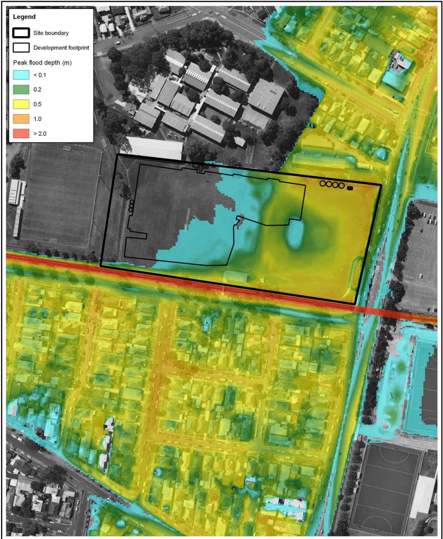
Title: Modelled 1% AEP (2050) Peak Flood Depth
