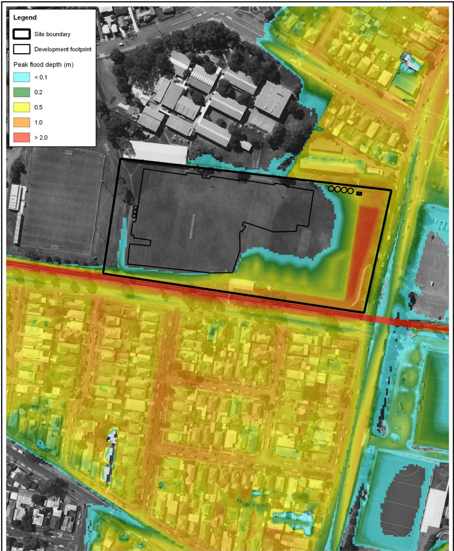
Title: Modelled 0.2% AEP Peak Flood Depth for Post-development Conditions
