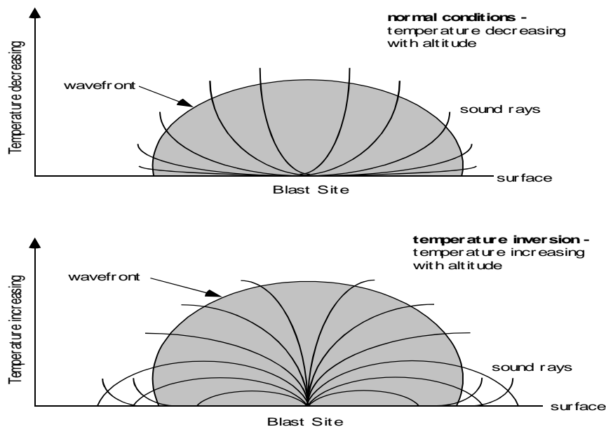
Figures 2 and 3 Normal Conditions where Airblast dissipates into the atmosphere versus Inversion Conditions Causing Airblast Waves to Bend Down to Earth after J Floyd Efficient Blasting Techniques Course 2005
