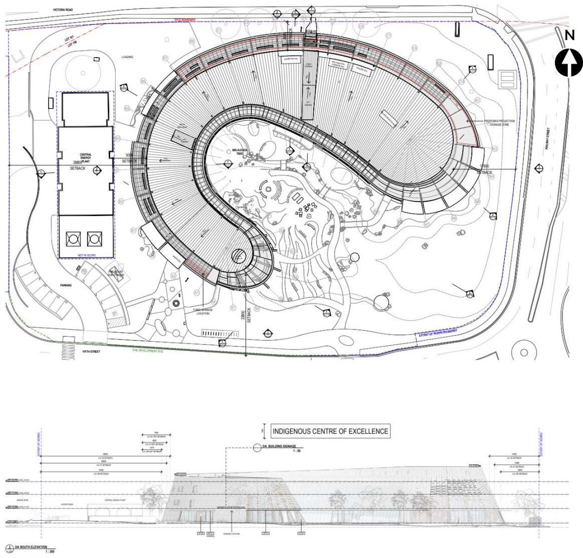
Figure 2: Roof plan (top) and South Elevation (bottom) of proposed development
