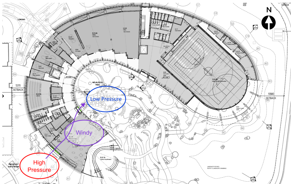
Figure 5: Diaphragm highlighting potential for wind flowing through open doors on the ground floor during south-westerly winds.
