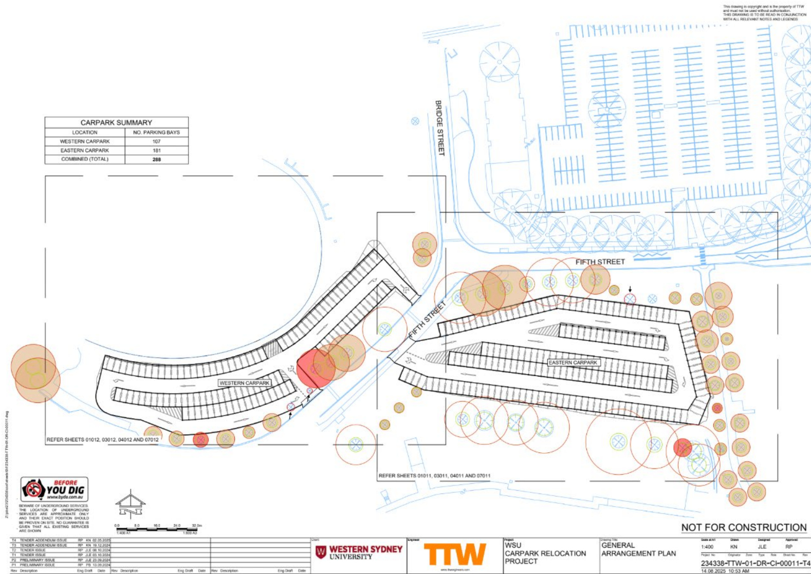
Figure 3. General Arrangement Plan for the Proposed Carparks (TTW 2025) - The black arrows indicate trees proposed for removal
