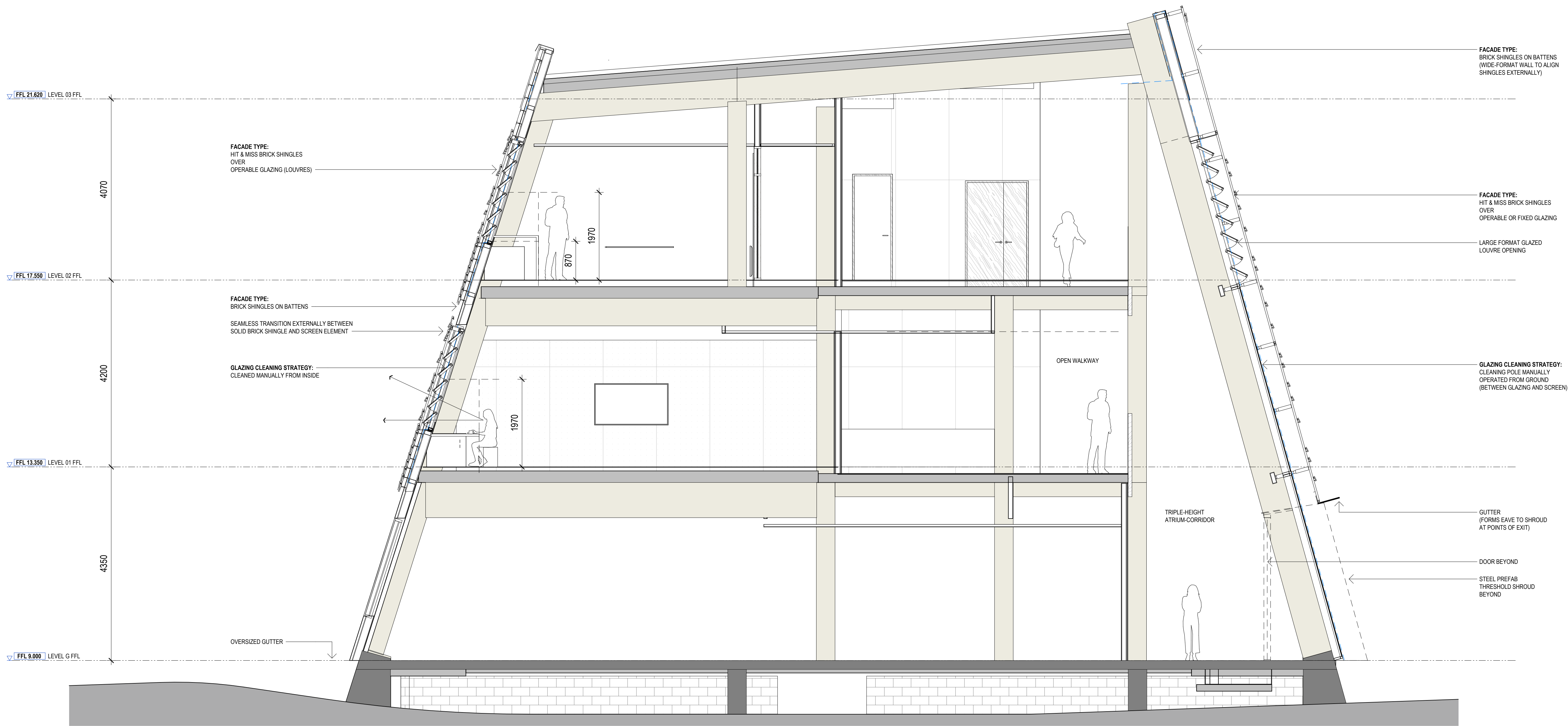
1 TYPICAL FAÇADE SECTION 01 1 : 50
