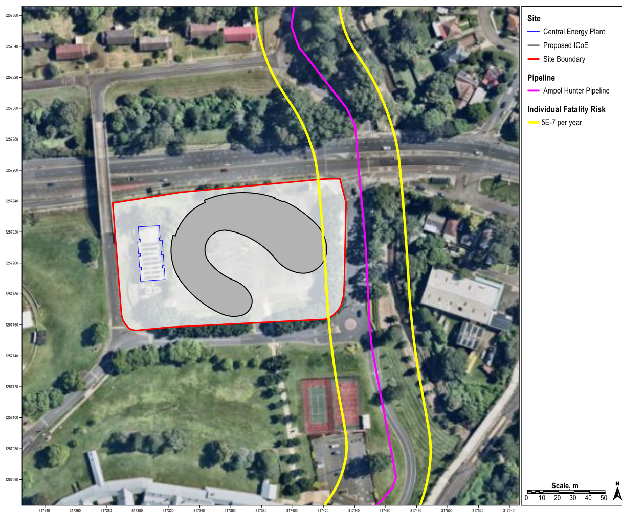
Figure 8.1: Individual fatality risk contours
