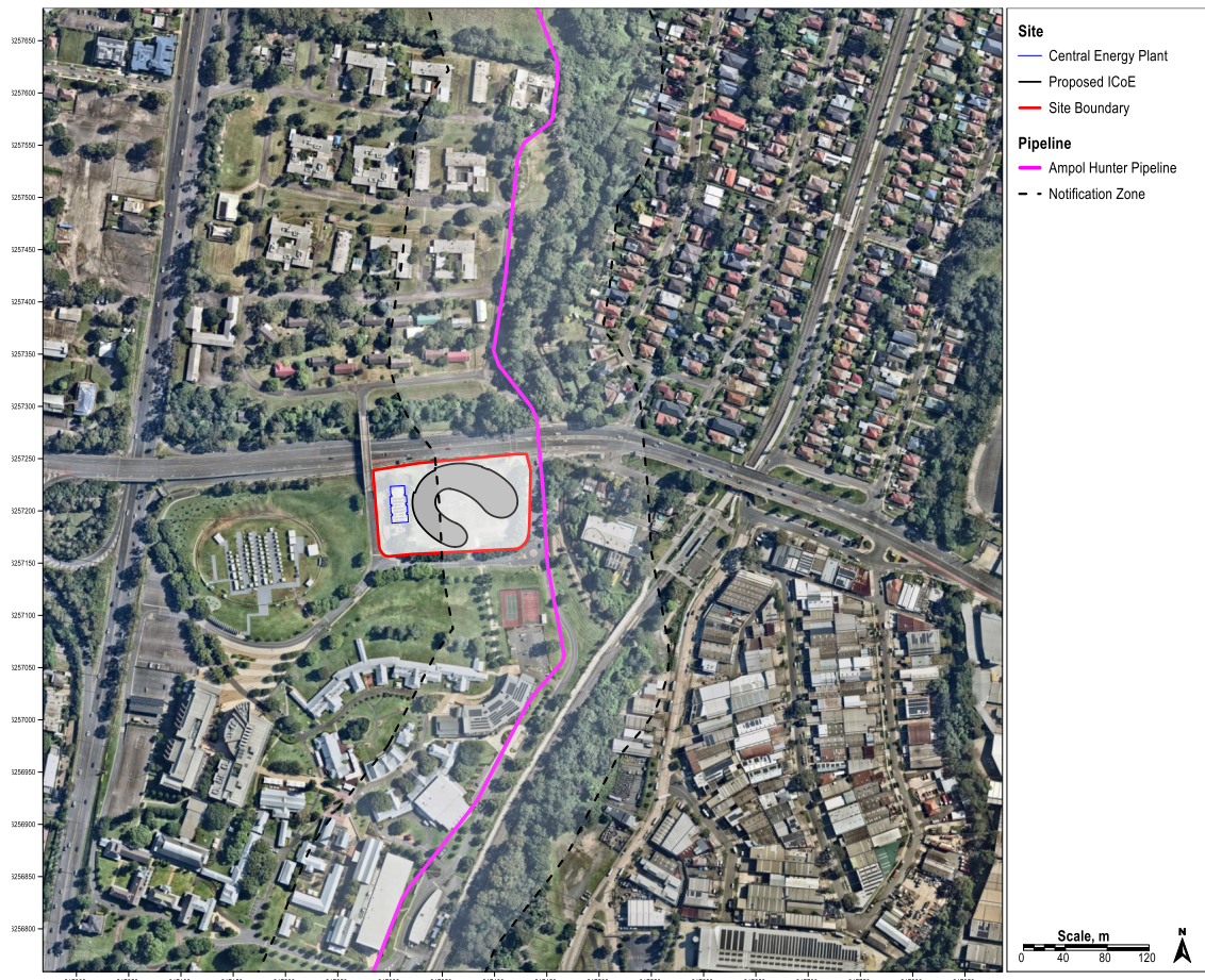
Figure 4.3: Hunter Pipeline route
