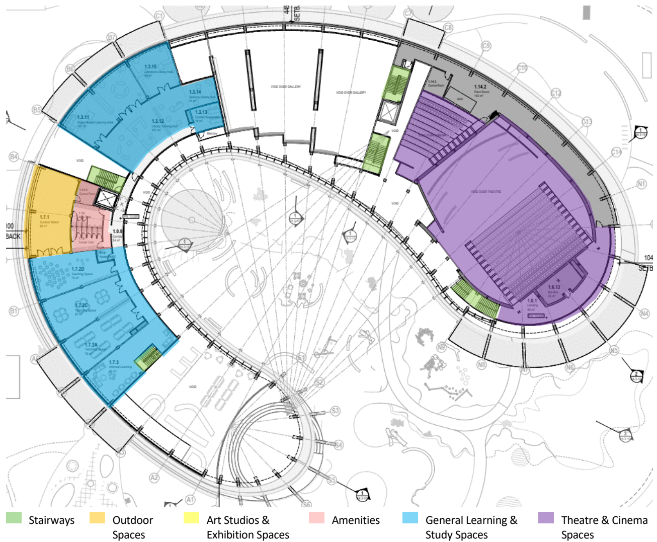
Figure 2.5: Floor Plan – Level 1
