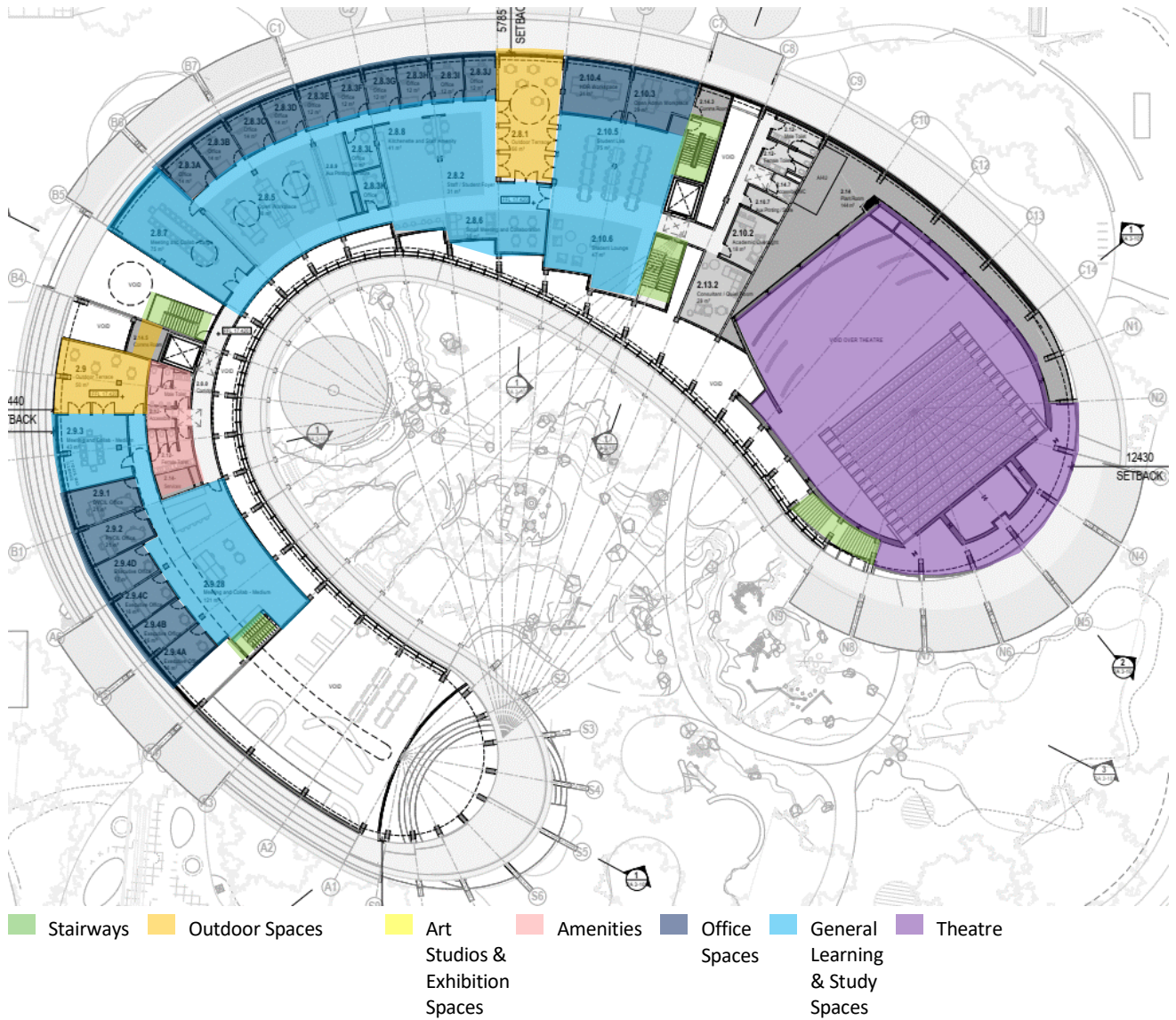
Figure 2.6: Floor Plan – Level 2
