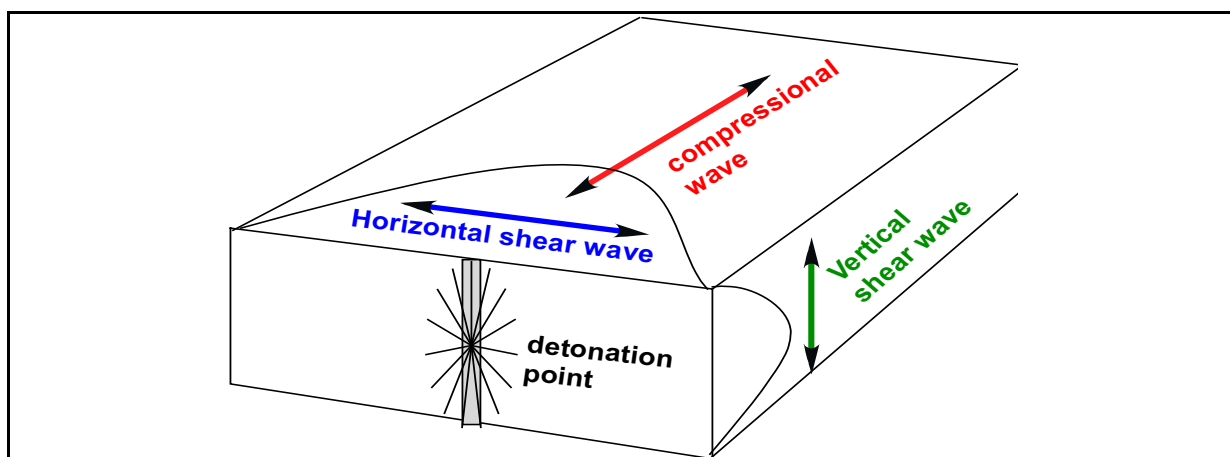
Figure 1: Ground vibration components showing Compression wave, Horizontal Shear wave and Vertical Shear wave.
