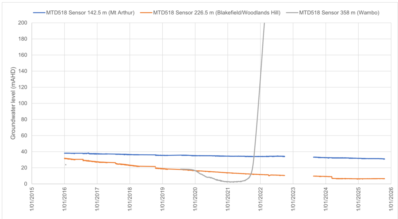
Figure D 9 VWP MTD518 pressure heads
