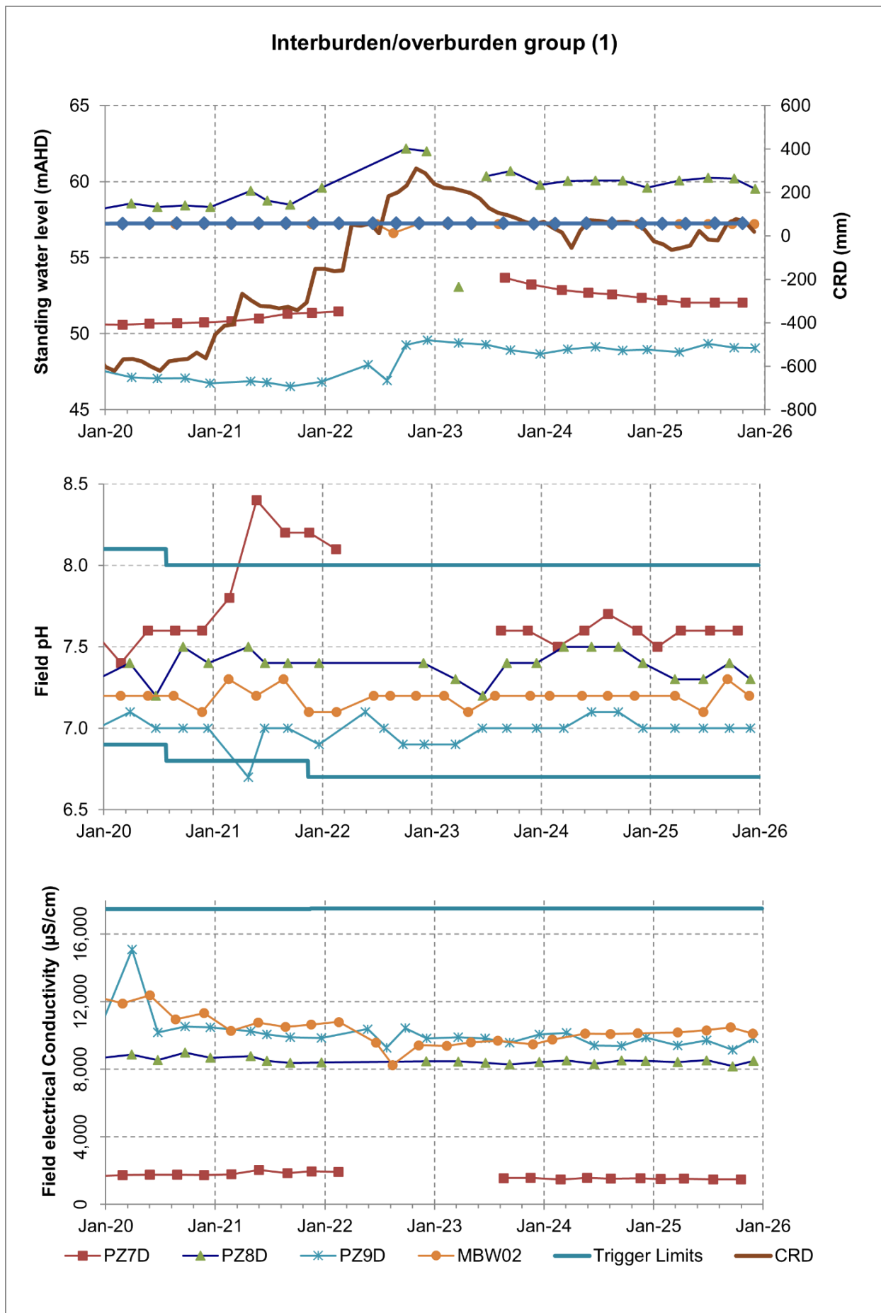
Figure B 7 Shallow overburden bores GWL, pH, and EC (1)
