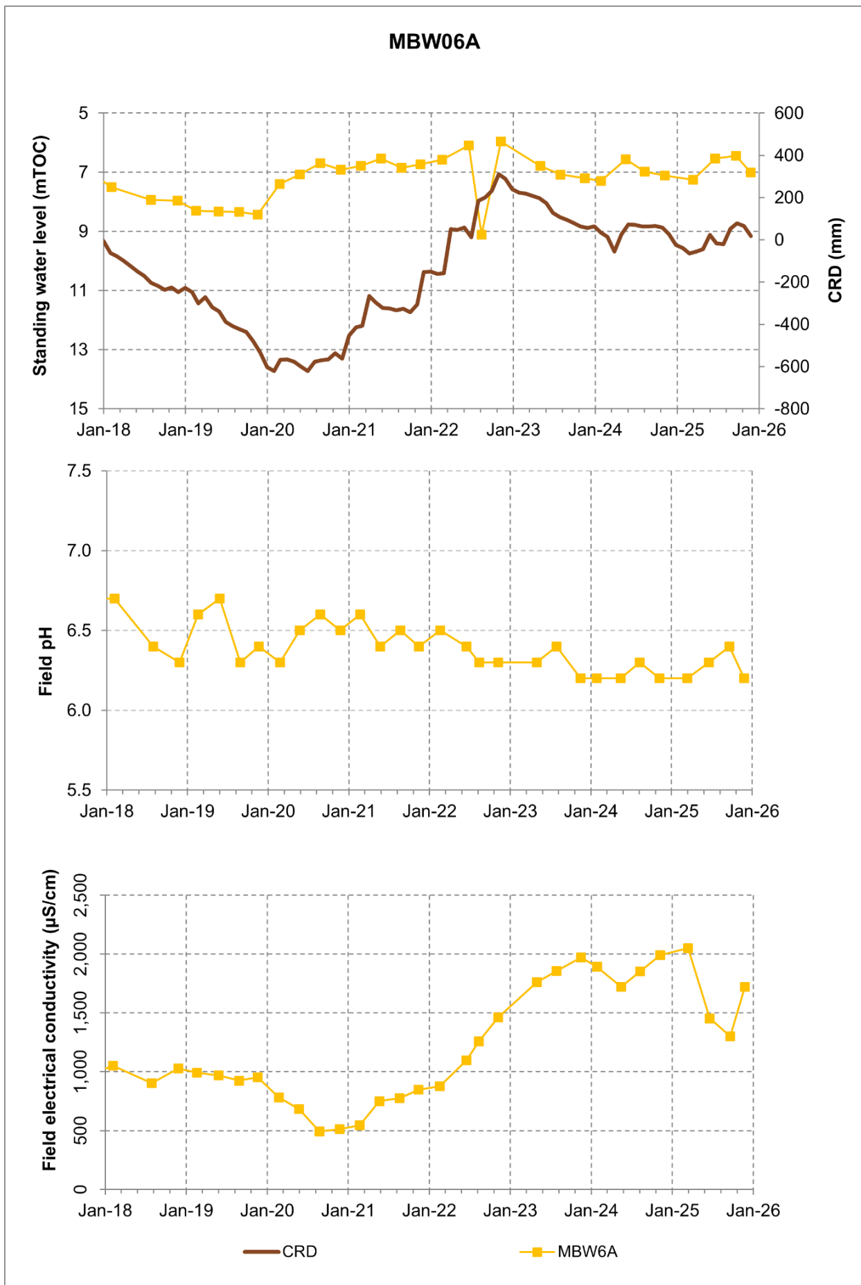
Figure B 24 MBW06 GWL, pH, and EC
