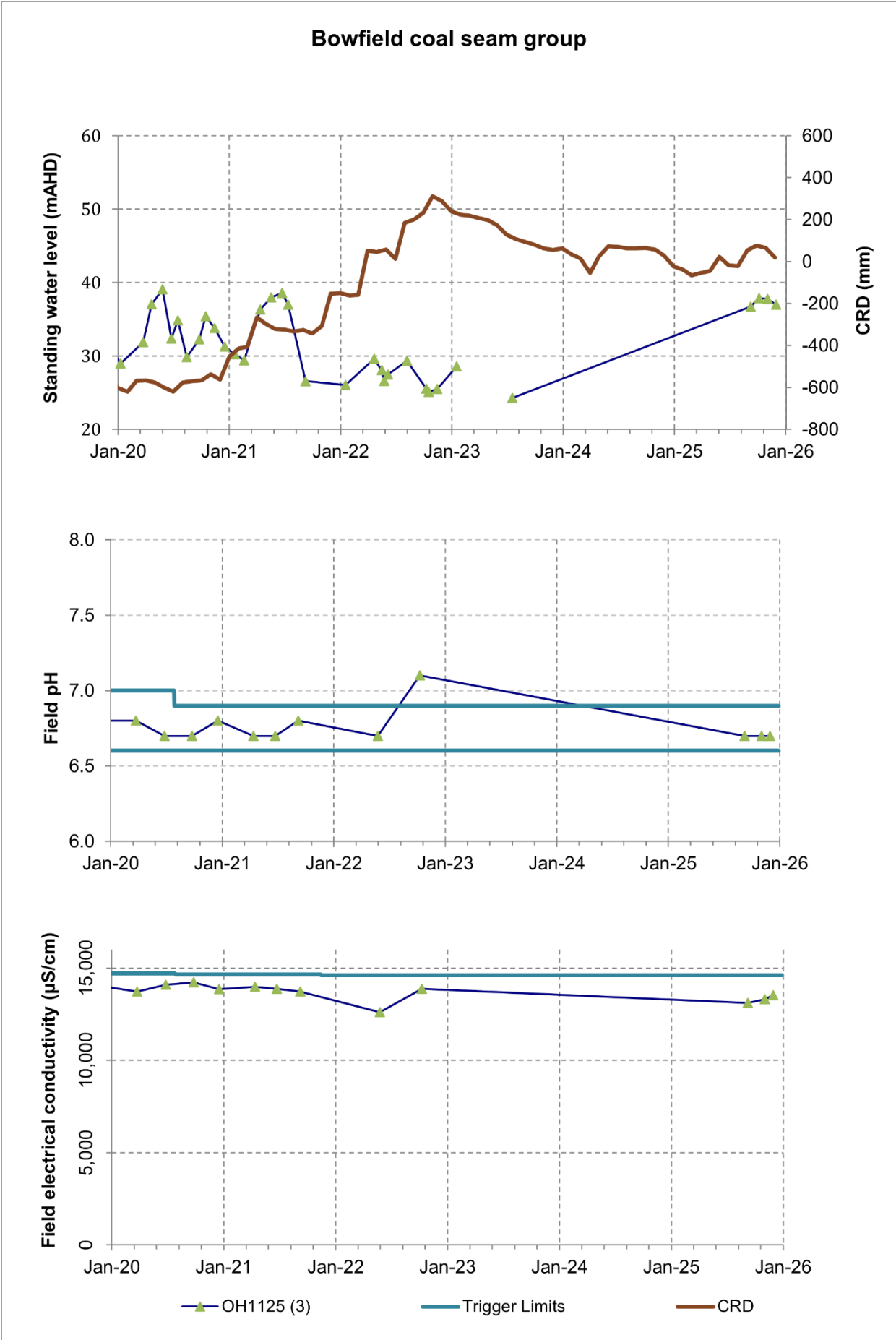
Figure B 4 Bowfield coal seam bores GWL, pH, and EC
