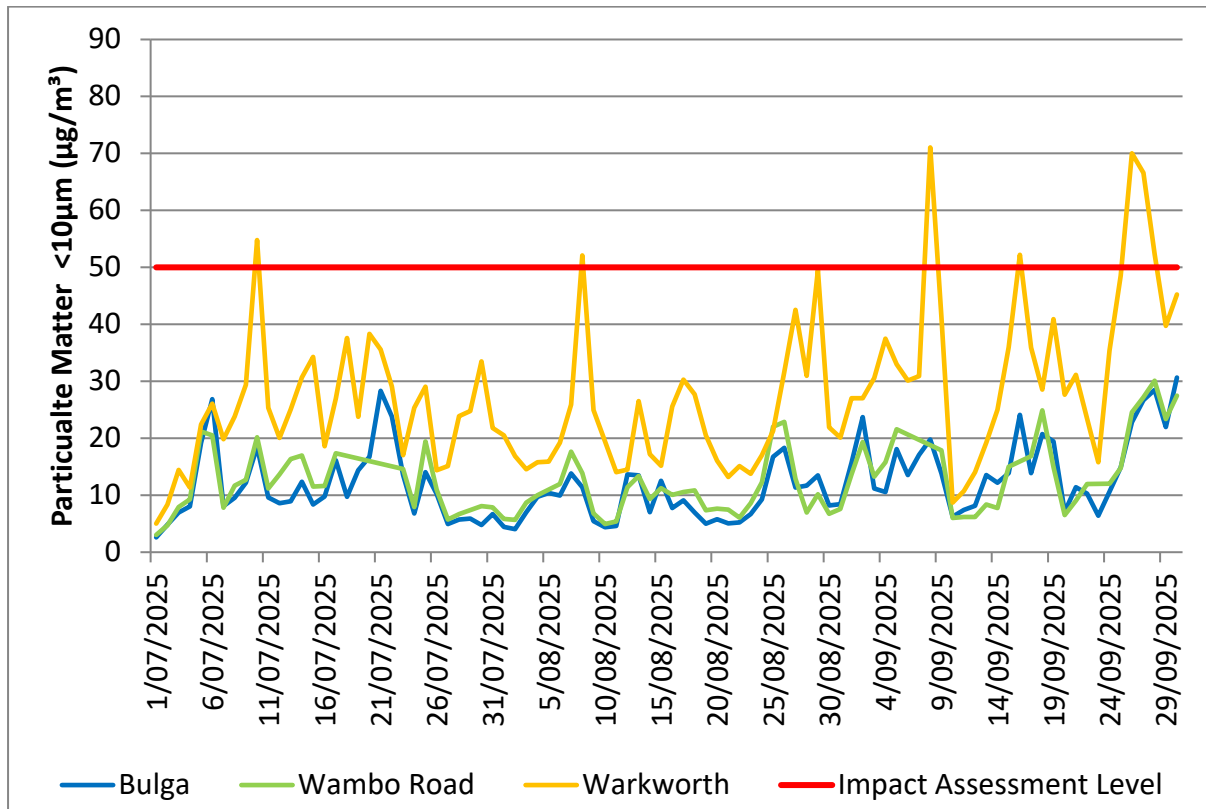
FIGURE 20: 24HR AVERAGE PM10 MEASURED AT TEOM MONITORS SURROUNDING MTW - QUARTER THREE 2025
