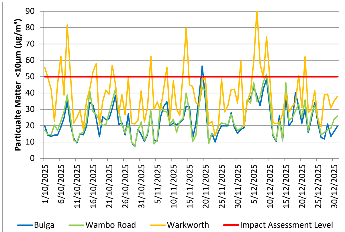
FIGURE 21: 24HR AVERAGE PM 10 MEASURED AT TEOM MONITORS SURROUNDING MTW - QUARTER FOUR 2025
