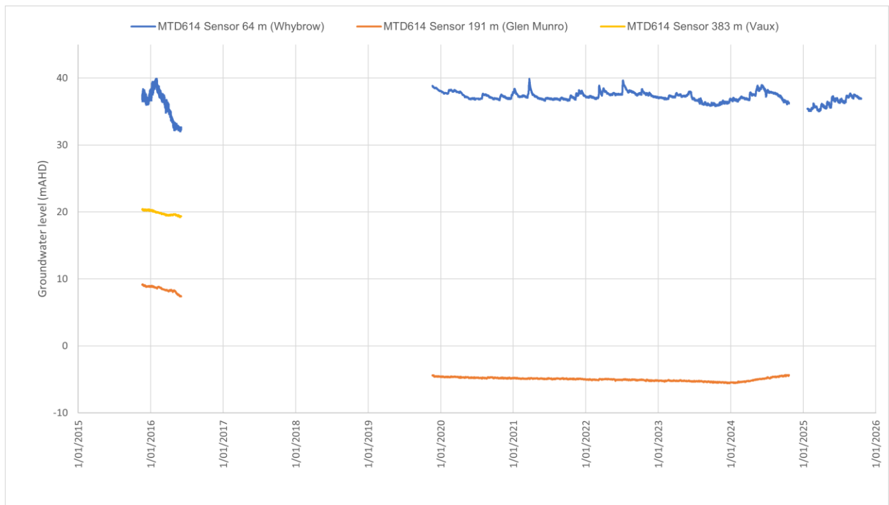
Figure D 8 VWP MTD614 pressure heads
