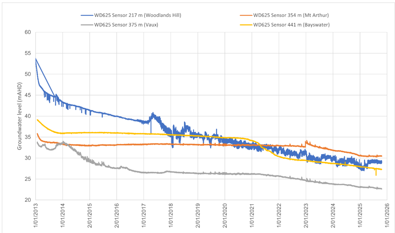
Figure D 3 VWP WD625 pressure heads
