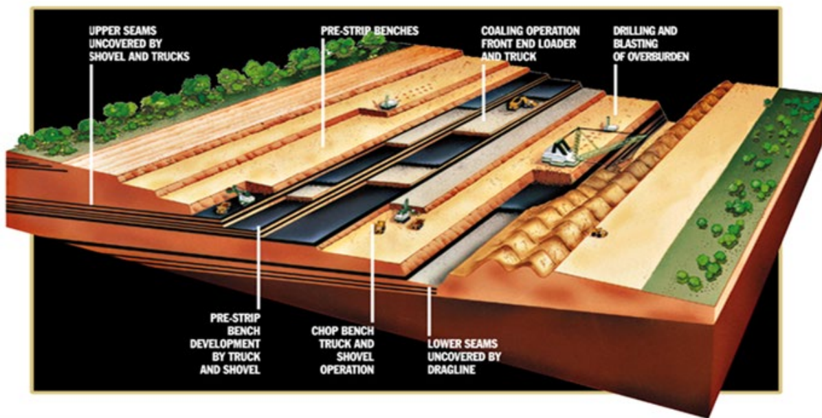
FIGURE 4: MINING PROCESS
