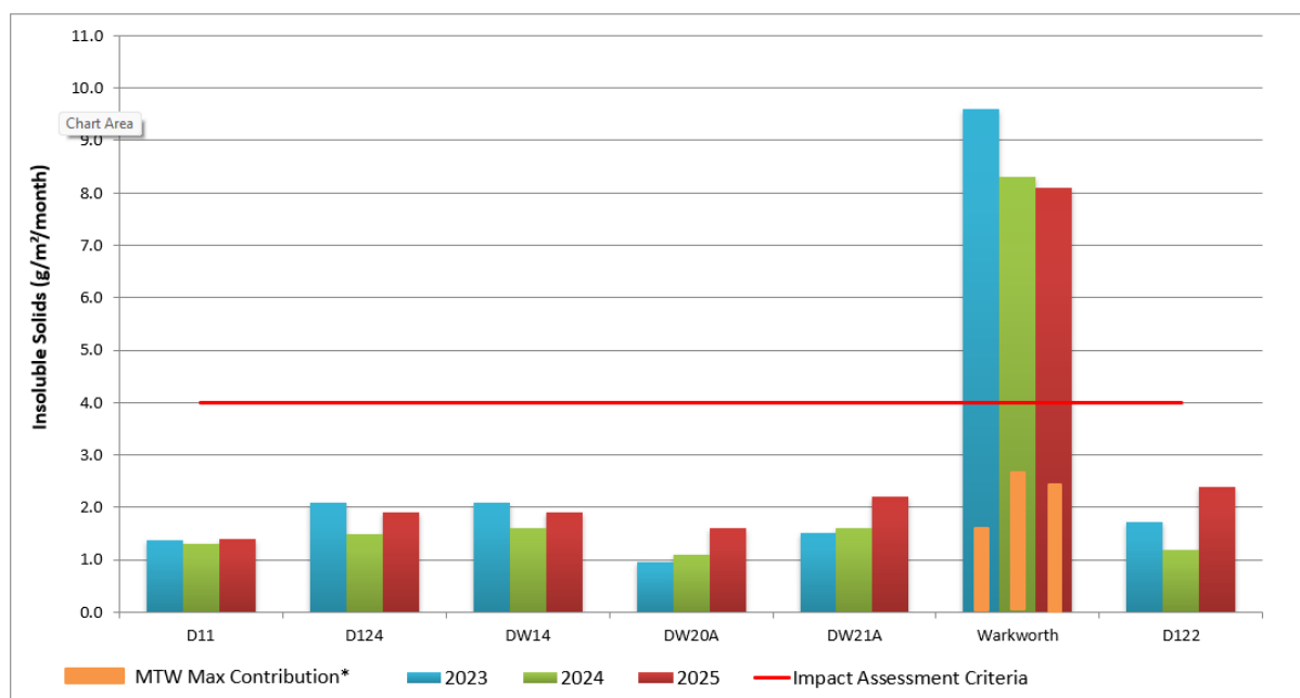
FIGURE 15: 2025 DEPOSITIONAL DUST RESULTS COMPARED AGAINST THE IMPACT ASSESSMENT CRITERIA AND PREVIOUS YEARS' RESULTS
