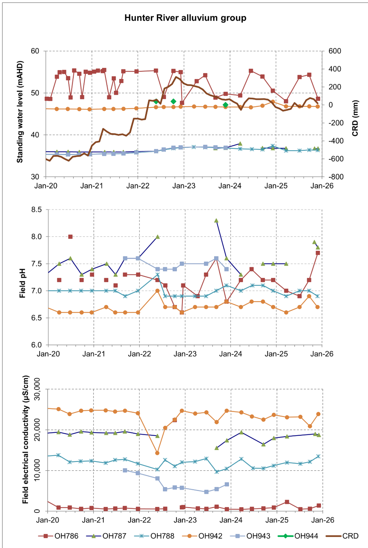
Figure B 9 Hunter River alluvium bores GWL, pH, and EC
