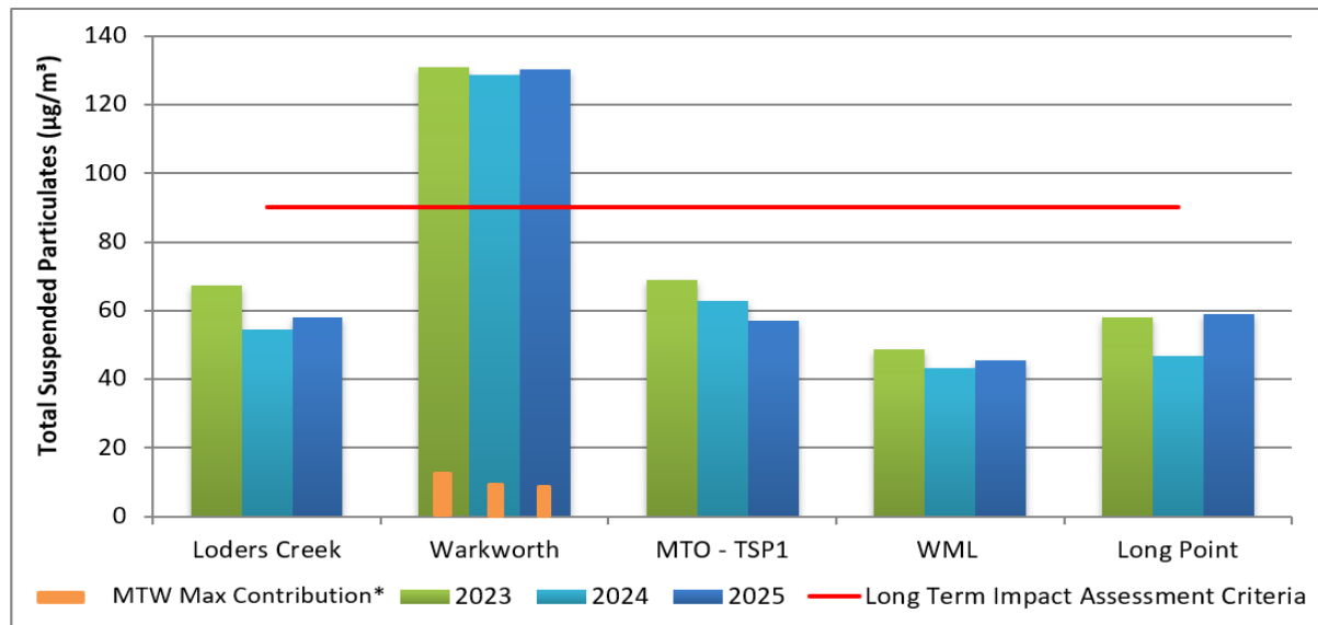
FIGURE 16: 2025 TSP ANNUAL AVERAGE COMPARED AGAINST THE IMPACT ASSESSMENT CRITERIA AND PREVIOUS YEARS' RESULTS
