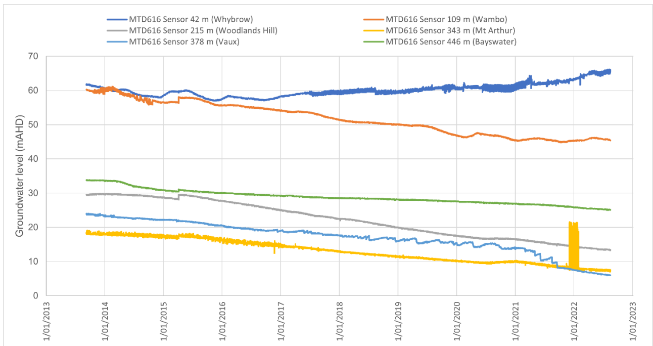
Figure D 5 VWP MTD616 pressure heads
