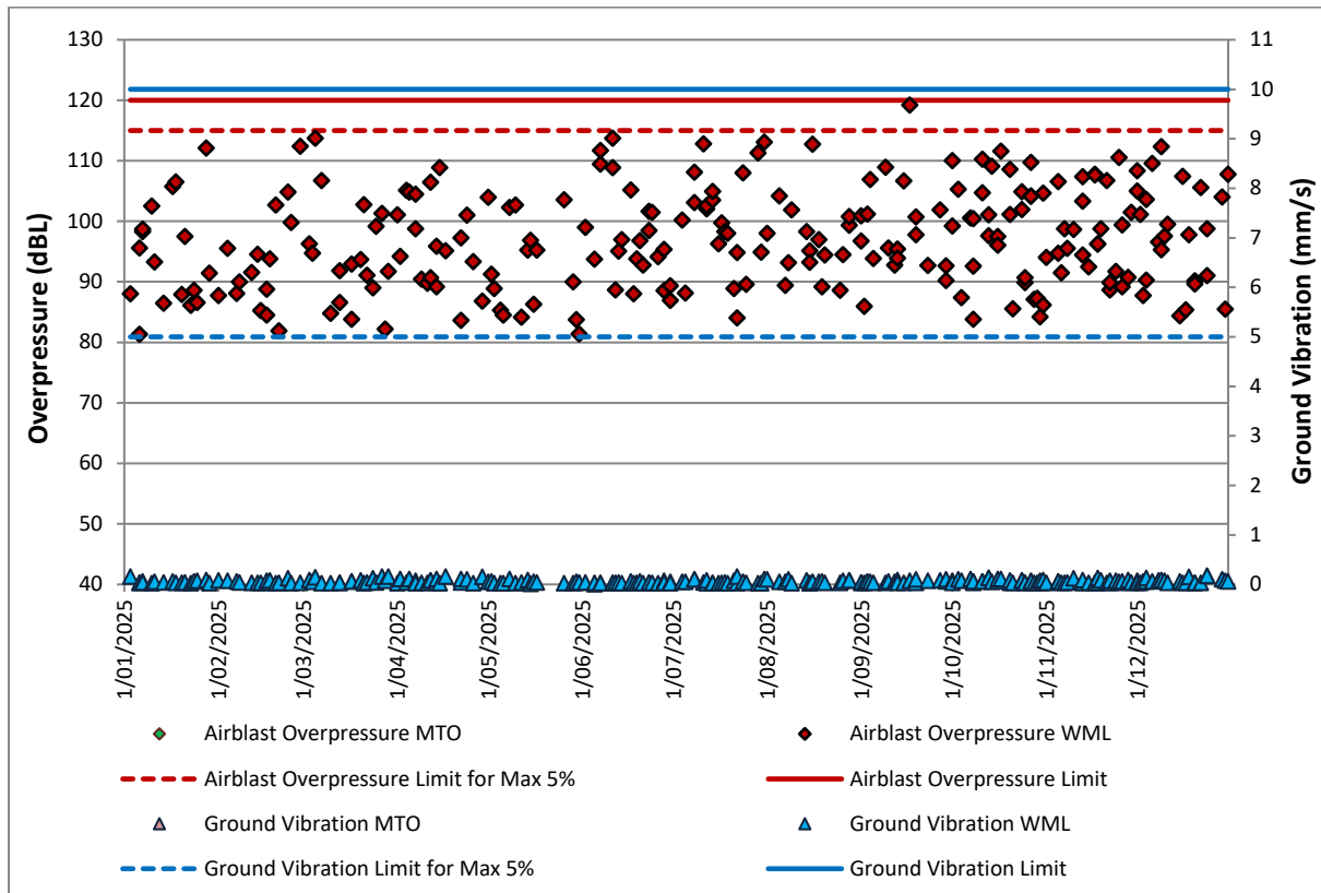
FIGURE 6: ABBEY GREEN BLAST RESULTS
