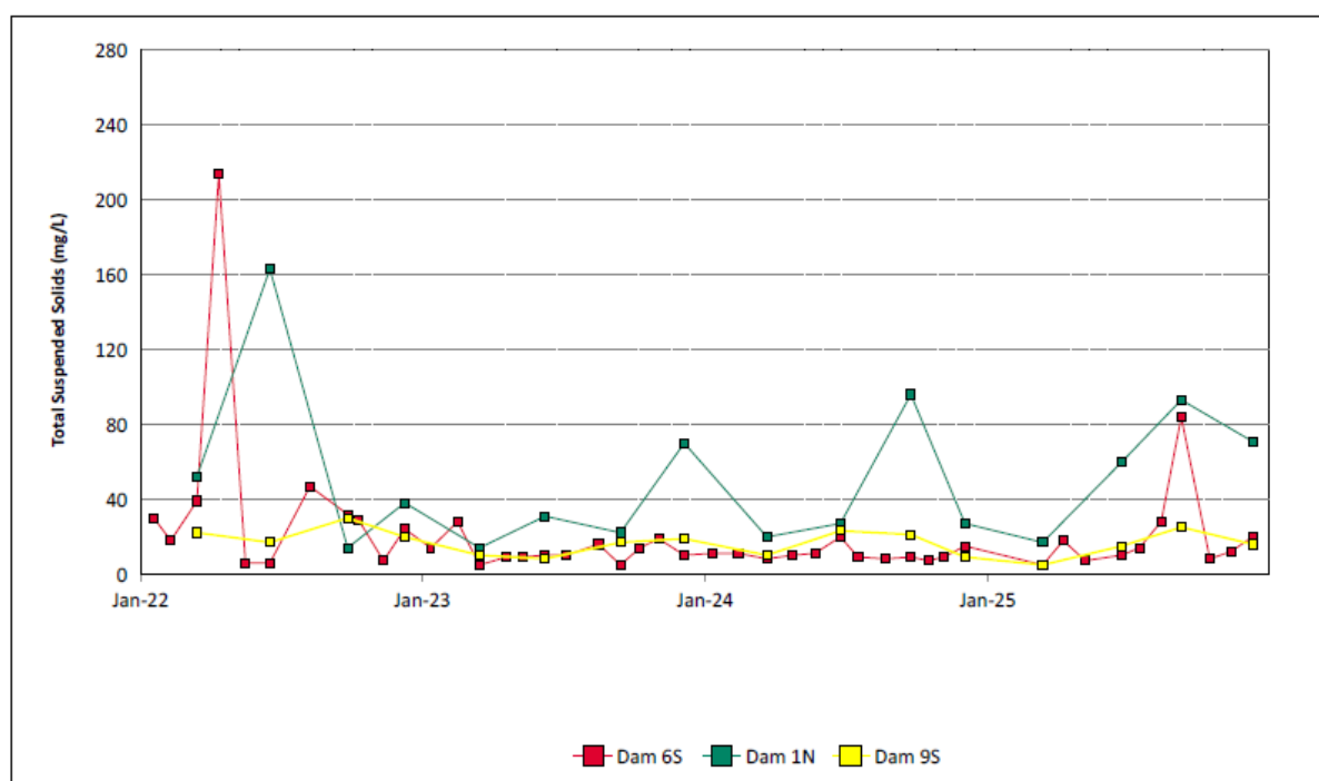
FIGURE 34: SITE DAMS TSS TRENDS 2022 TO 2025
