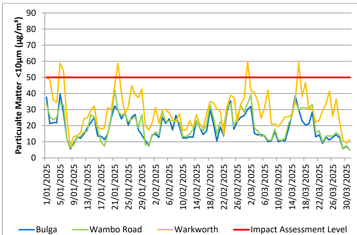
FIGURE 18: 24HR AVERAGE PM10 MEASURED AT TEOM MONITORS SURROUNDING MTW - QUARTER ONE 2025
