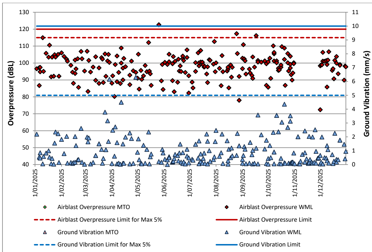
FIGURE 7: BULGA VILLAGE BLAST RESULTS
