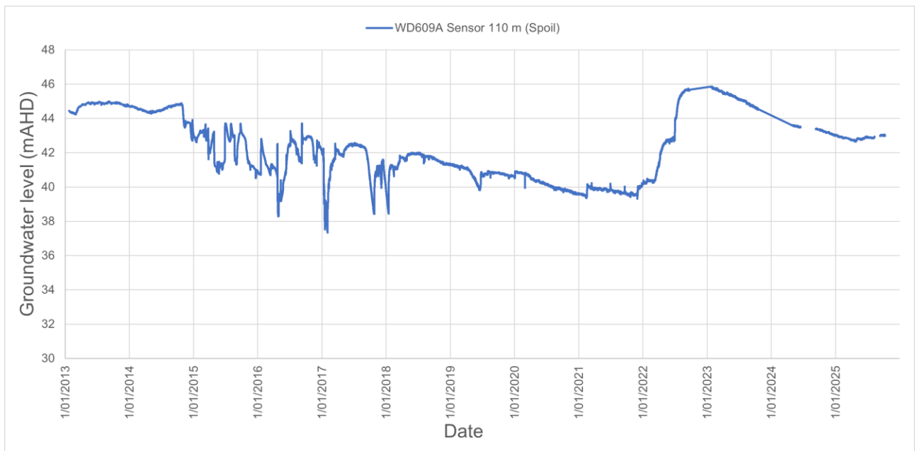
Figure D 1 VWP WD609A pressure head
