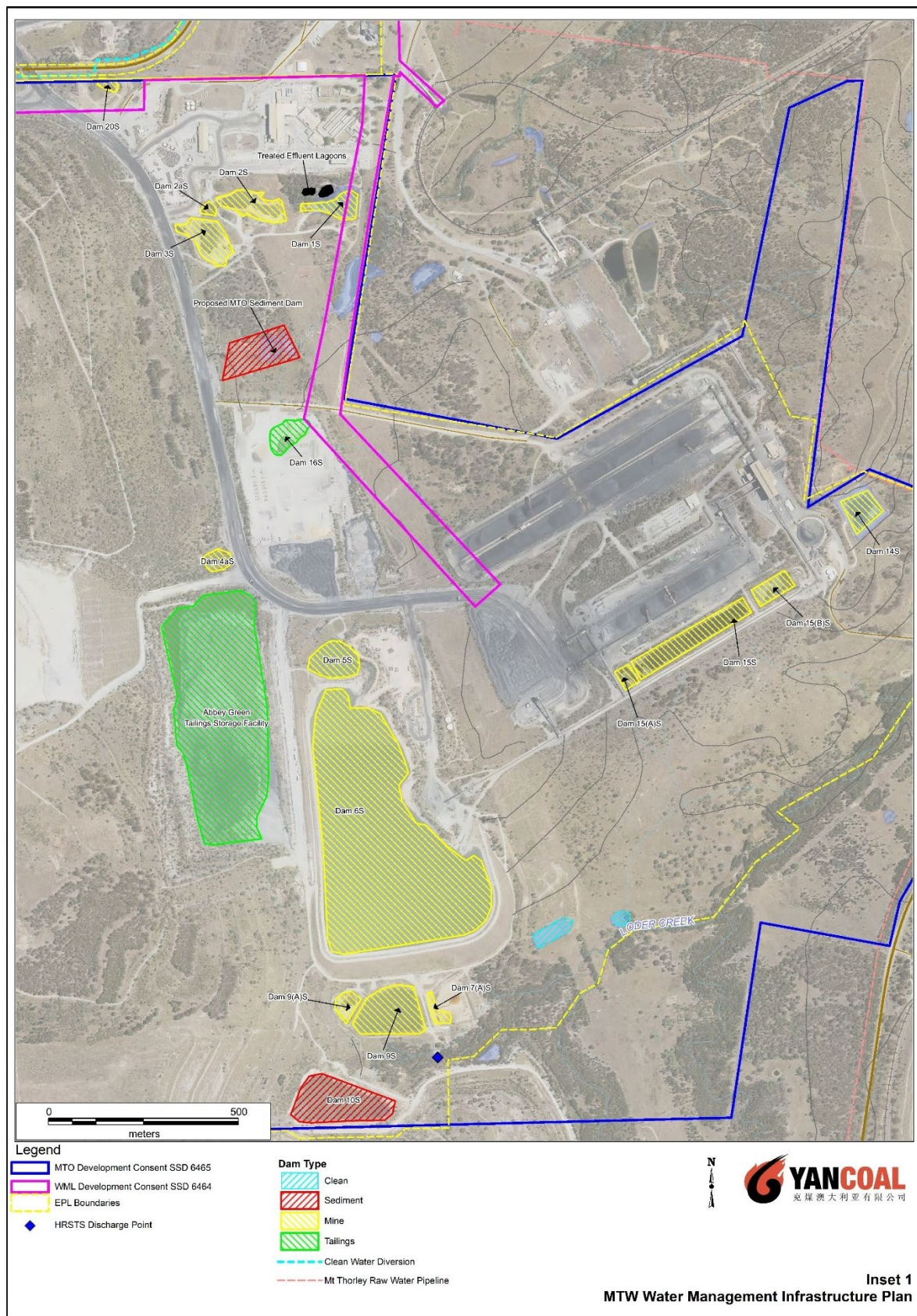
FIGURE 25A – MTW WATER MANAGEMENT INFRASTRUCTURE PLAN – INSET 1 (MTO DETAIL)
