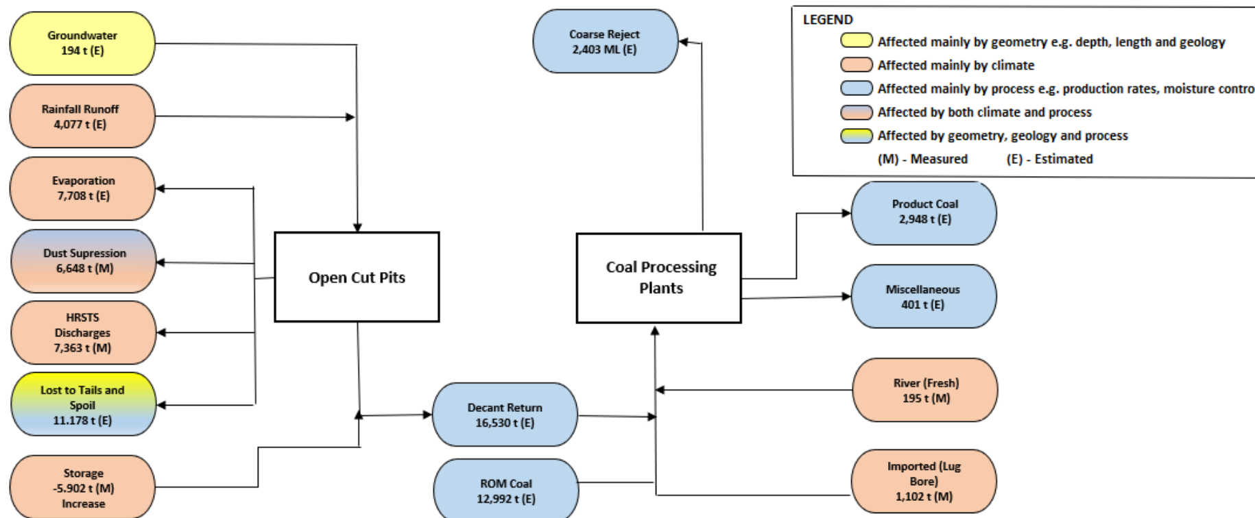
FIGURE 27: SCHEMATIC DIAGRAM MTW SALT FLUX
