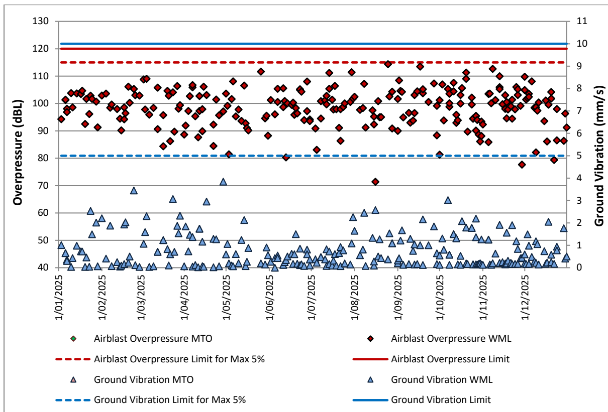
FIGURE 9: WOLLEMI PEAK ROAD BLAST RESULTS
