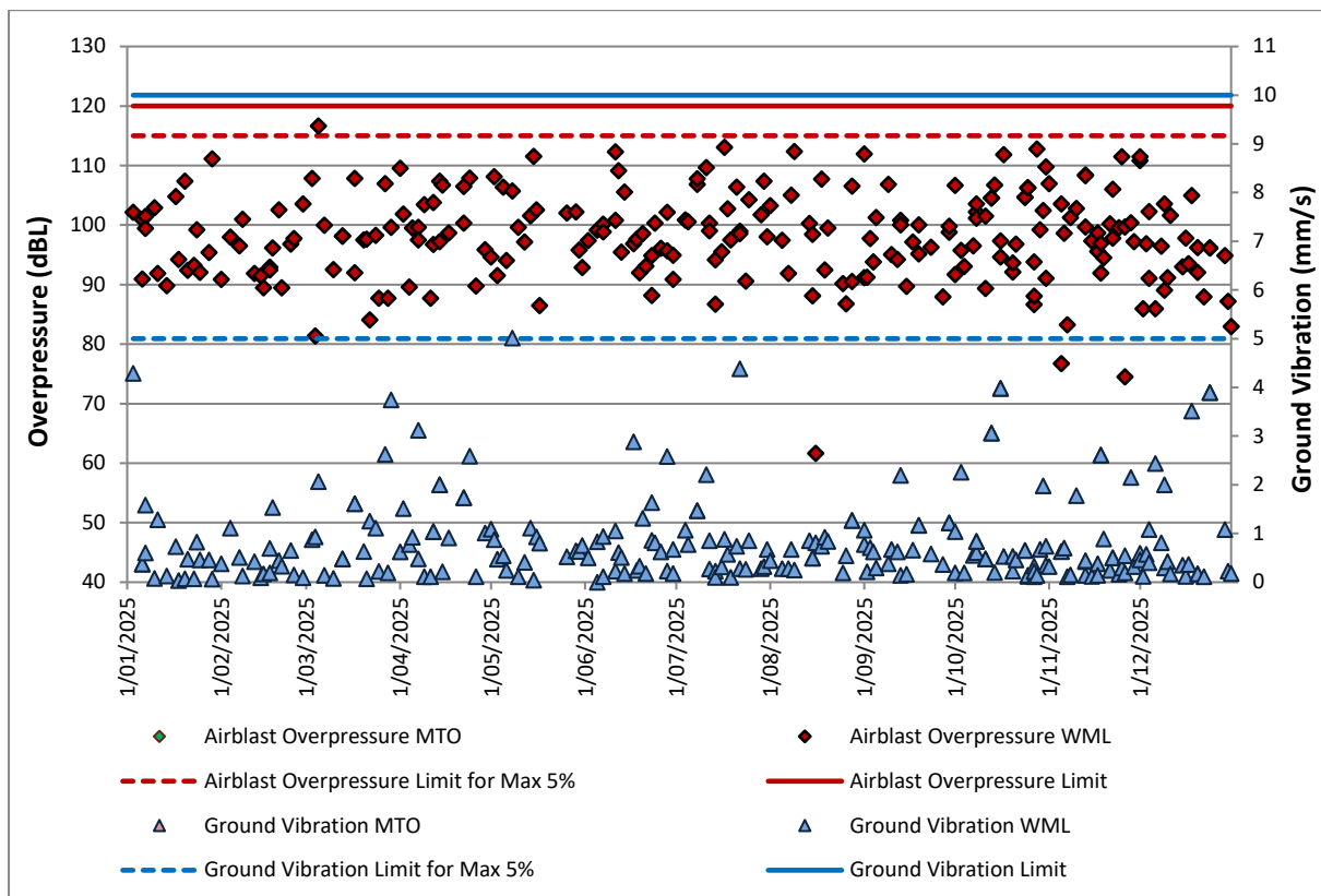
FIGURE 11: WARKWORTH BLAST RESULTS
