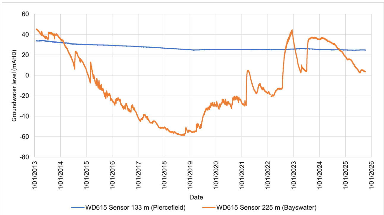
Figure D 2 VWP WD615 pressure heads
