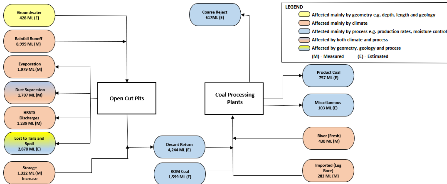
FIGURE 26: SCHEMATIC DIAGRAM MTW WATER FLUX
