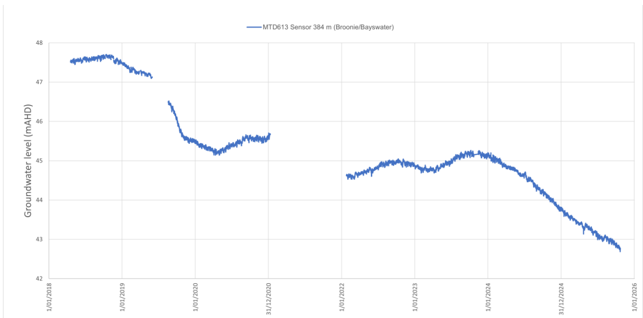
Figure D 6 VWP MTD613 pressure head
