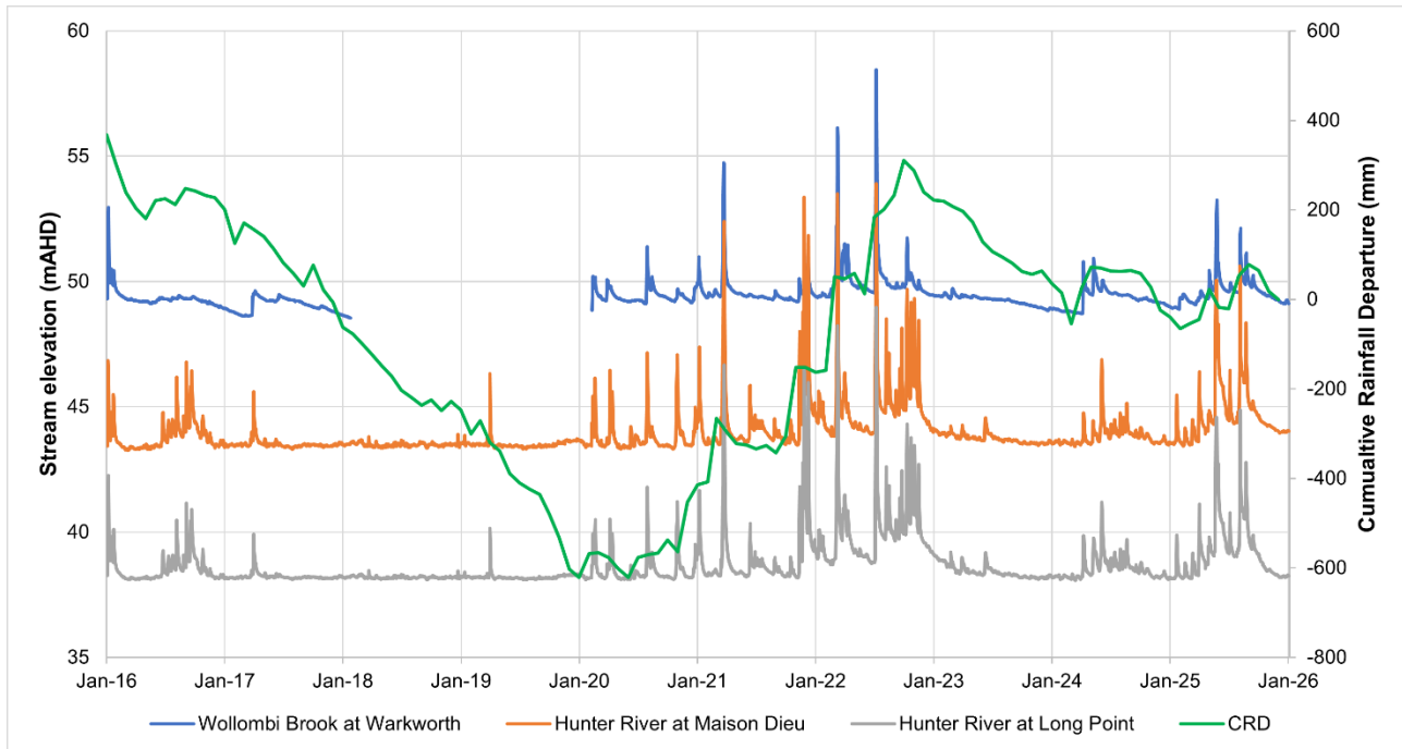
Figure 2.2 Surface water levels
