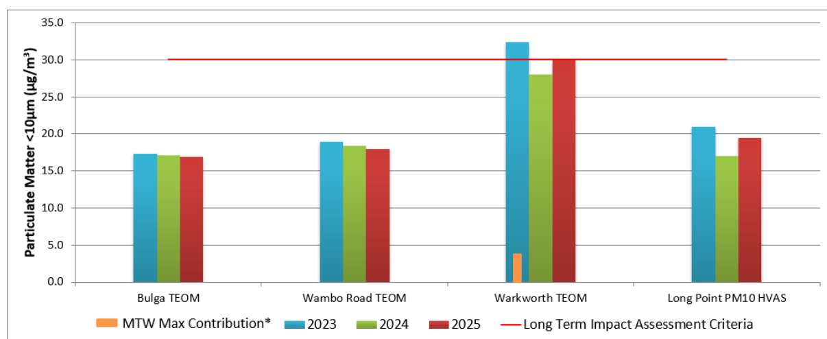
FIGURE 22: ANNUAL AVERAGE PM 10 RESULTS 2023 TO 2025
