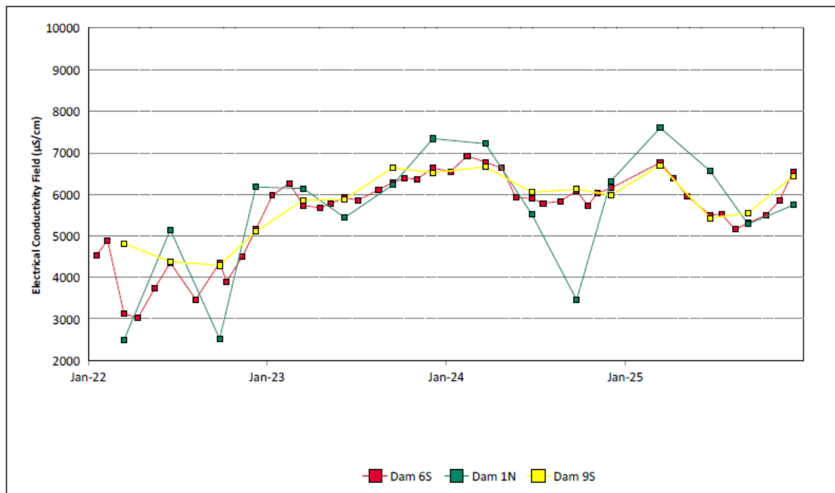
FIGURE 30: WATERCOURSE EC TRENDS 2022 TO 2025
