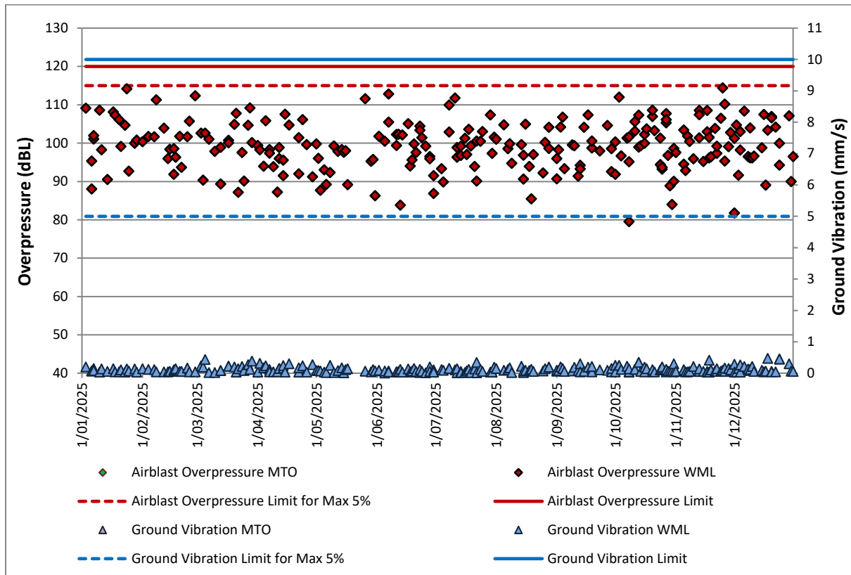
FIGURE 8: MTIE BLAST RESULTS
