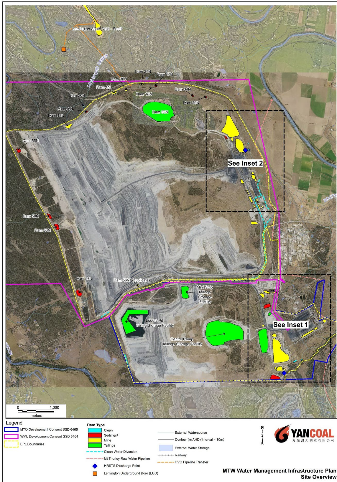
FIGURE 25: WATER MANAGEMENT INFRASTRUCTURE PLAN – SITE OVERVIEW
