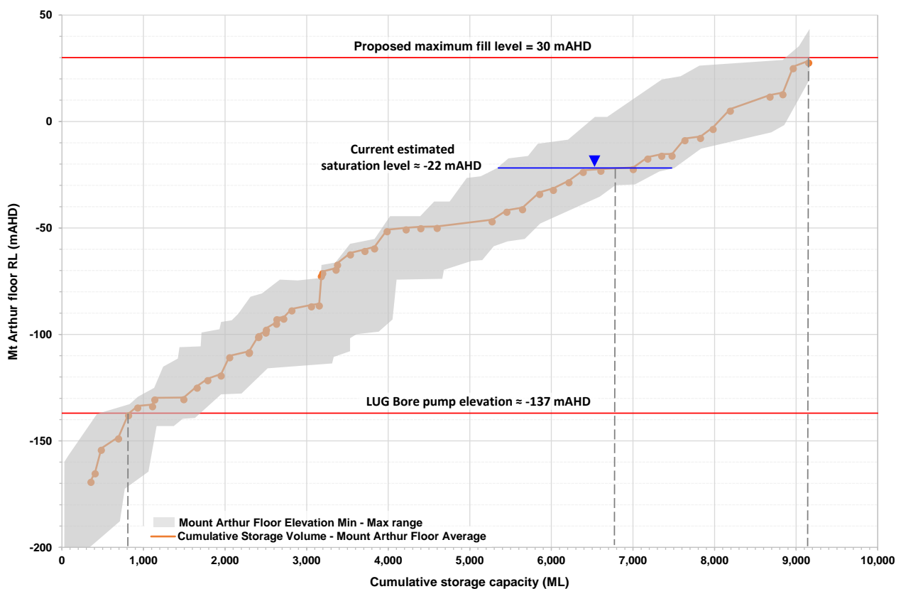
Figure 5.27 Estimated Lemington Underground storage curve
