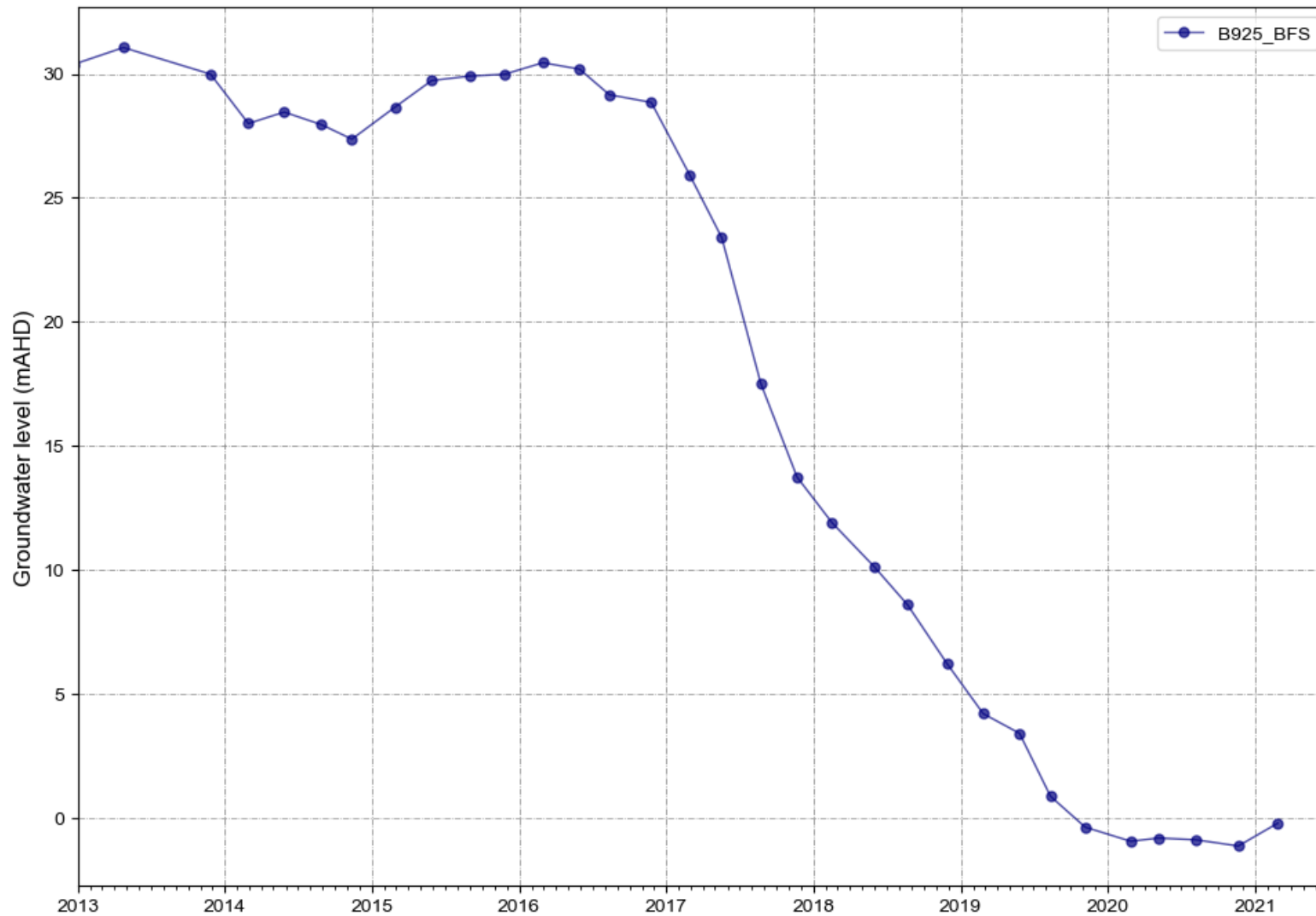
Figure A 19 B925_BFS water levels
