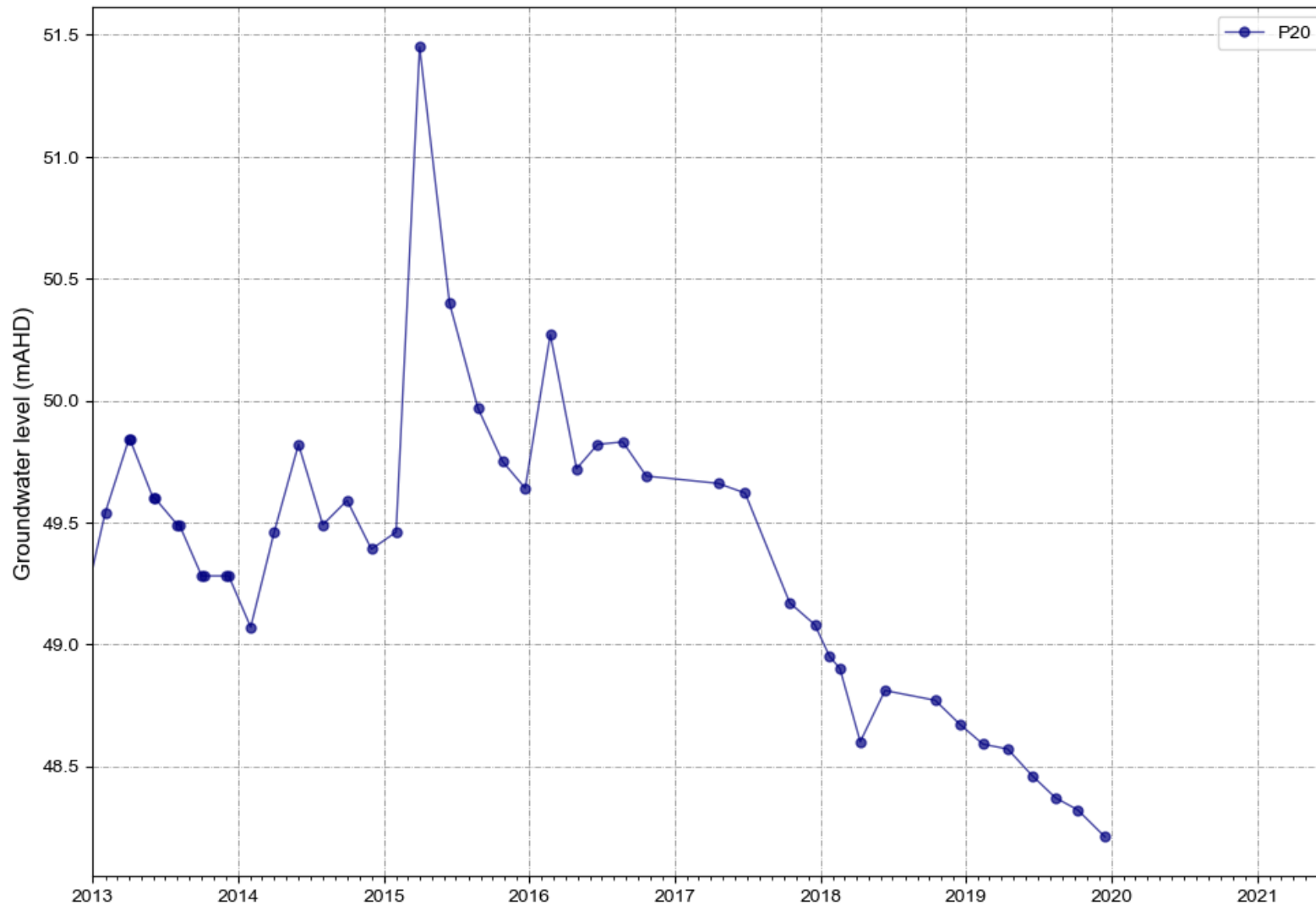
Figure A 50 P20 water levels
