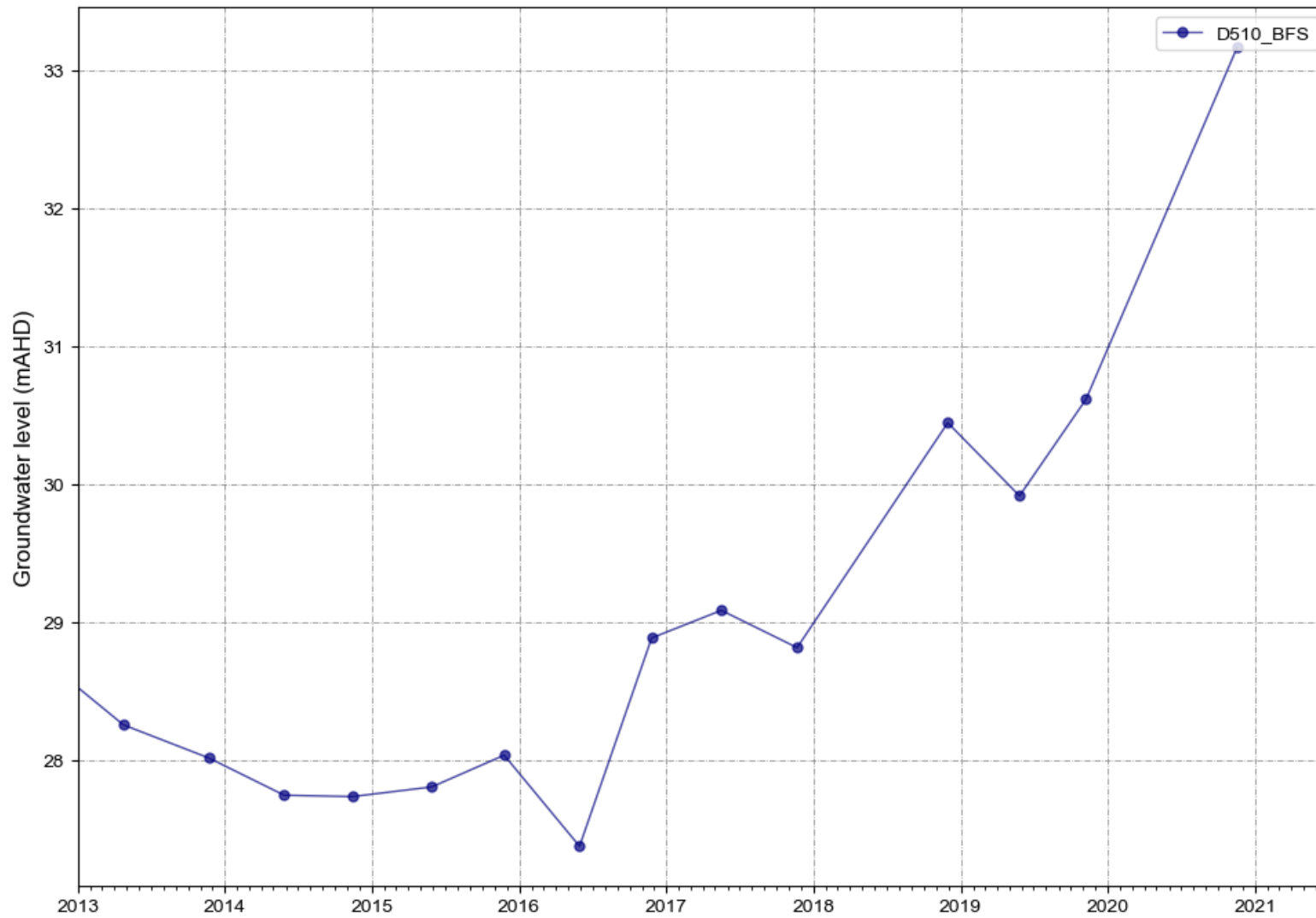
Figure A 29 D510_BFS water levels
