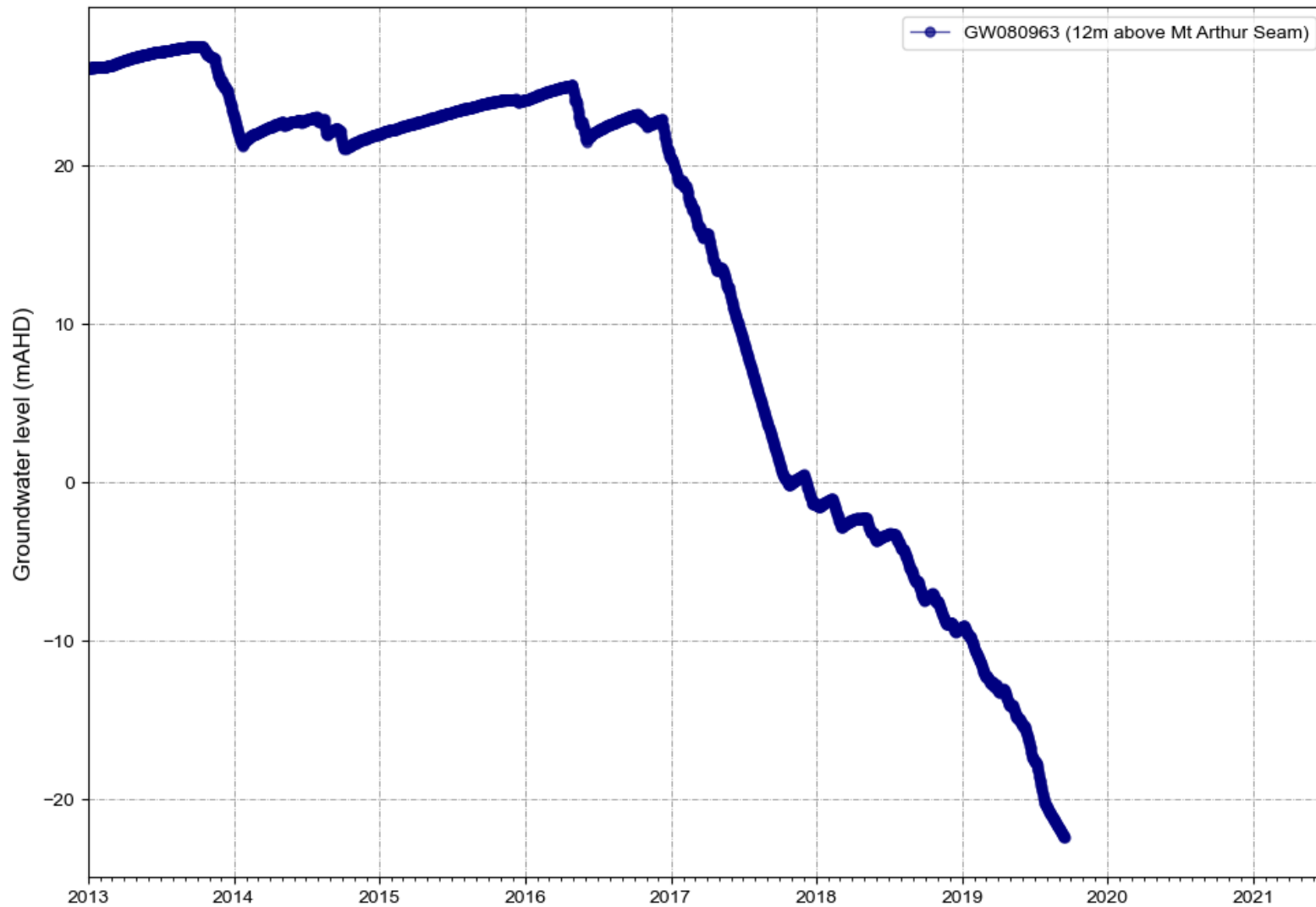
Figure A 2 GW080963 water levels
