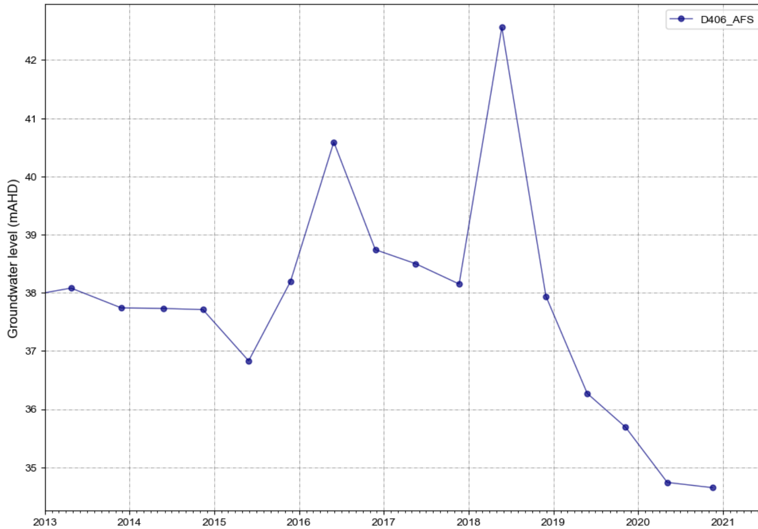
Figure A 33 D406_AFS water levels
