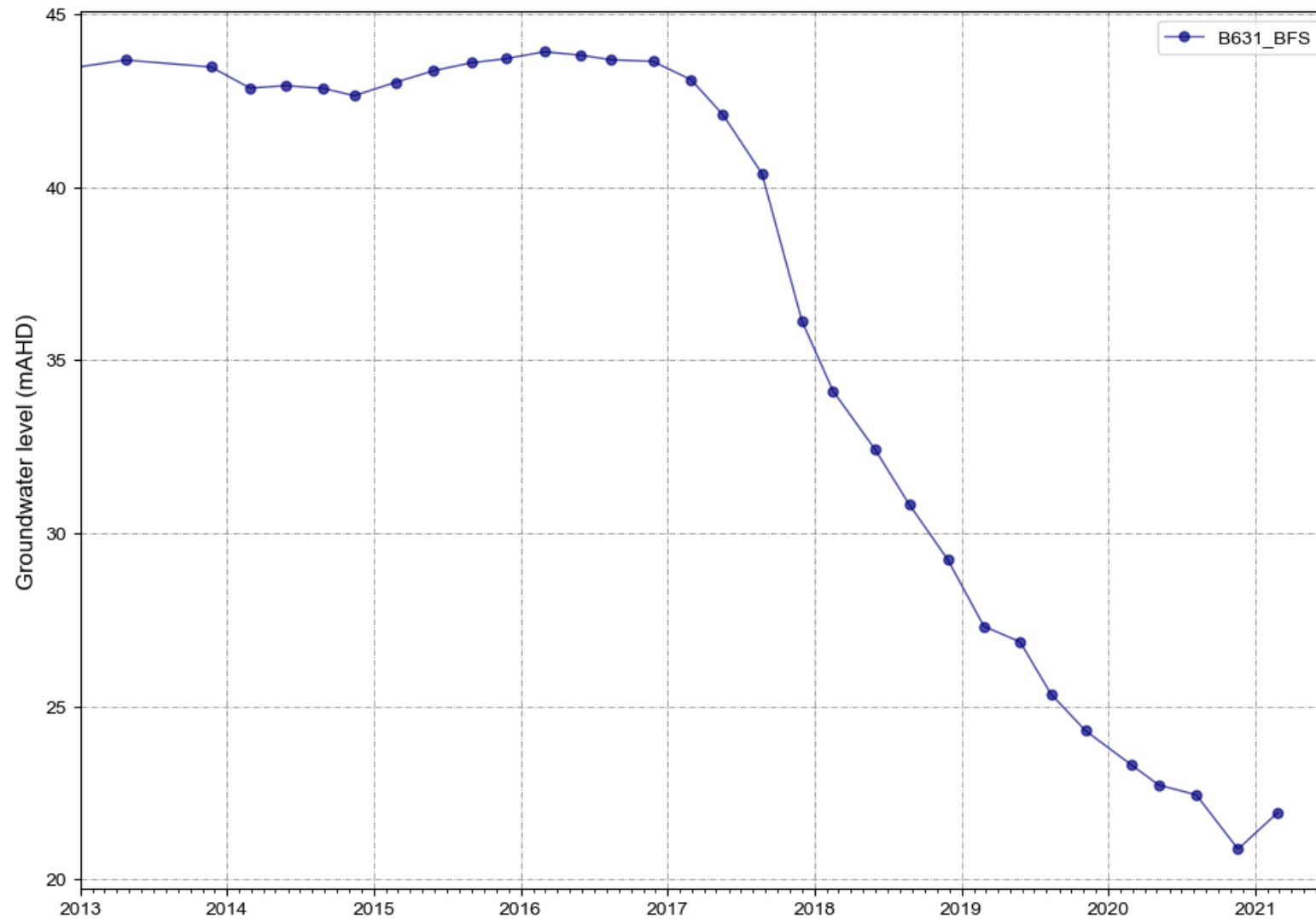
Figure A 18 B631_BFS water levels
