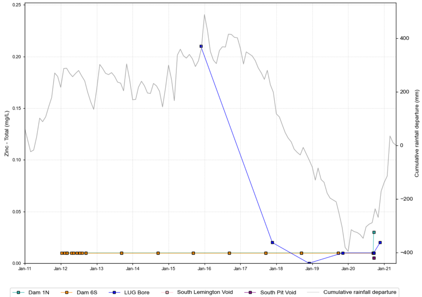
Figure B 13 MTW main surface water stores and LUG Bore, zinc time series data
