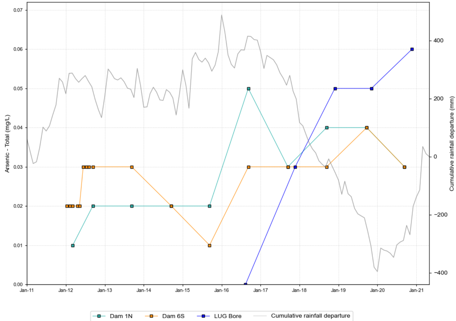
Figure B 2 MTW main surface water stores and LUG Bore, arsenic time series data
