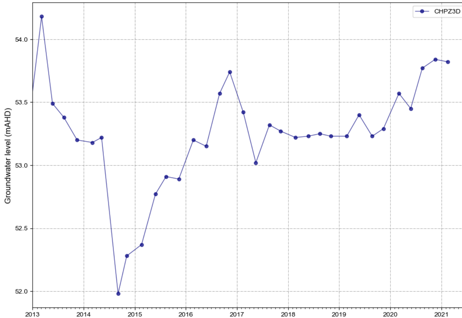
Figure A 11 CHPZ3D water levels
