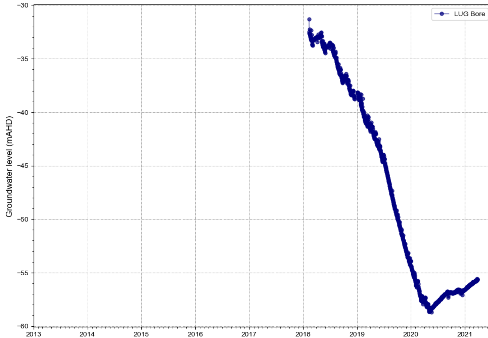
Figure A 1 LUG Bore water levels
