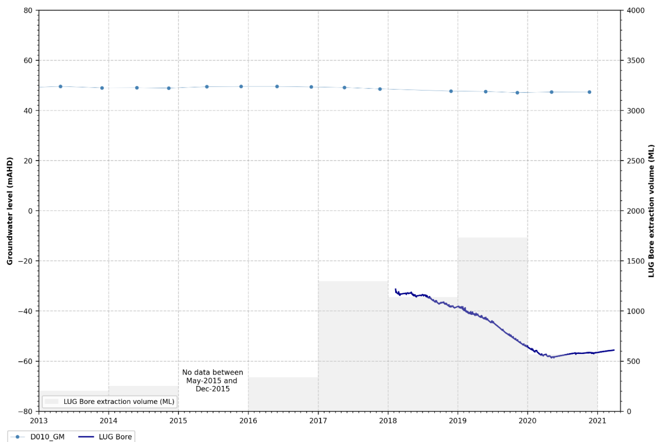
Figure 5.17 Groundwater levels Glen Munro coal seam
