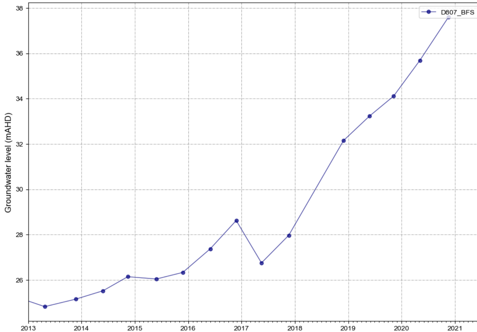
Figure A 31 D807_BFS water levels
