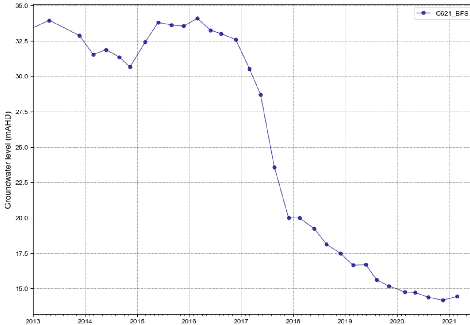
Figure A 23 C621_BFS water levels
