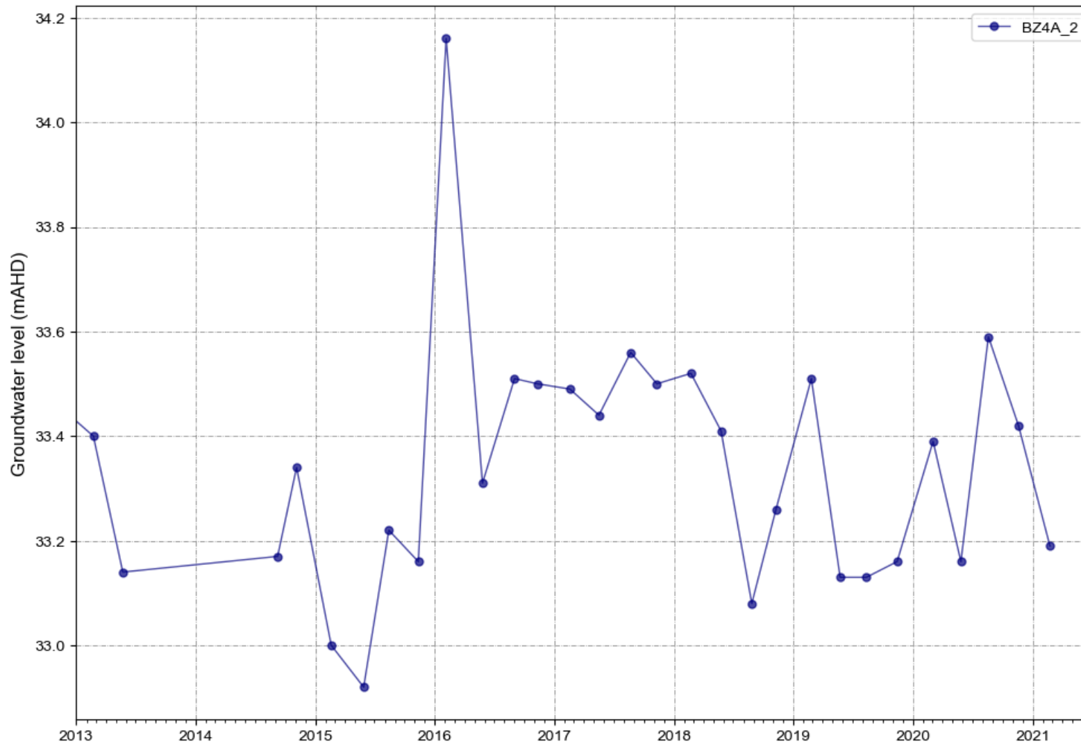
Figure A 10 BZ4A_2 water levels
