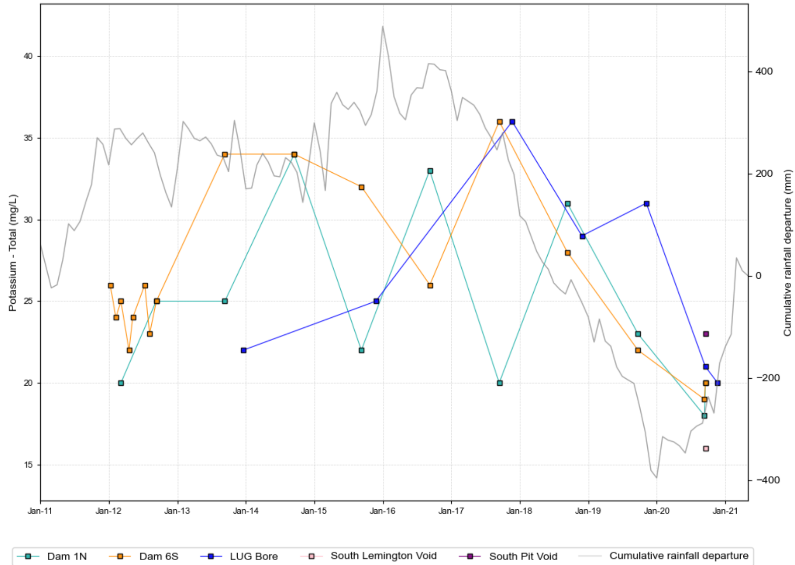
Figure B 10 MTW main surface water stores and LUG Bore, potassium time series data
