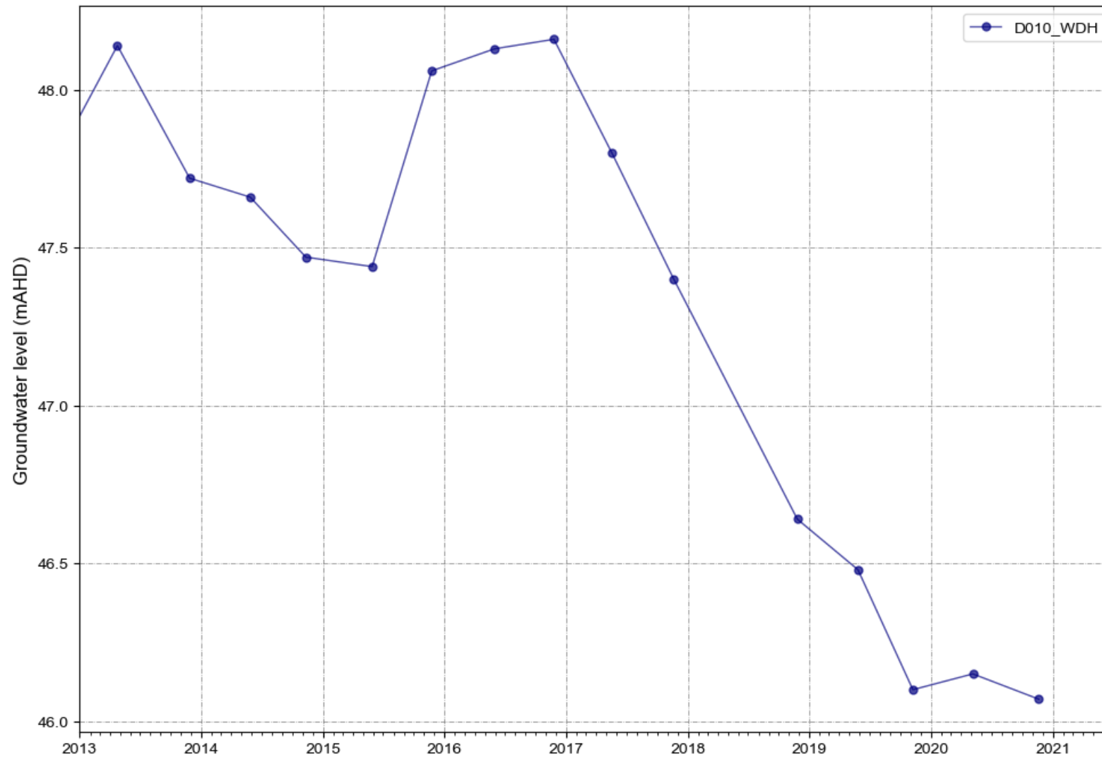
Figure A 43 D010_WDH water levels
