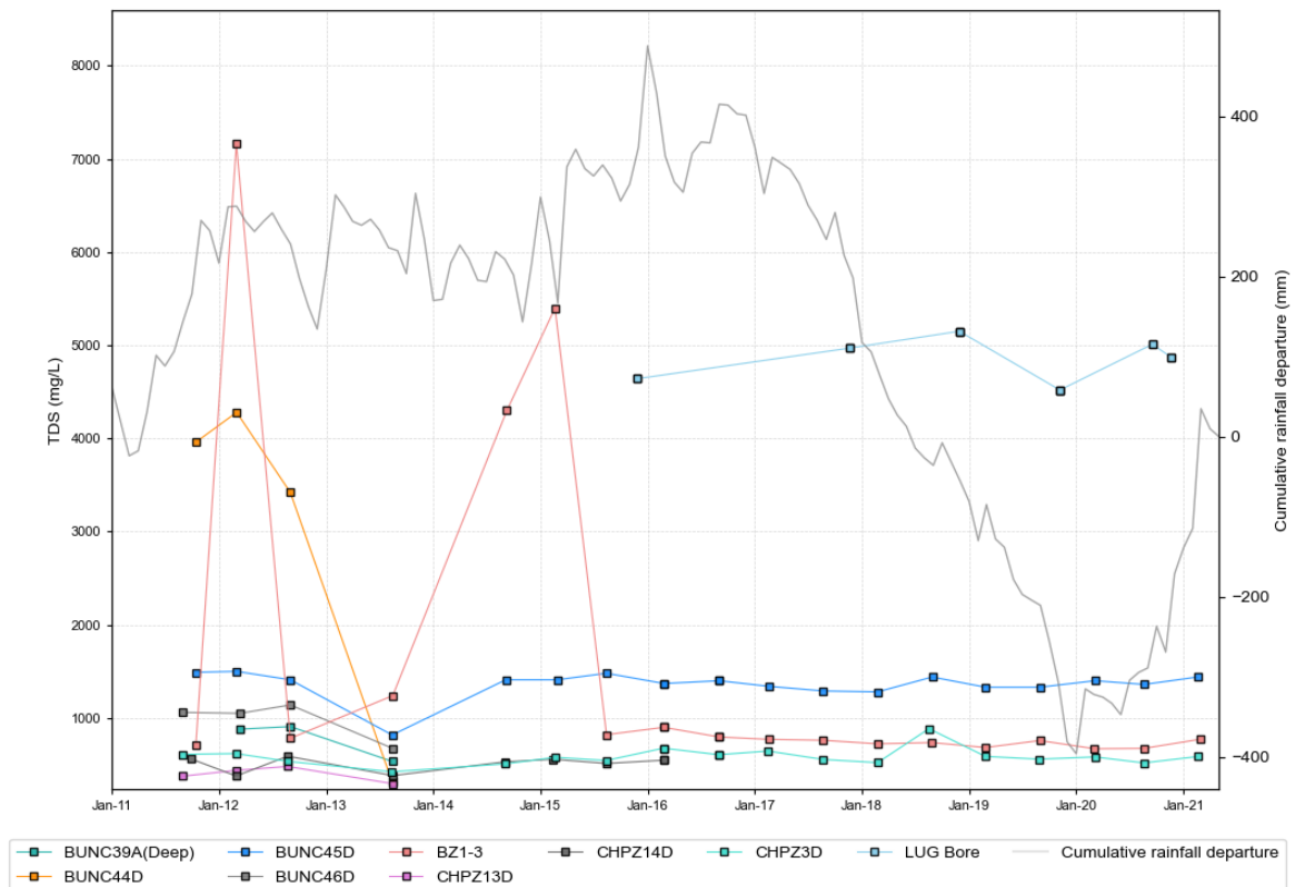
Figure 5.42 Mount Arthur coal seam TDS concentrations
