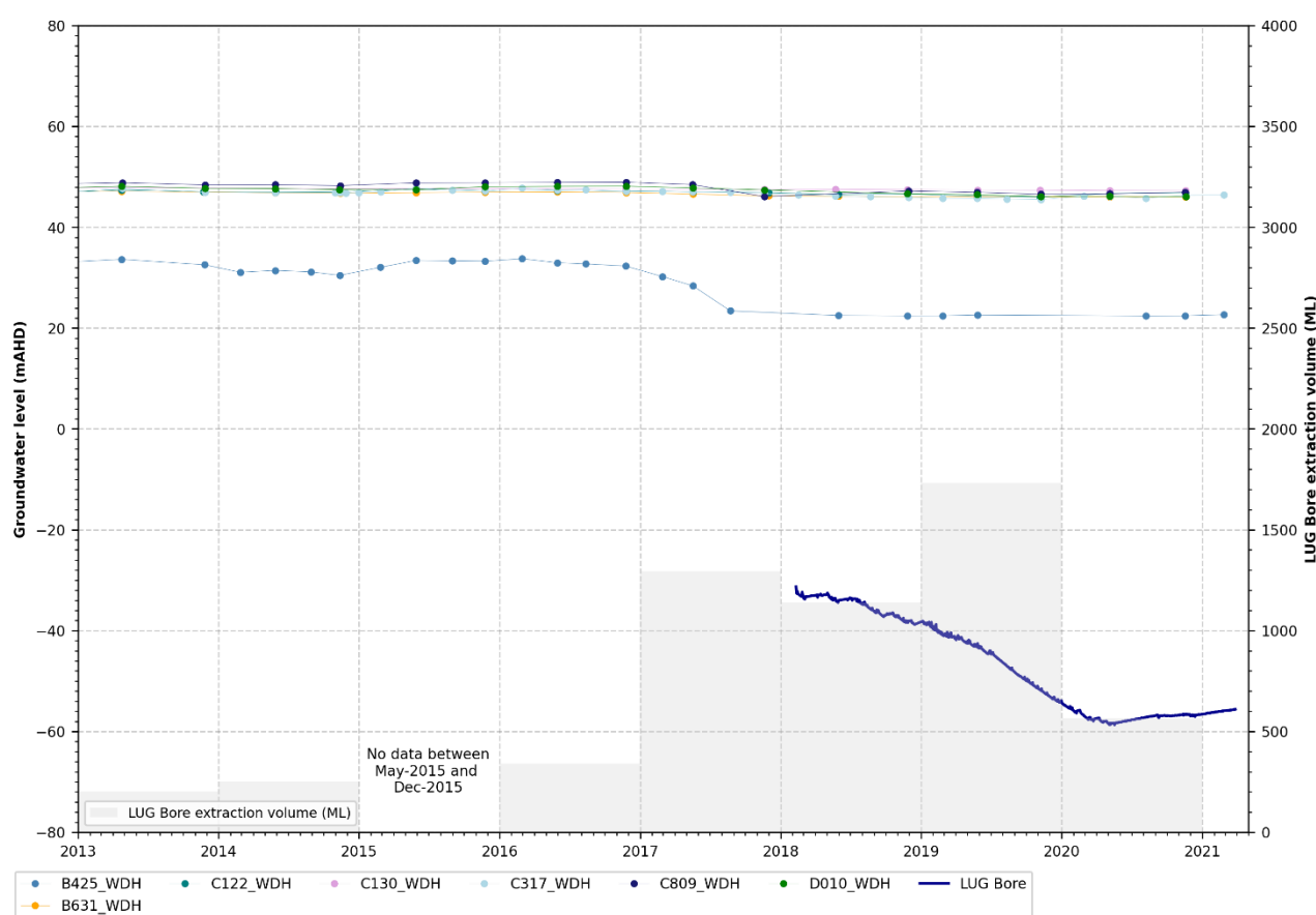
Figure 5.15 Groundwater levels Woodlands Hill coal seam
