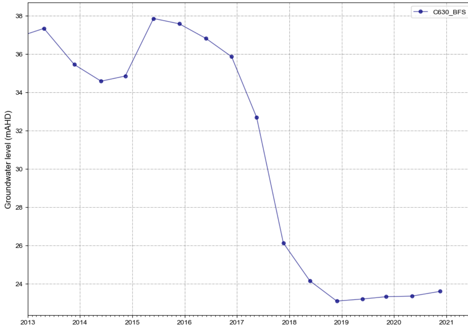
Figure A 24 C630_BFS water levels
