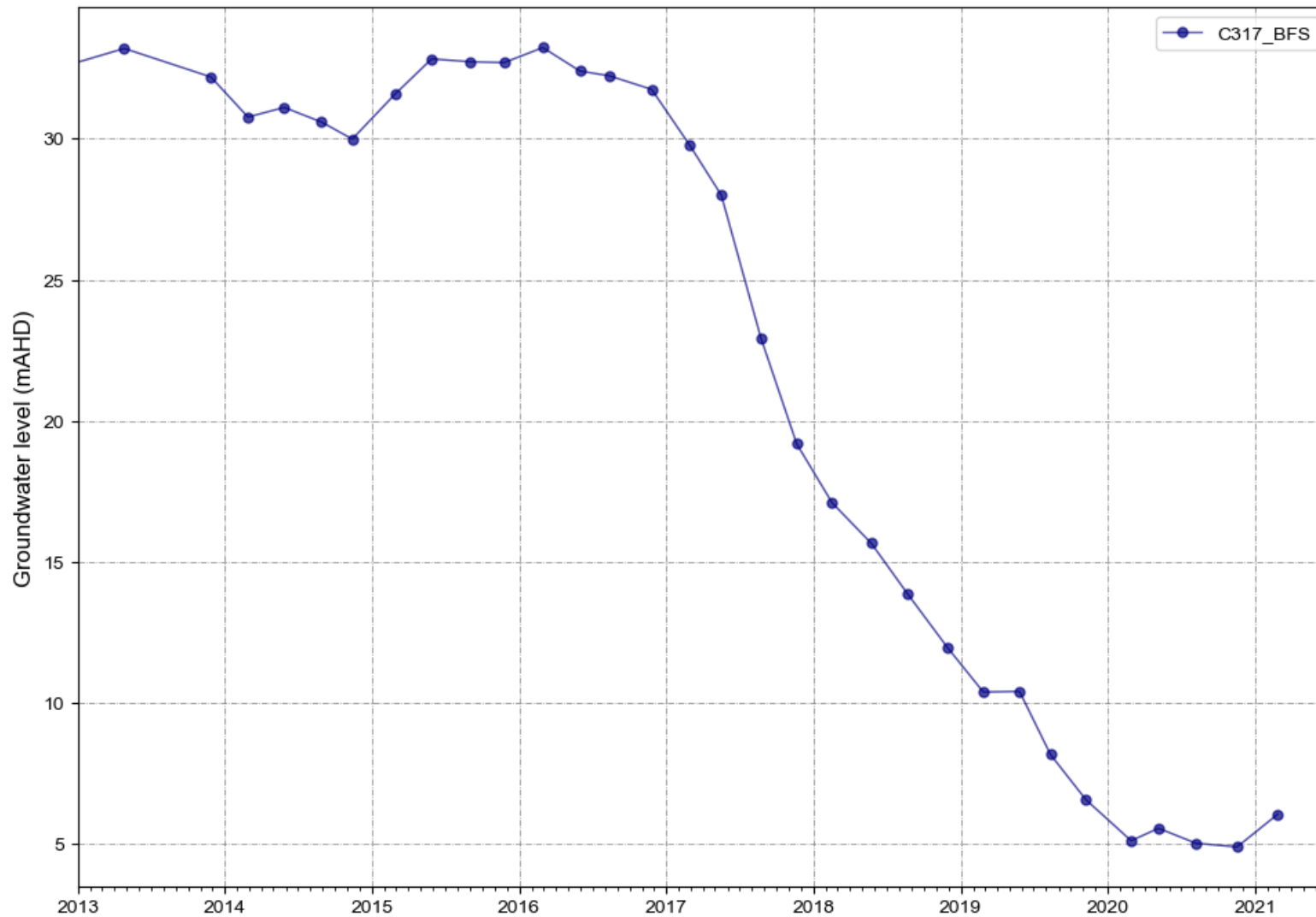
Figure A 21 C317_BFS water levels
