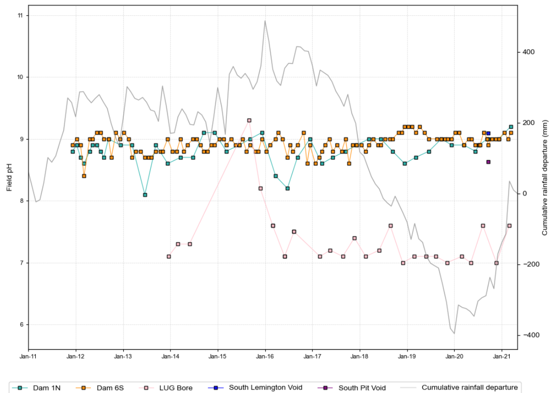
Figure 5.37 MTW main surface water stores and LUG Bore, pH time series data
