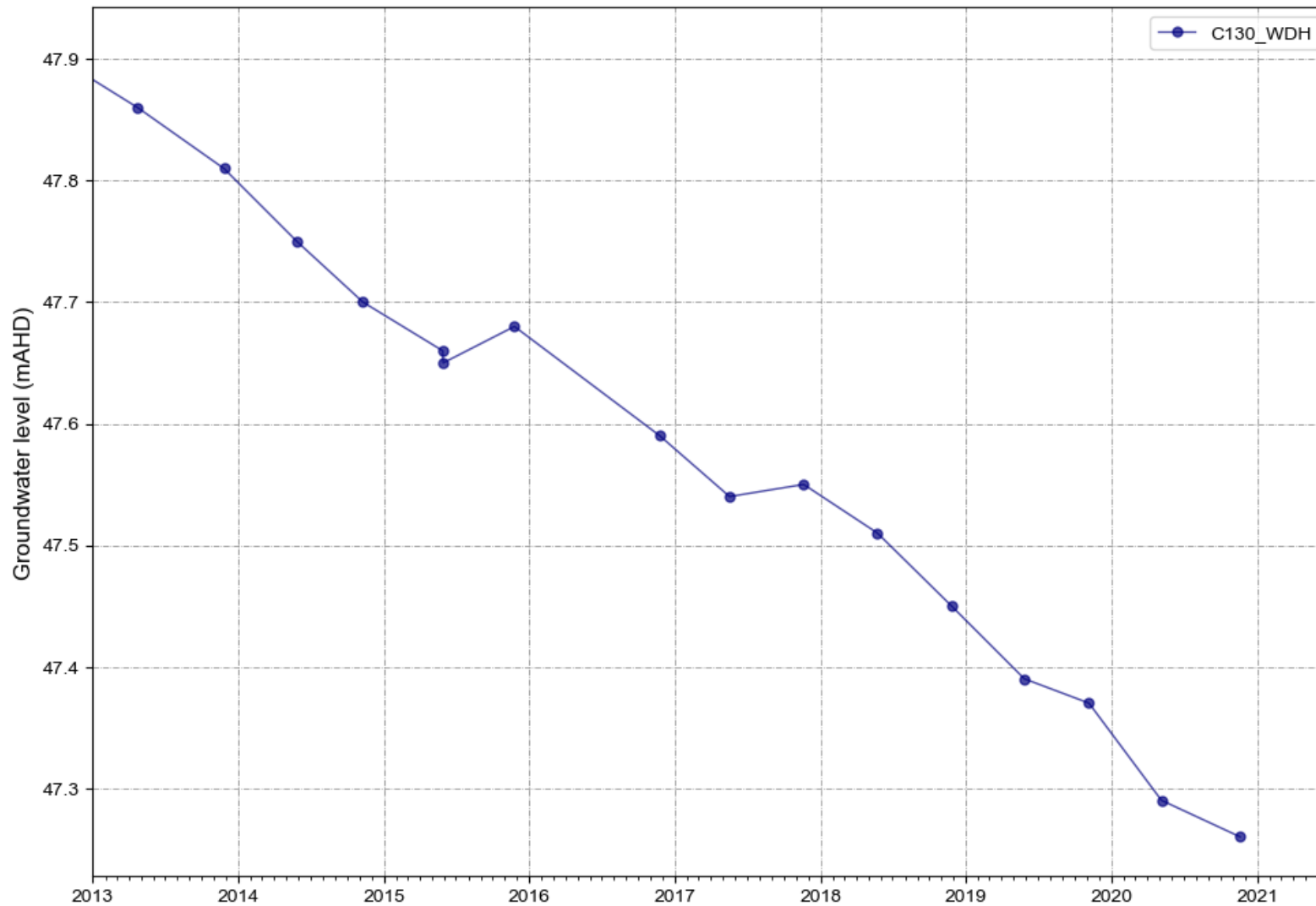
Figure A 40 C130_WDH water levels
