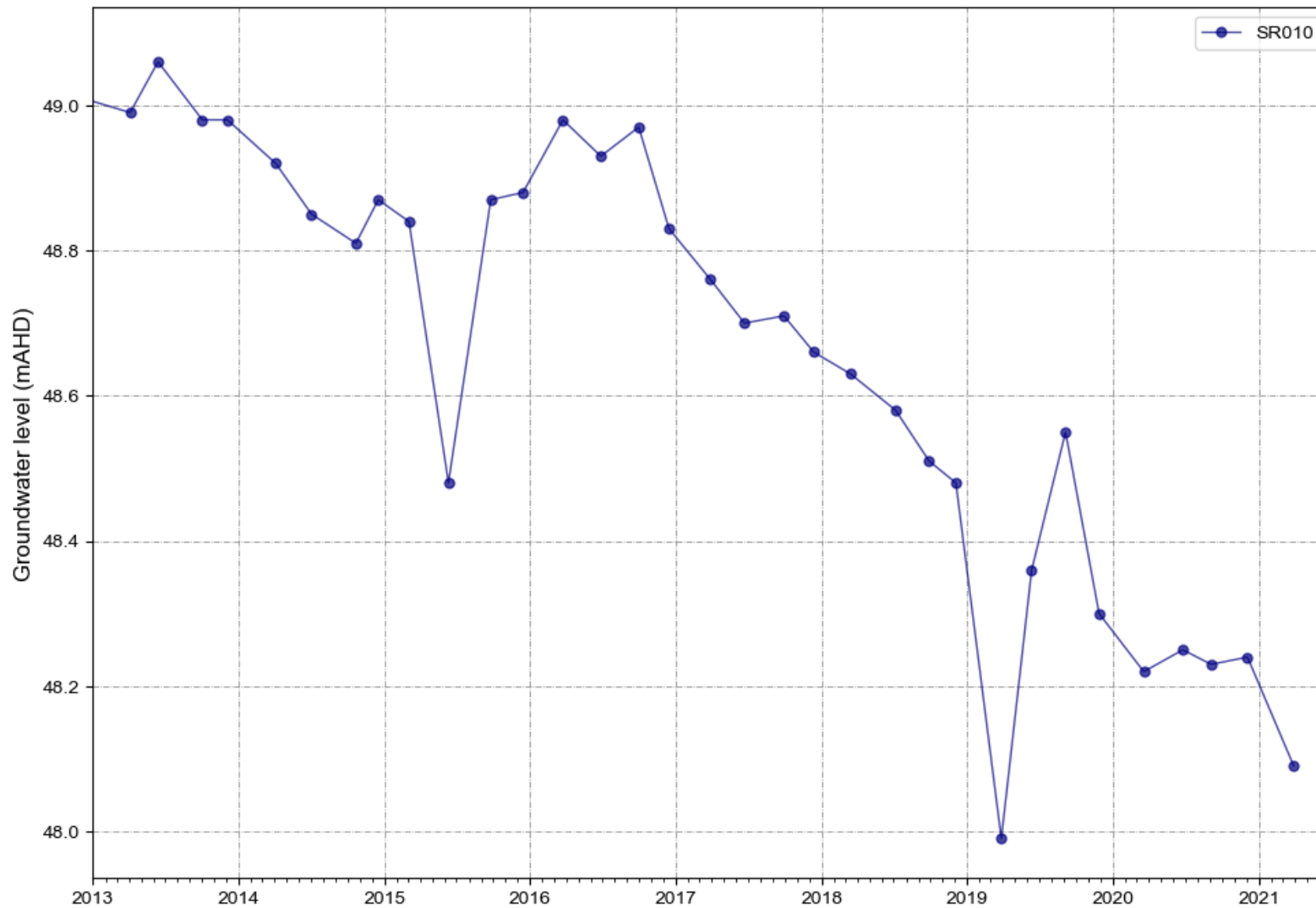
Figure A 13 SR010 water levels
