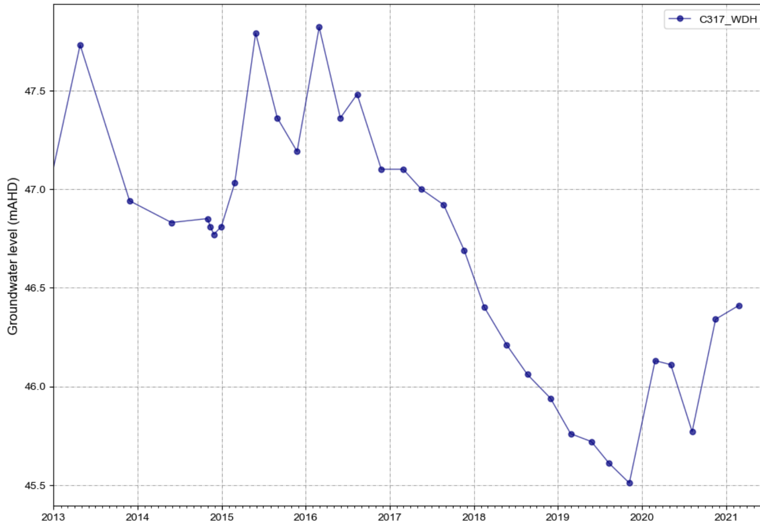
Figure A 41 C317_WDH water levels
