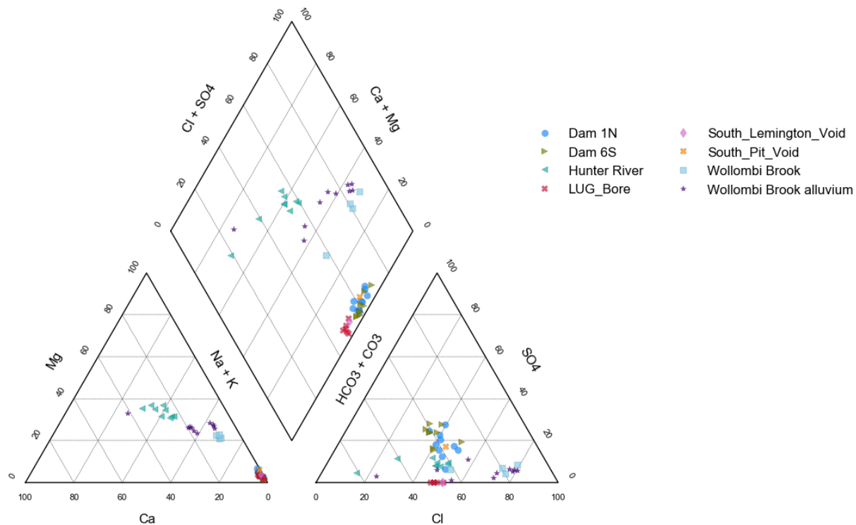
Figure 5.38 MTW main surface water stores, LUG Bore, surface drainages, and alluvium – Piper plot
