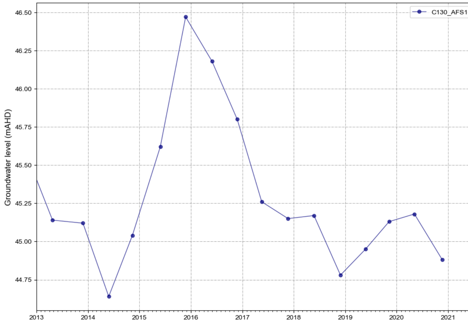
Figure A 32 C130_AFS water levels
