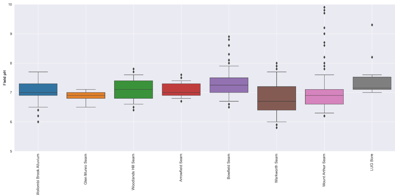
Figure 5.46 Box and whisker plot of pH for coal seams with data above Mount Arthur coal seam
