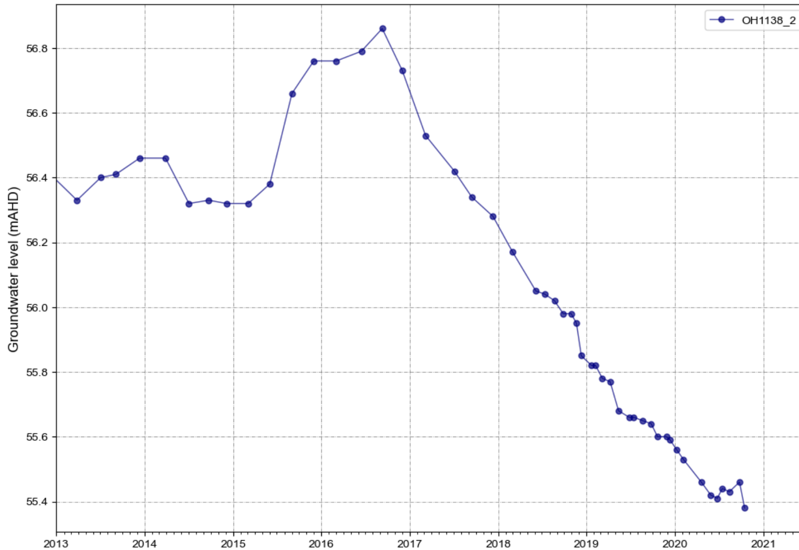
Figure A 15 OH1138_2 water levels
