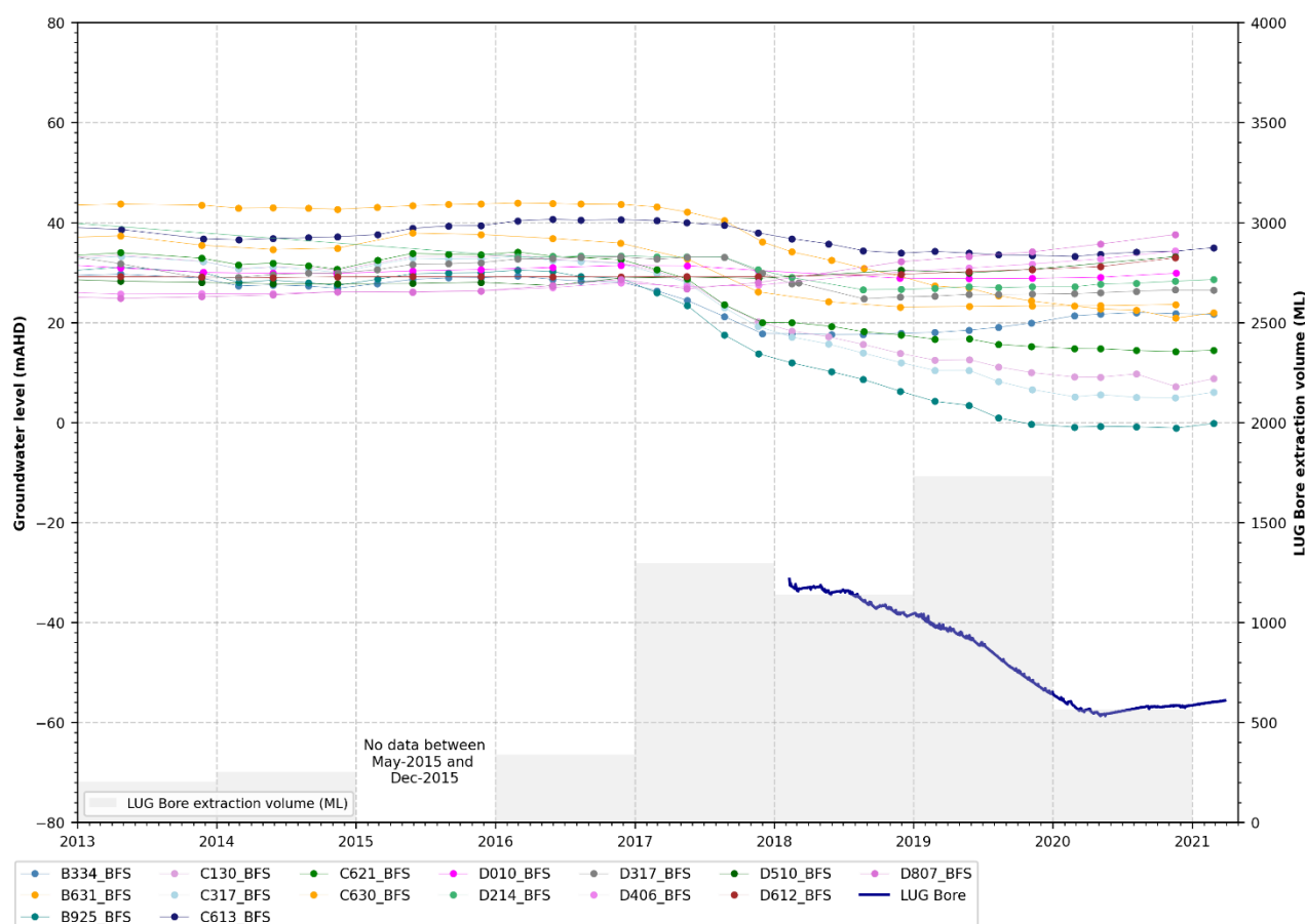
Figure 5.11 Groundwater levels Bowfield coal seam
