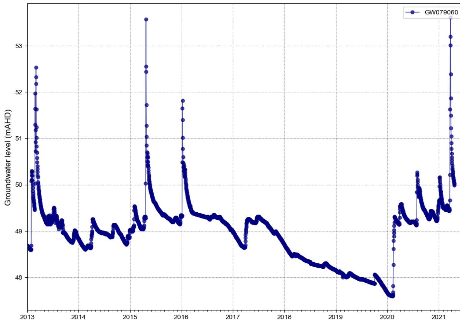
Figure A 48 GW079060 water levels
