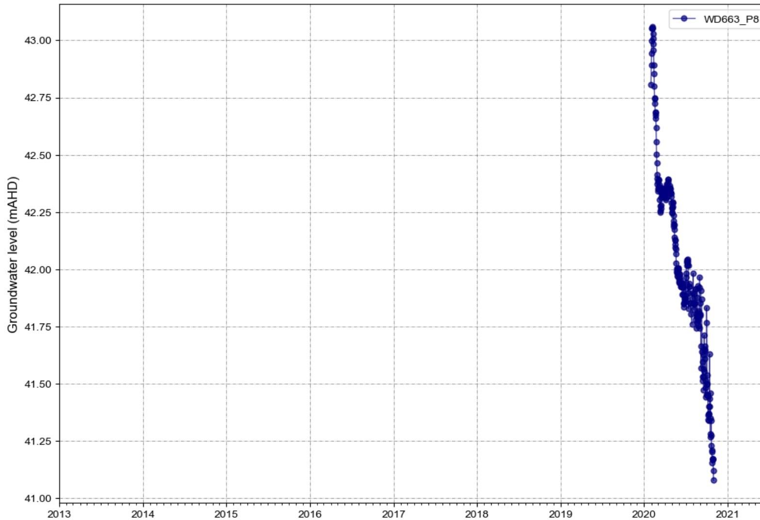
Figure A 16 WD663_P8 water levels
