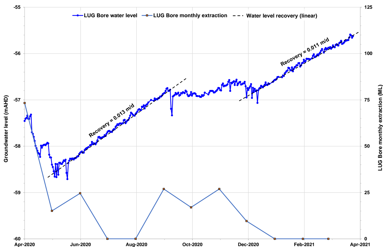
Figure 5.29 Estimated inflow- and recovery rates at the LUG Bore
