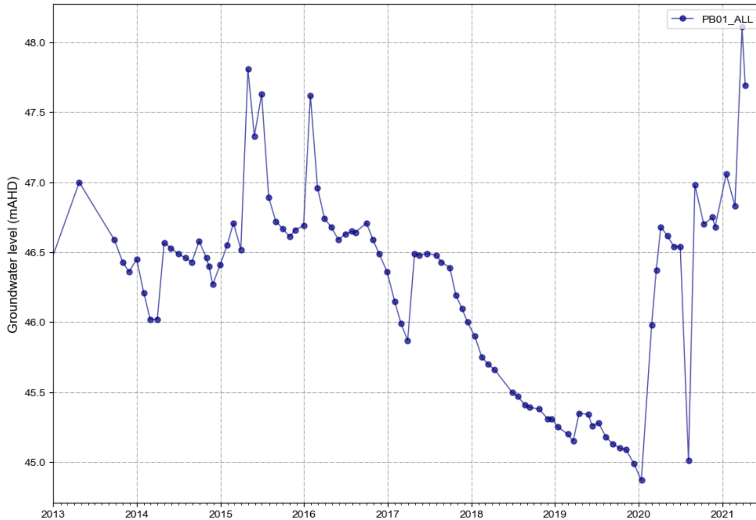
Figure A 51 PB01_ALL water levels
