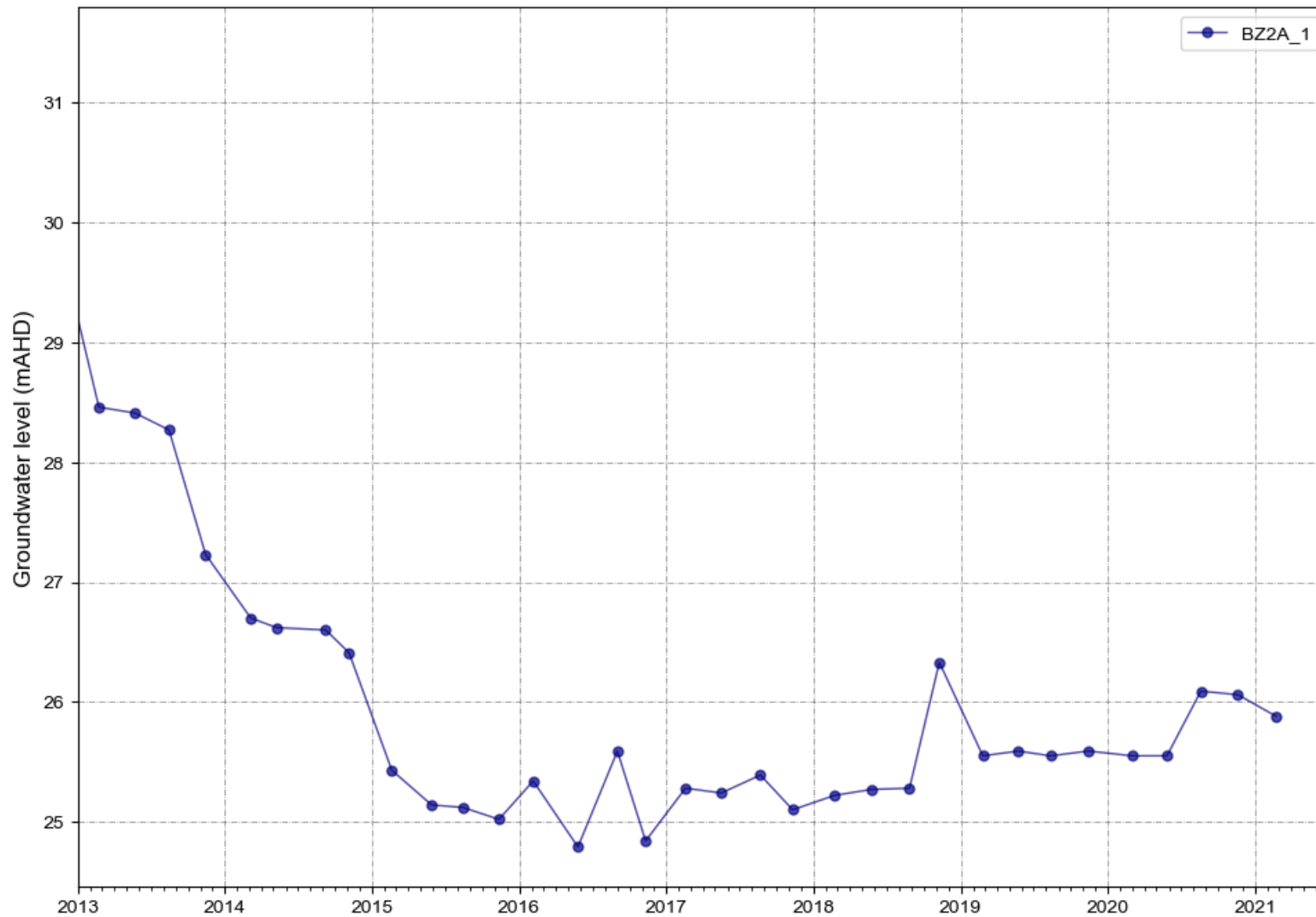
Figure A 8 BZ2A_1 water levels
