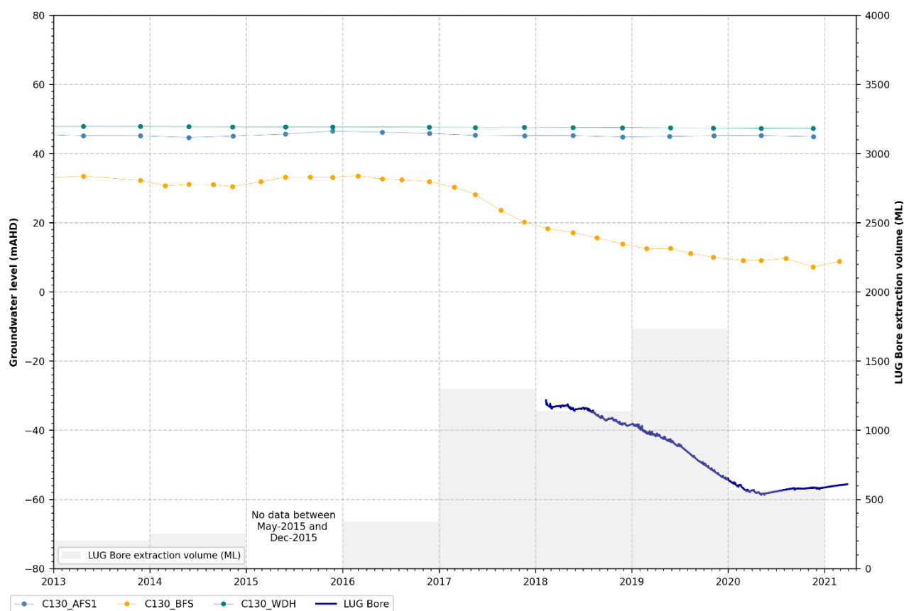
Figure 5.24 C130 nested facility water levels
