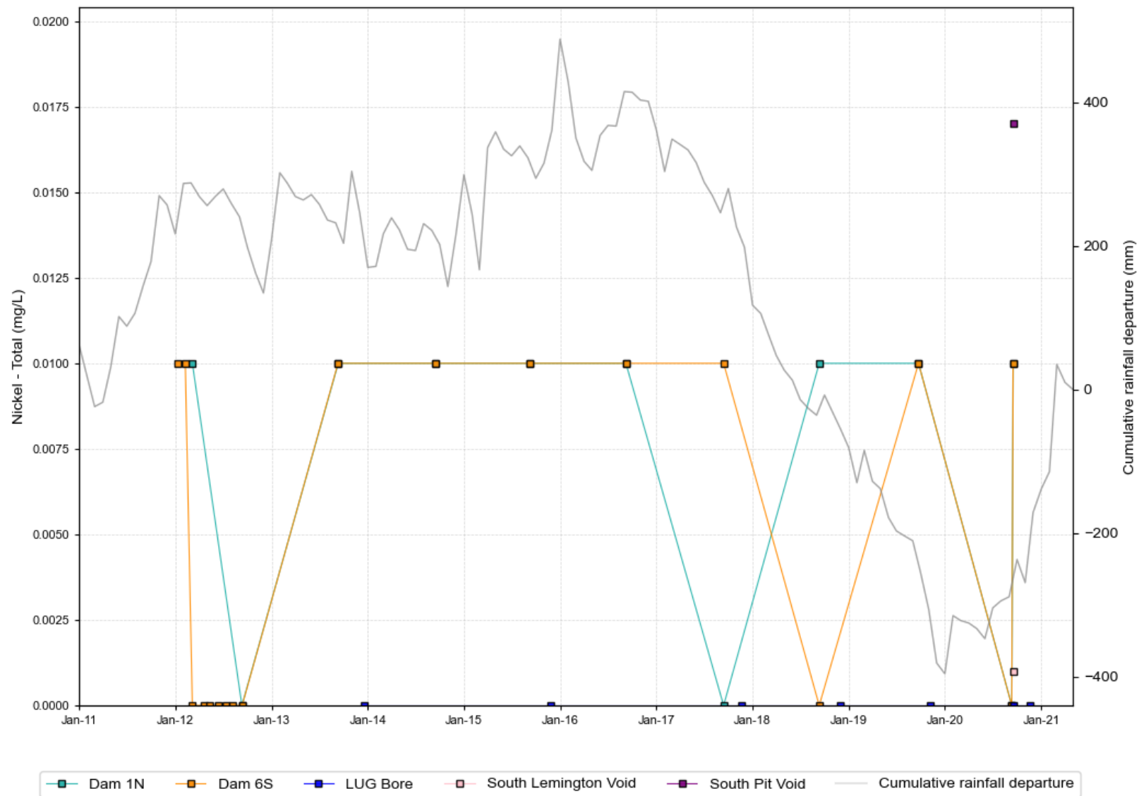
Figure B 9 MTW main surface water stores and LUG Bore, nickel time series data
