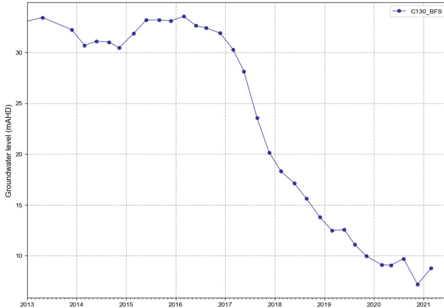
Figure A 20 C130_BFS water levels
