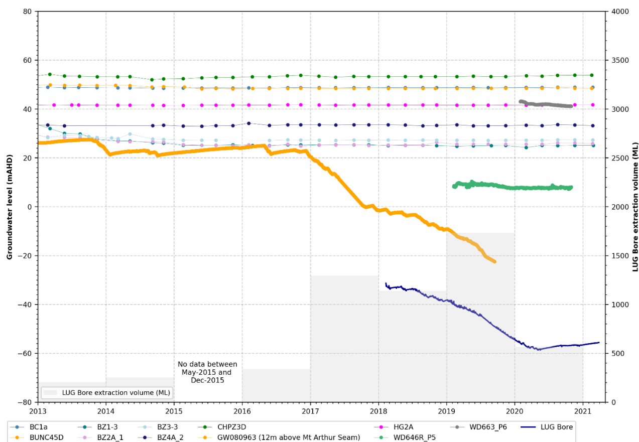
Figure 5.3 Mount Arthur coal seam groundwater levels
