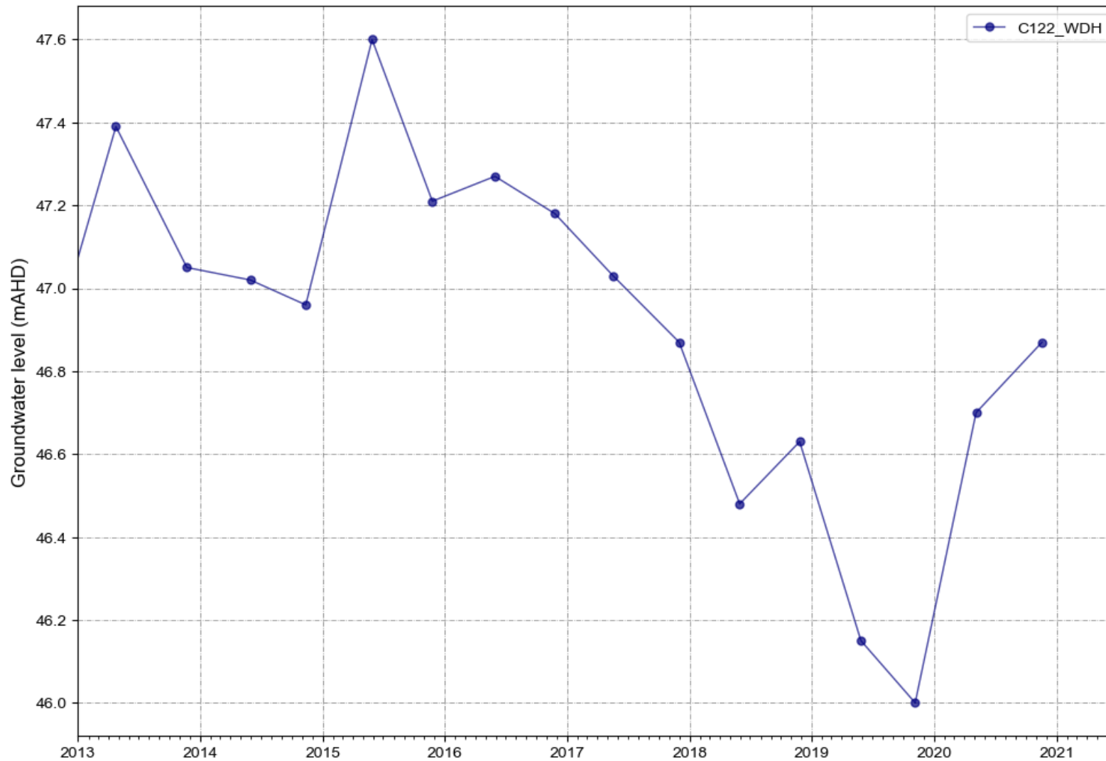
Figure A 39 C122_WDH water levels
