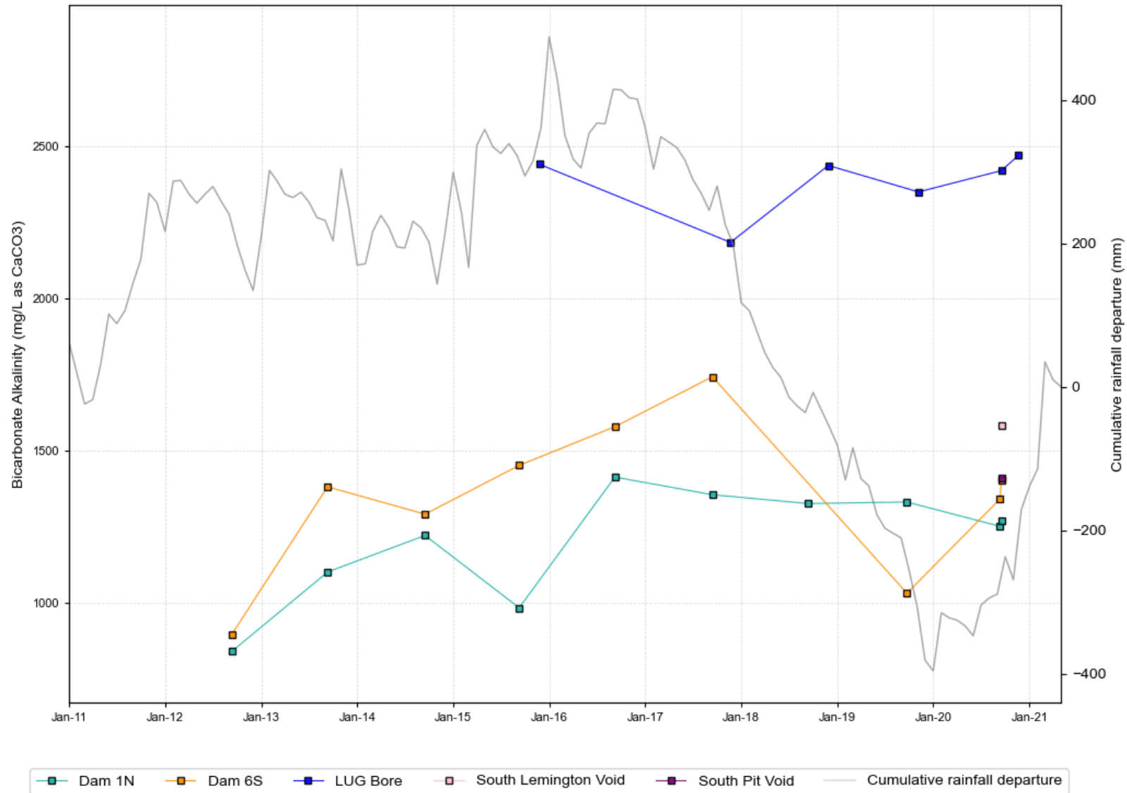
Figure B 3 MTW main surface water stores and LUG Bore, bicarbonate alkalinity time series data
