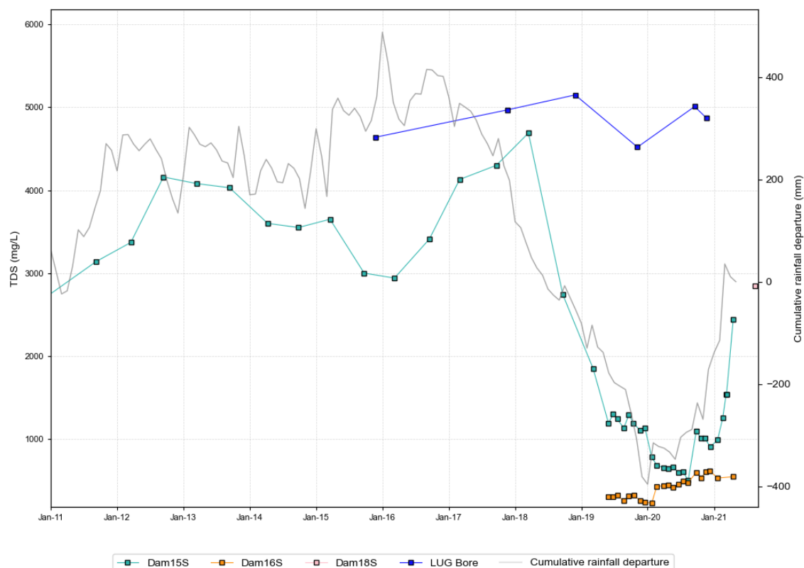
Figure 5.31 HVO main surface water stores and LUG Bore, TDS time series data
