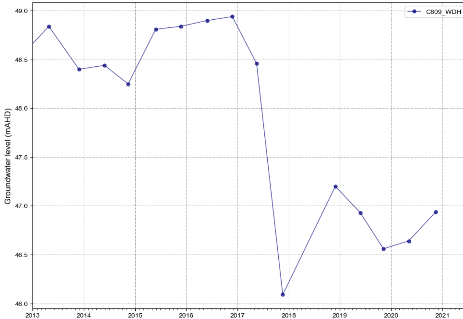
Figure A 42 C809_WDH water levels
