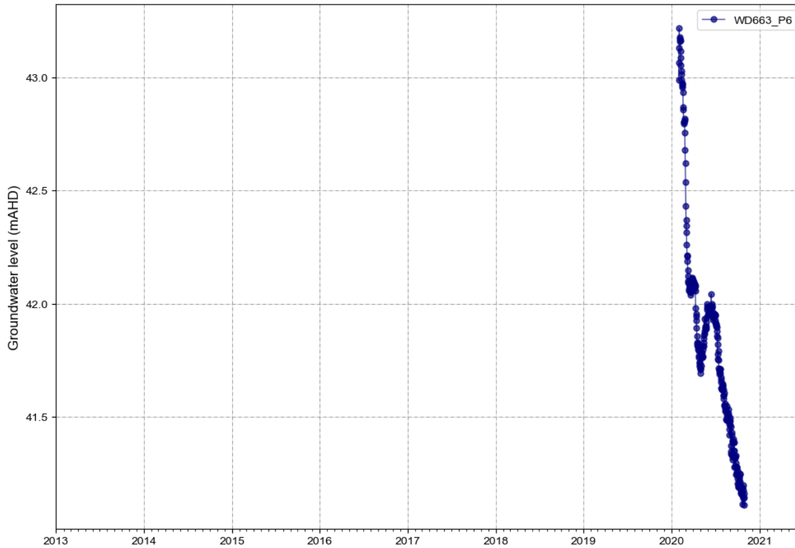
Figure A 4 WD663_P6 water levels
