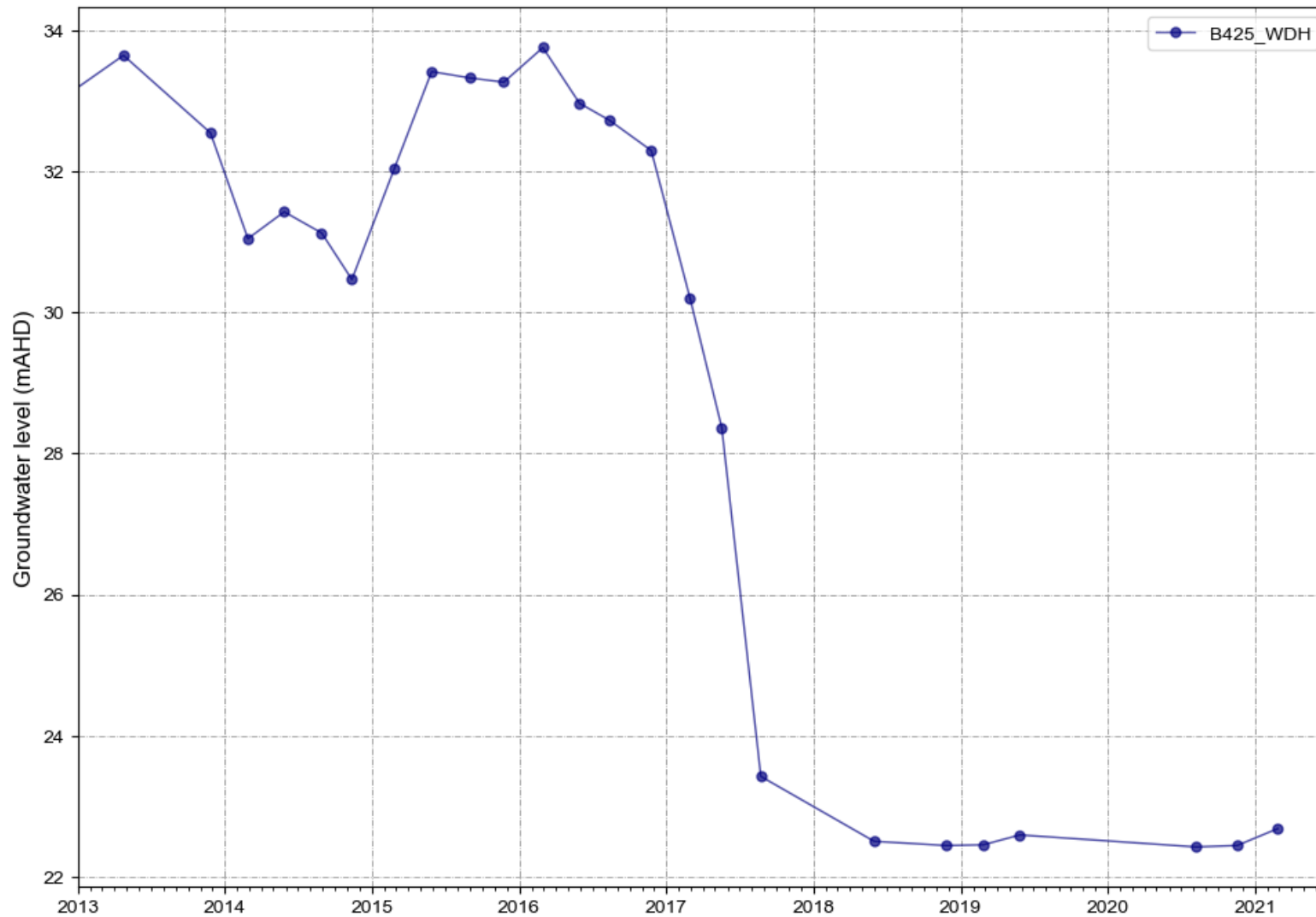
Figure A 37 B425_WDH water levels
