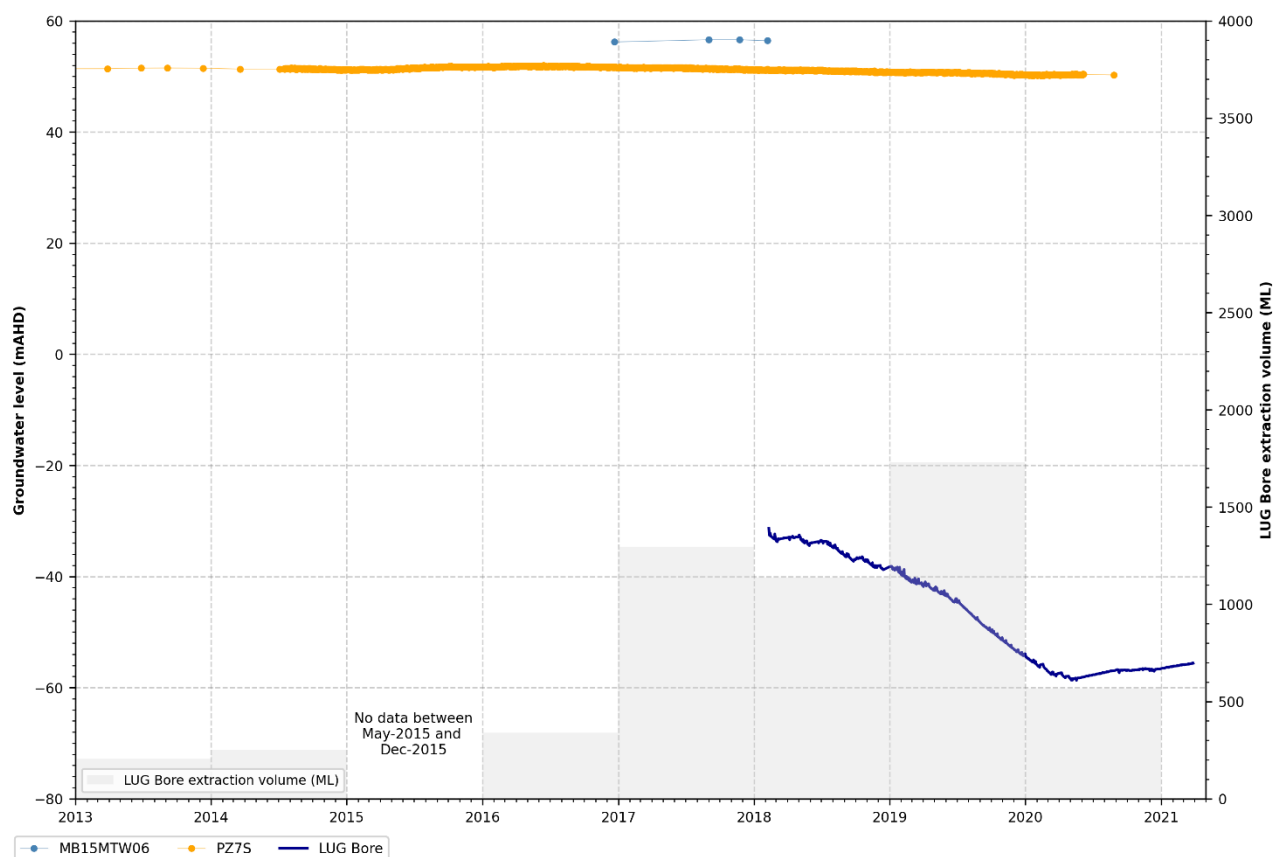
Figure 5.22 Groundwater levels Warkworth Sands
