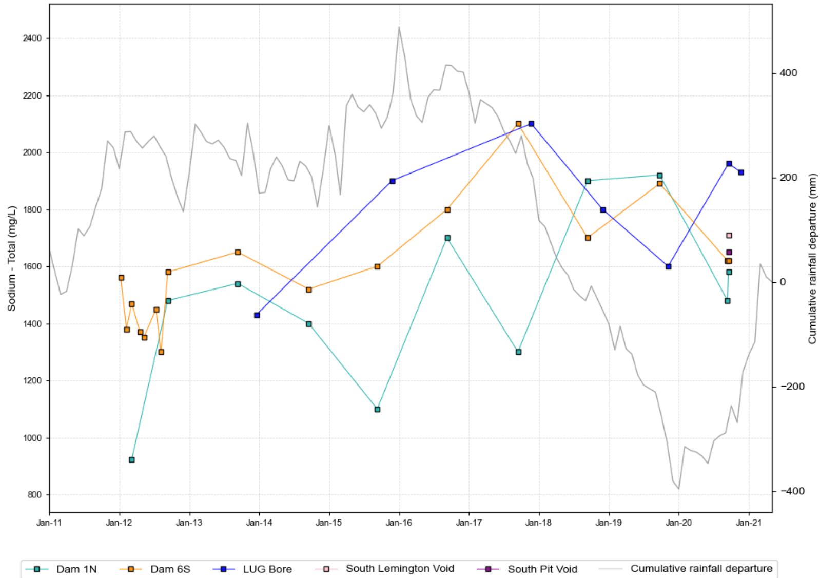
Figure B 11 MTW main surface water stores and LUG Bore, sodium time series data
