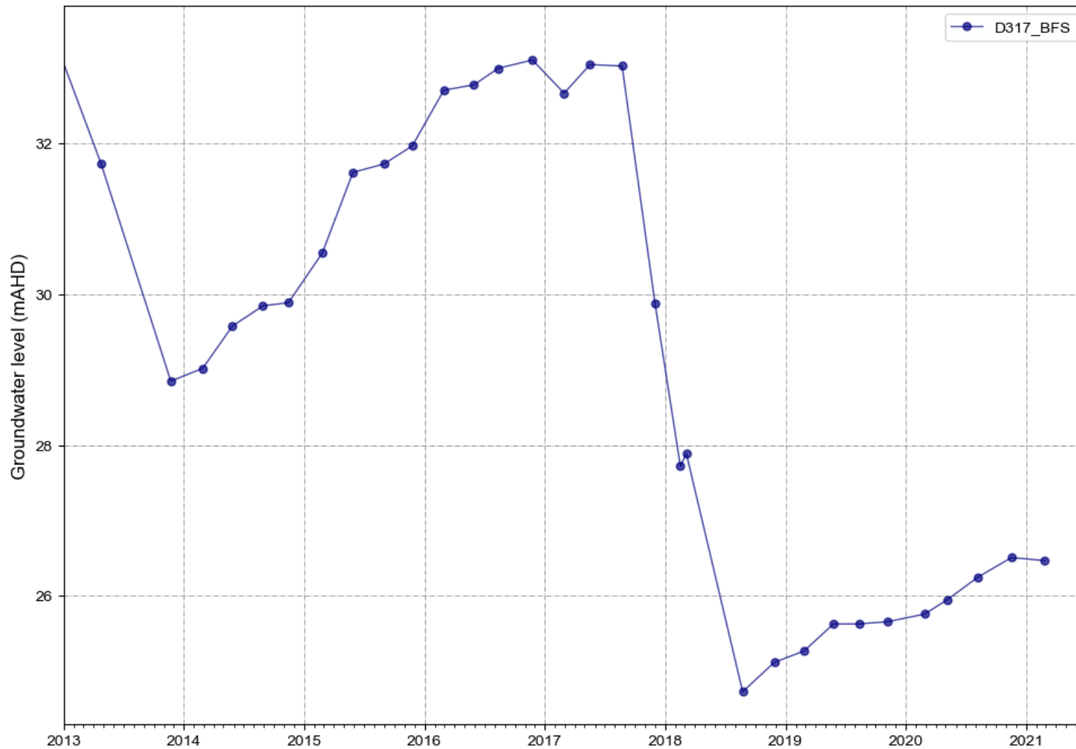
Figure A 27 D317_BFS
