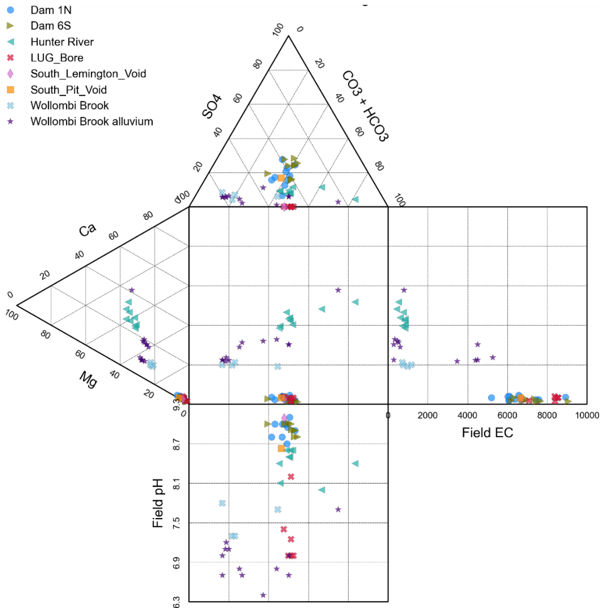
Figure 5.39 MTW main surface water stores, LUG Bore, surface drainages, and alluvium – Durov plot
