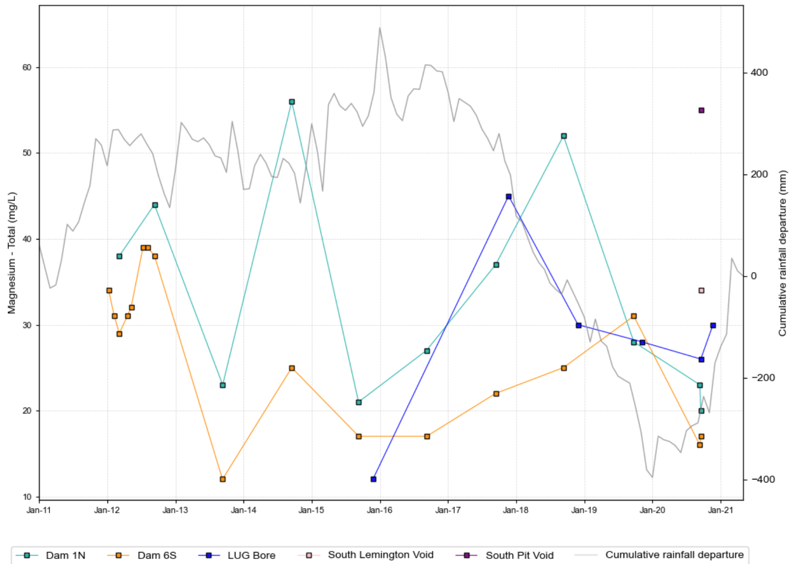
Figure B 8 MTW main surface water stores and LUG Bore, magnesium time series data
