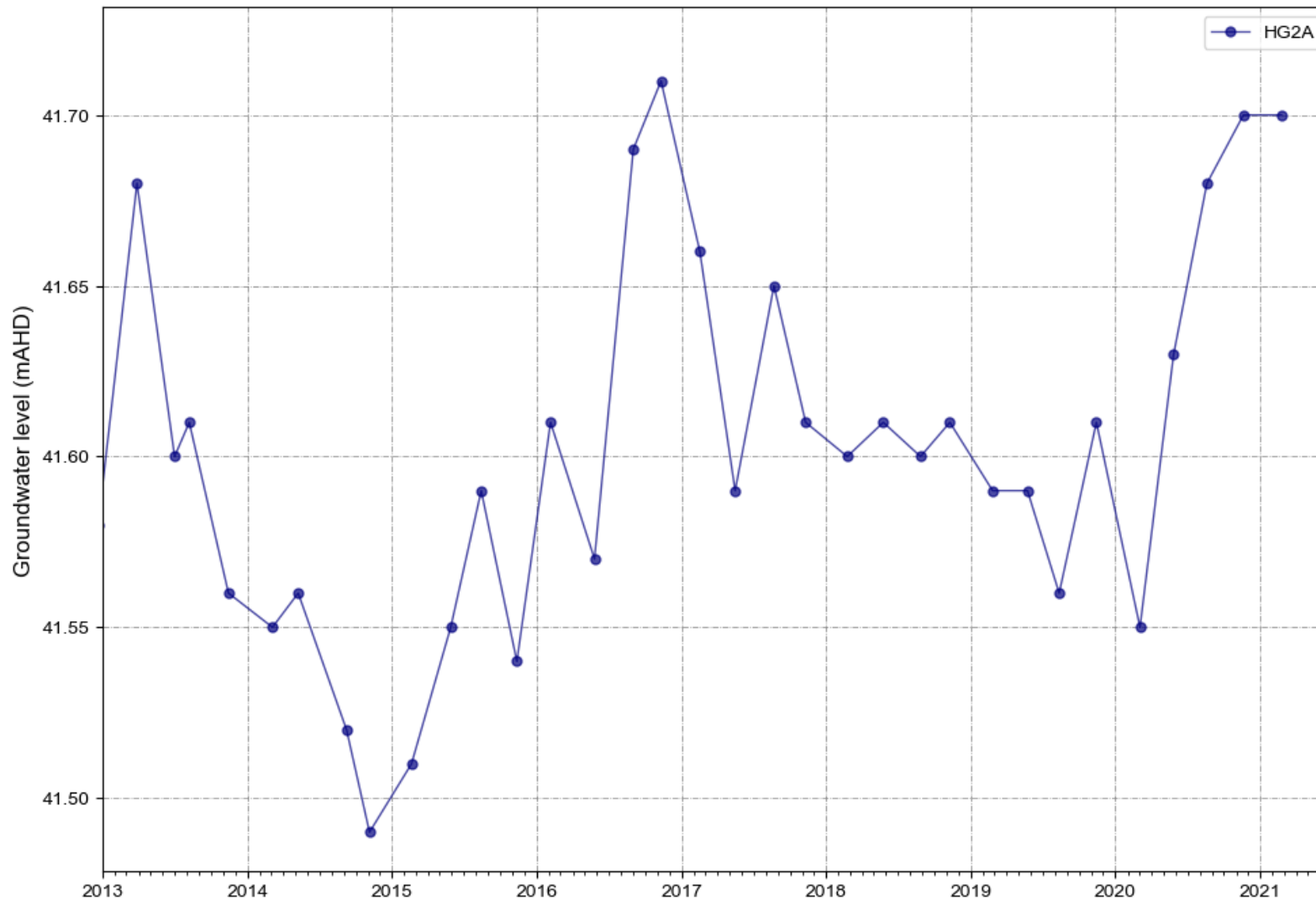
Figure A 12 HG2A water levels
