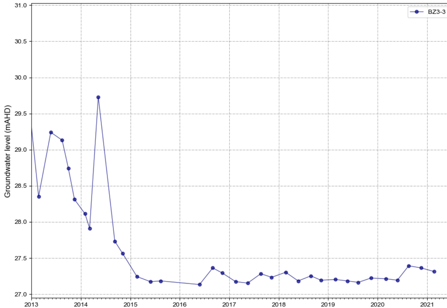
Figure A 9 BZ3-3 water levels
