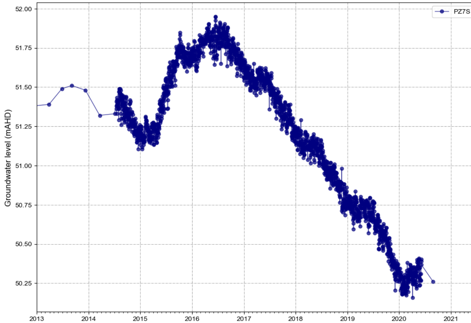
Figure A 53 PZ7S water levels
