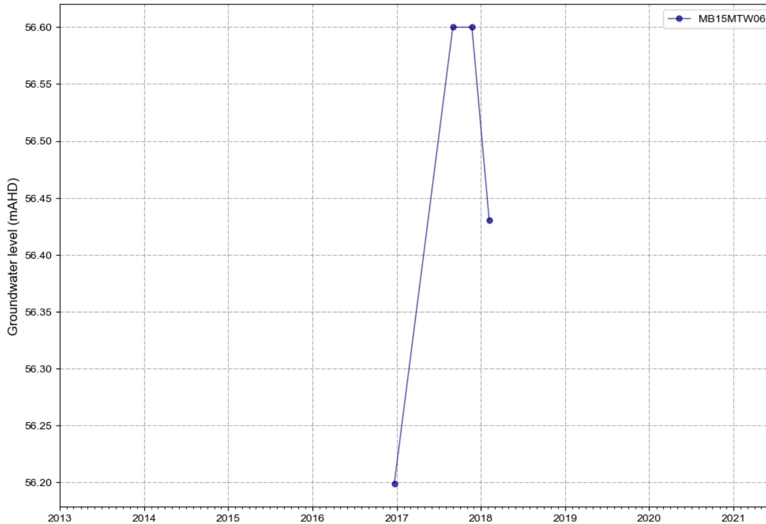
Figure A 52 MB15MTW06 water levels
