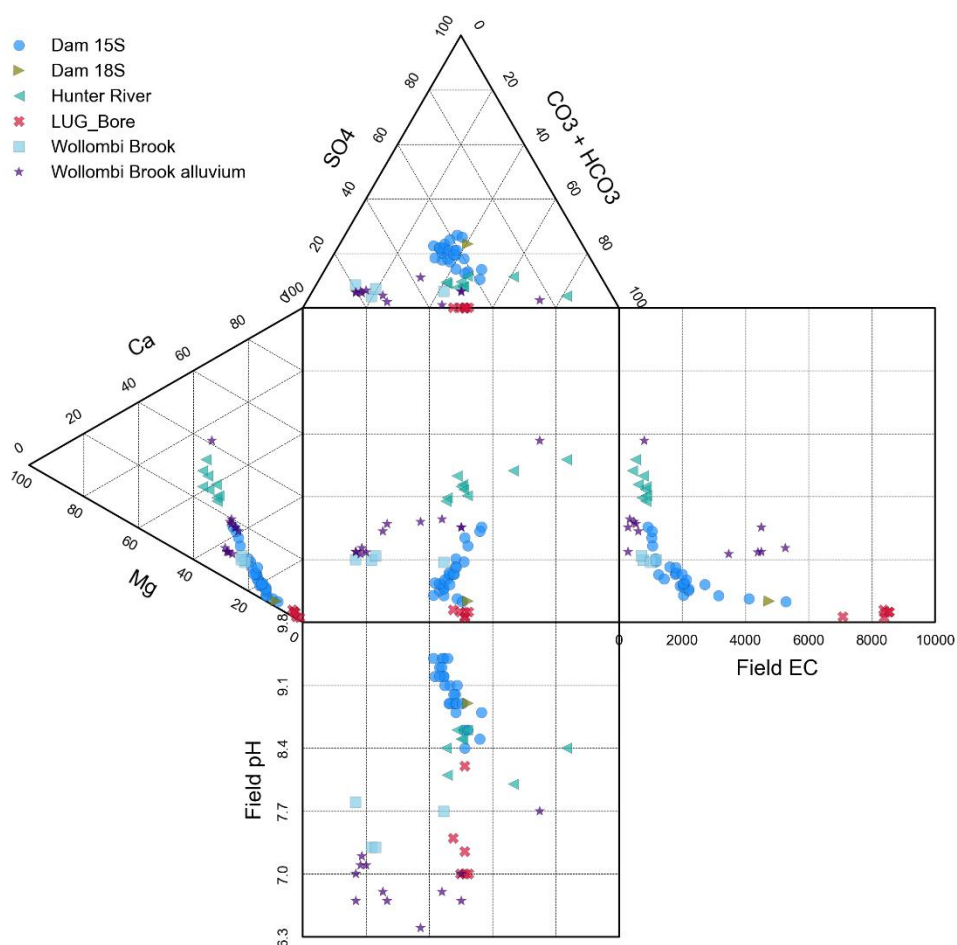
Figure 5.34 MTW main surface water stores, LUG Bore, surface water courses, and alluvium – Durov plot
