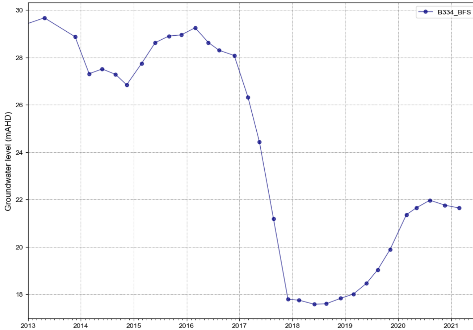
Figure A 17 B334_BFS water levels
