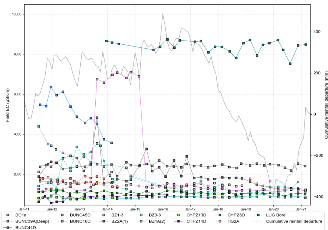
Figure 5.40 Mount Arthur coal seam electrical conductivity
