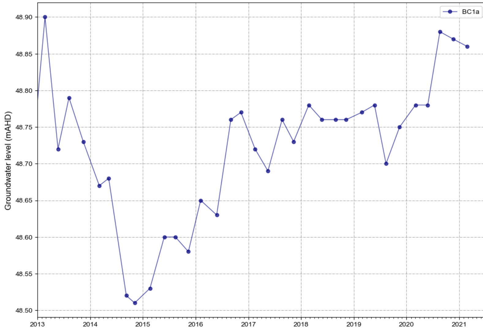
Figure A 5 BC1a water levels
