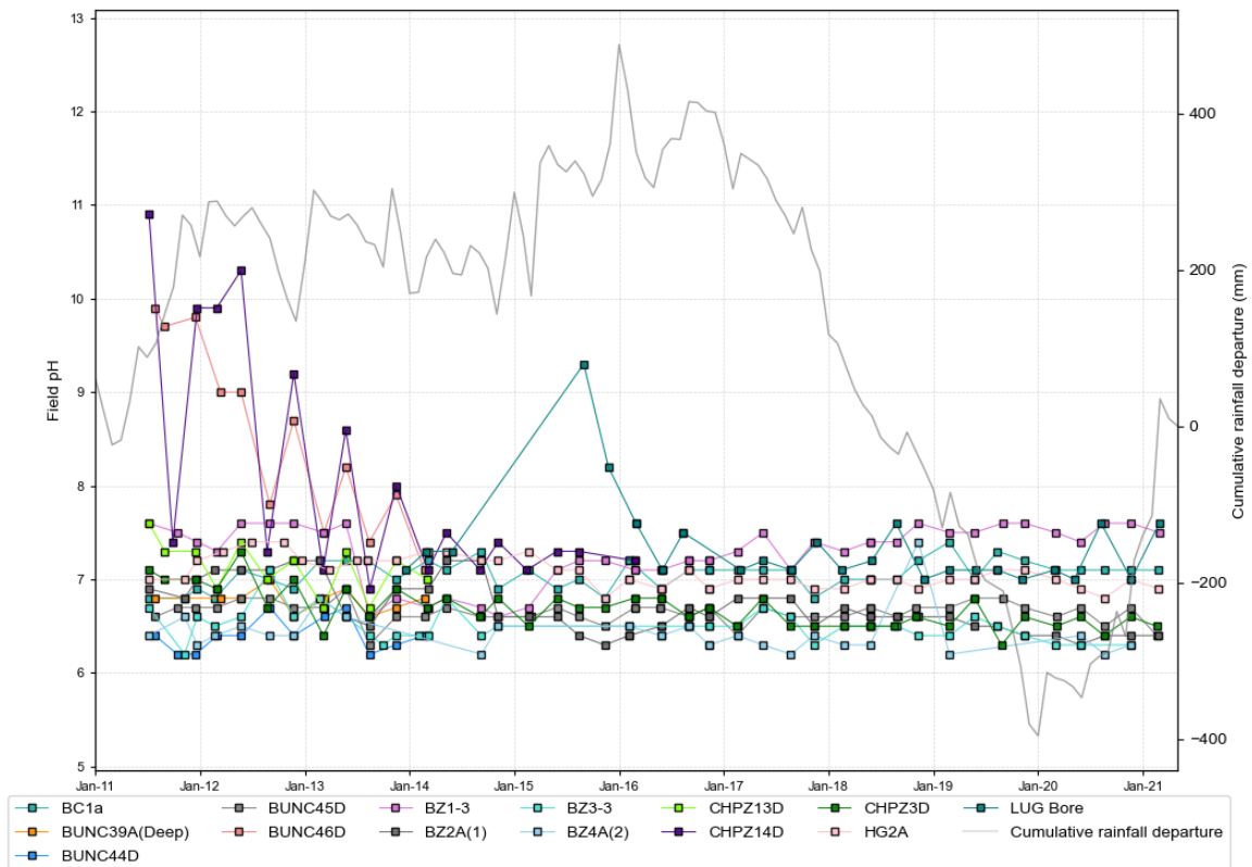
Figure 5.41 Mount Arthur coal seam pH
