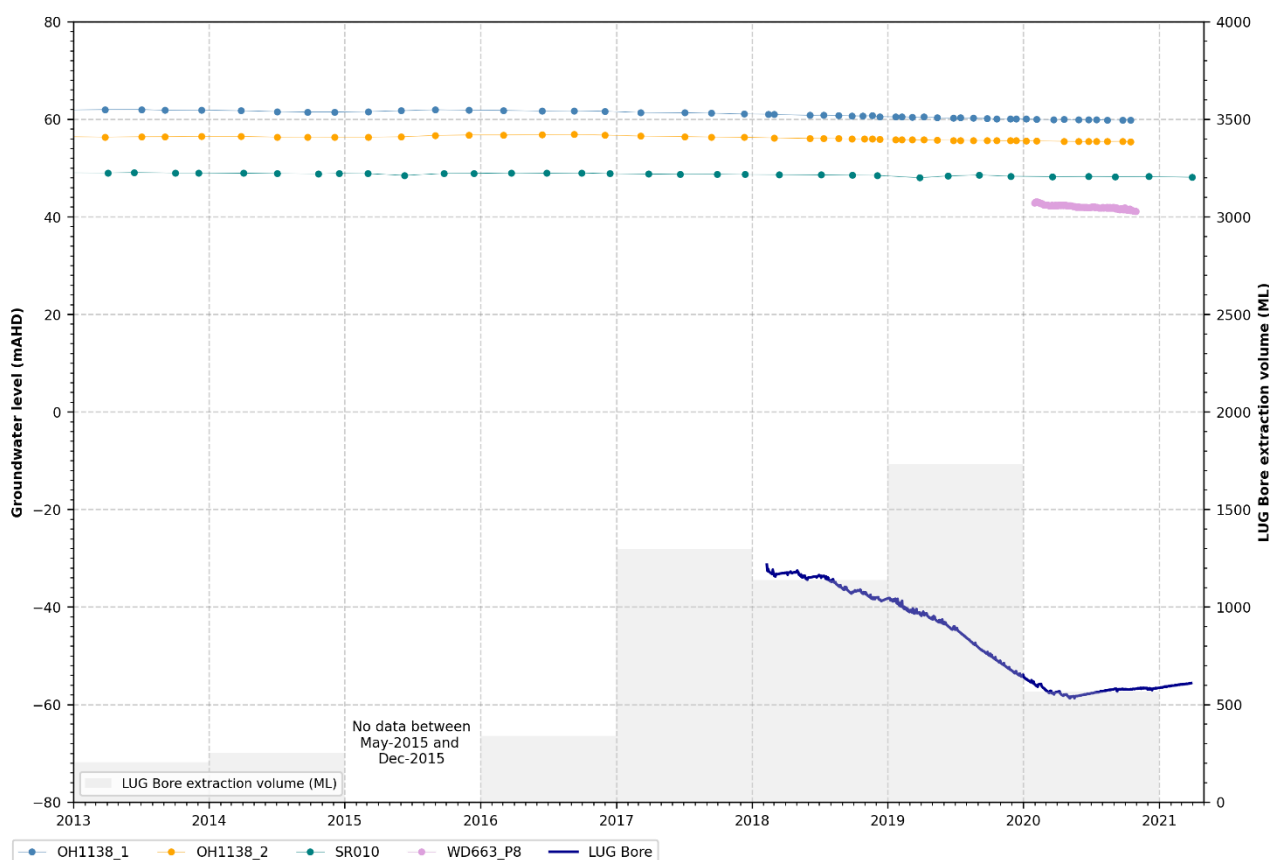
Figure 5.9 Groundwater levels Warkworth coal seam
