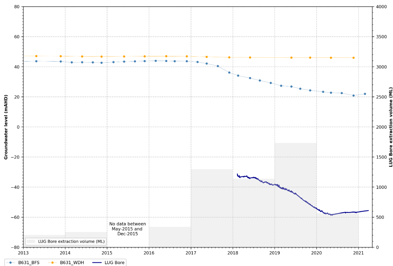
Figure 5.25 B631 nested facility water levels
