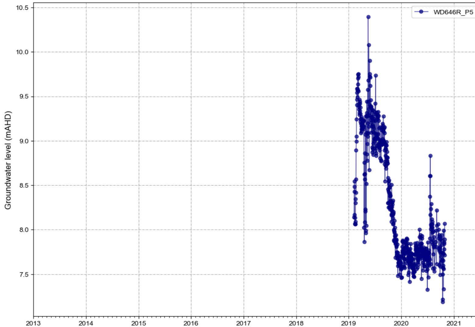
Figure A 3 WD646R_P5 water levels
