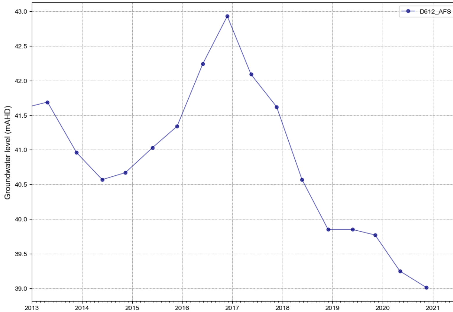
Figure A 35 D612_AFS water levels
