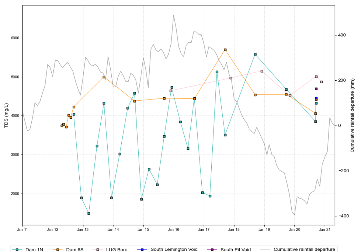
Figure 5.36 MTW main surface water stores and LUG Bore, TDS time series data
