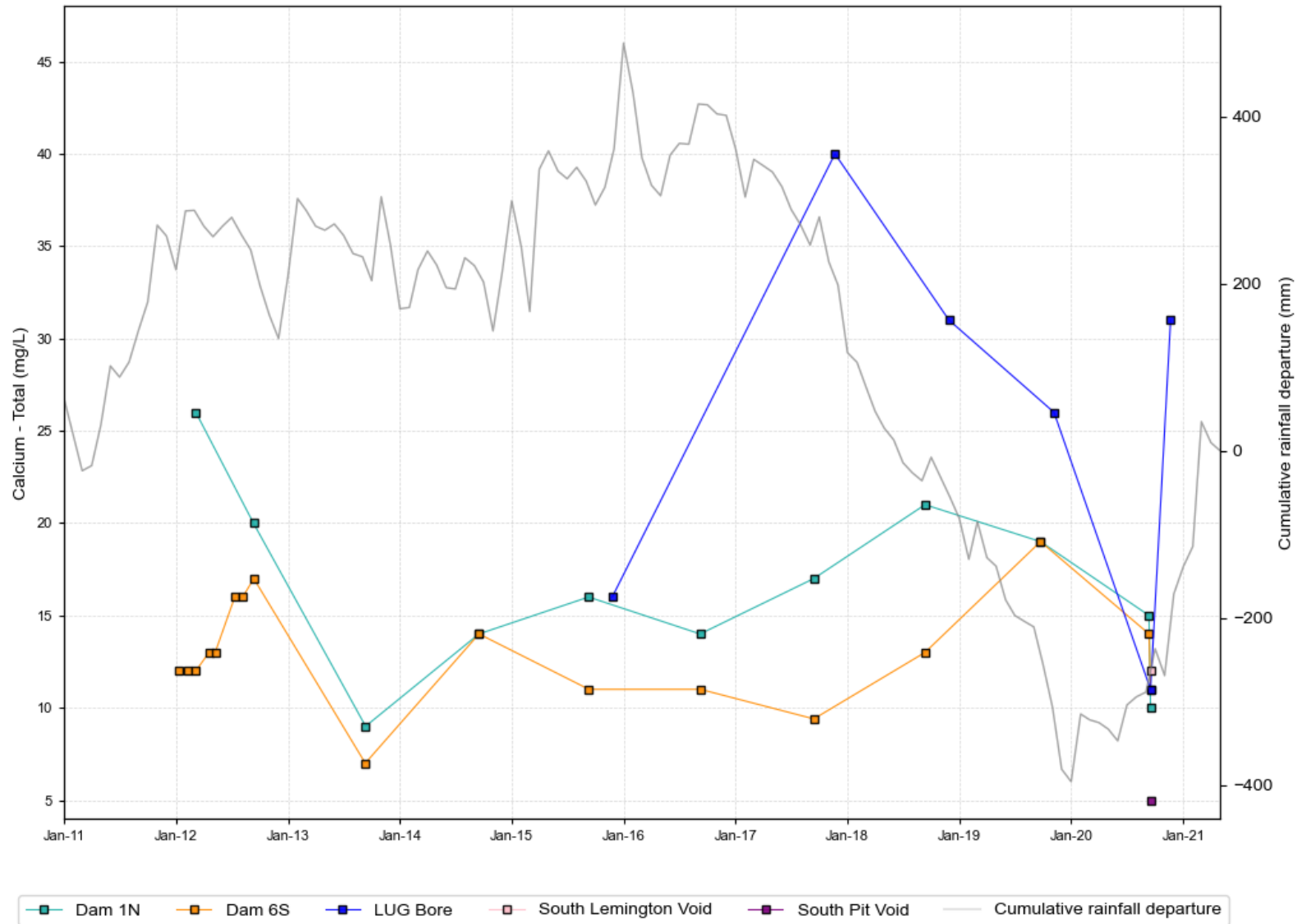
Figure B 4 MTW main surface water stores and LUG Bore, calcium time series data
