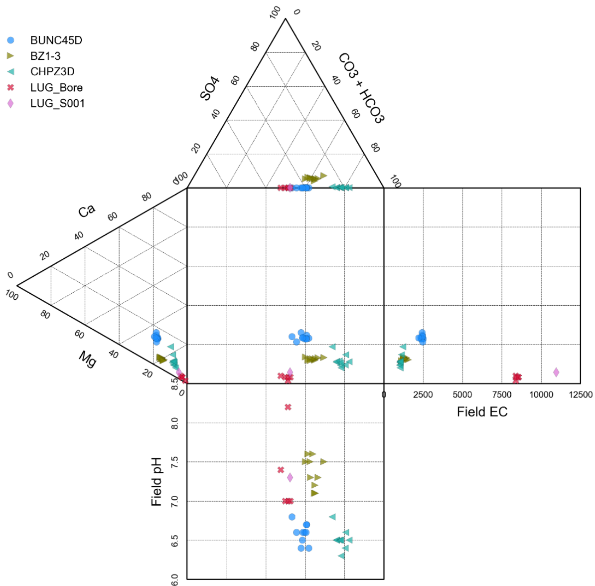
Figure 5.44 Durov plot of the Mount Arthur coal seam
