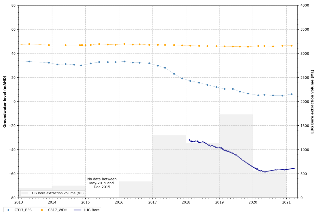
Figure 5.26 C317 nested facility water levels
