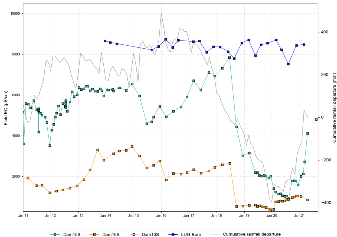
Figure 5.30 HVO main surface water stores and LUG Bore, electrical conductivity time series data
