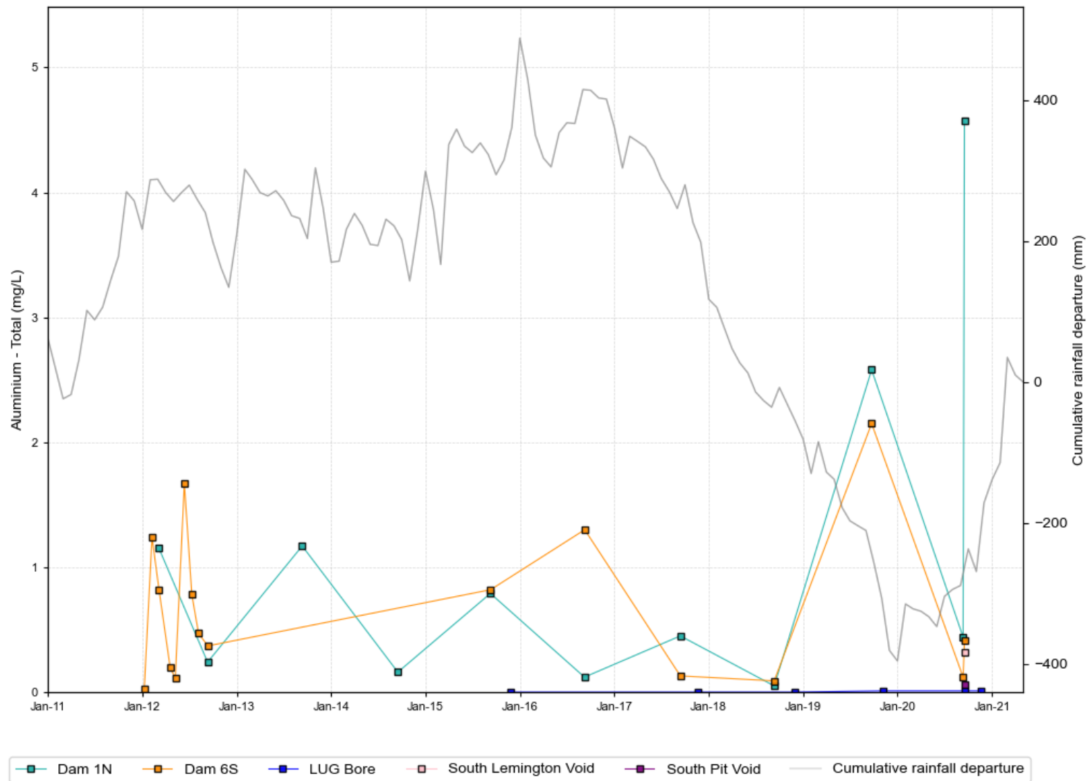
Figure B 1 MTW main surface water stores and LUG Bore, aluminium time series data
