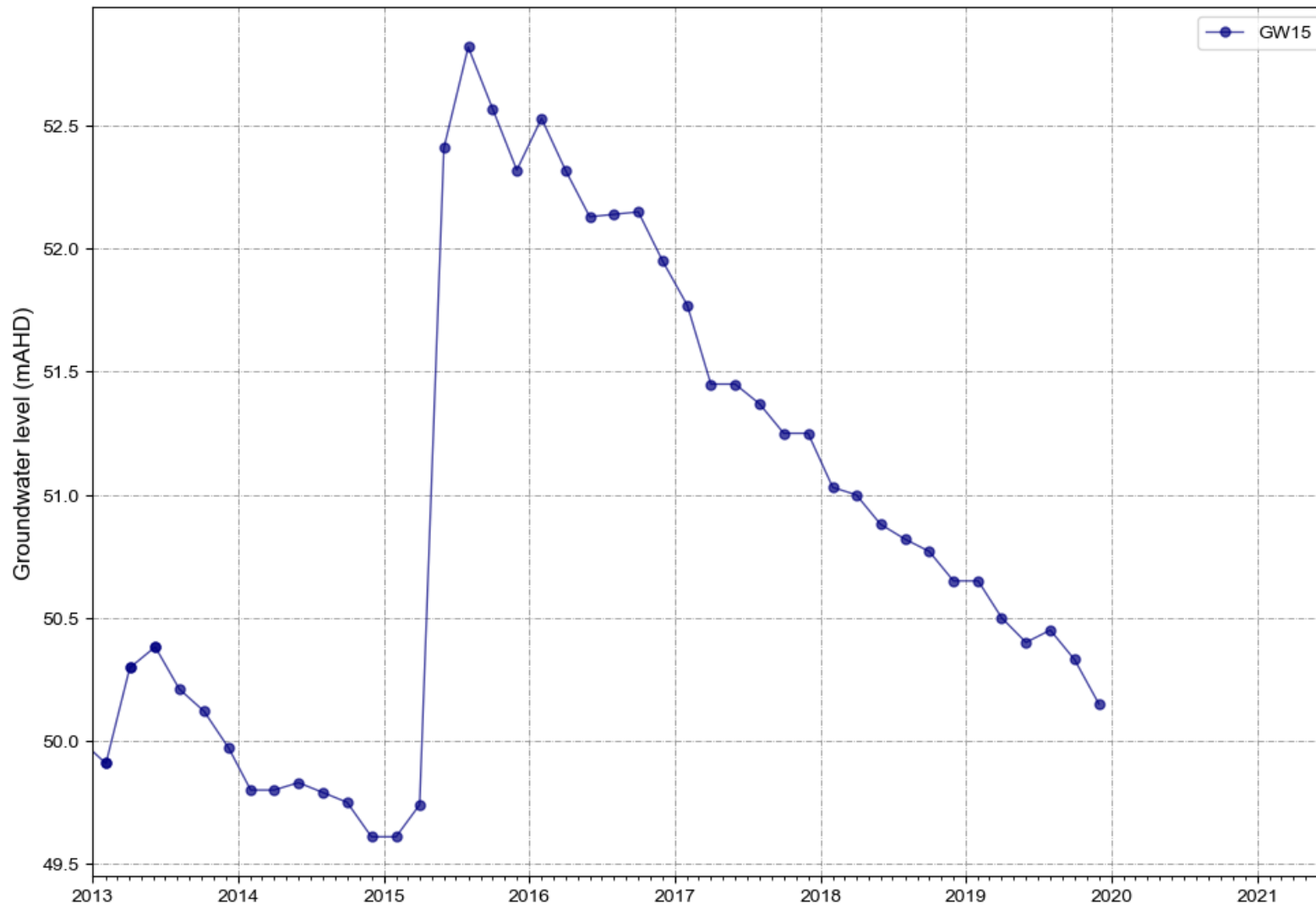
Figure A 47 GW15 water levels
