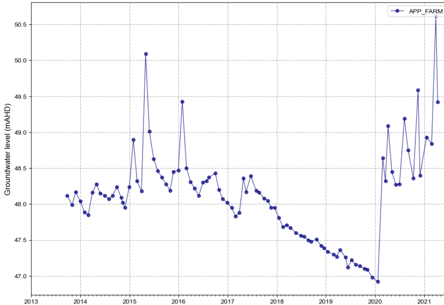
Figure A 45 APP_FARM water levels
