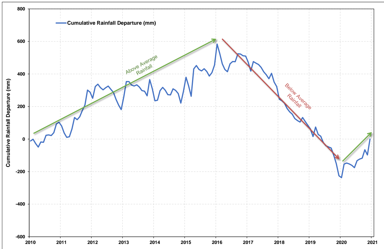
Figure 4.1 Cumulative rainfall departure (2010 – 2020)
