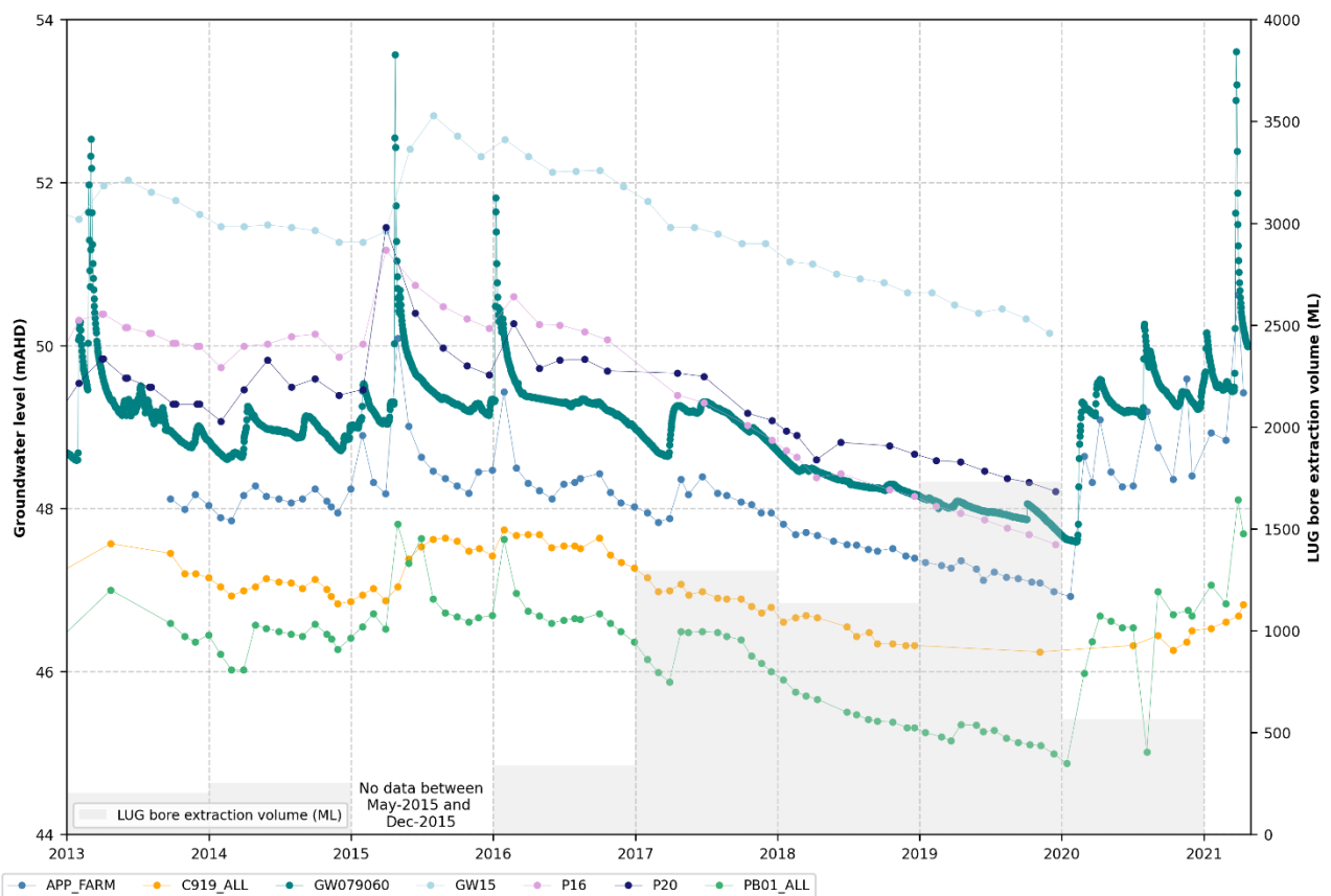
Figure 5.20 Wollombi Brook alluvium water levels compared to total annual extraction from LUG Bore
