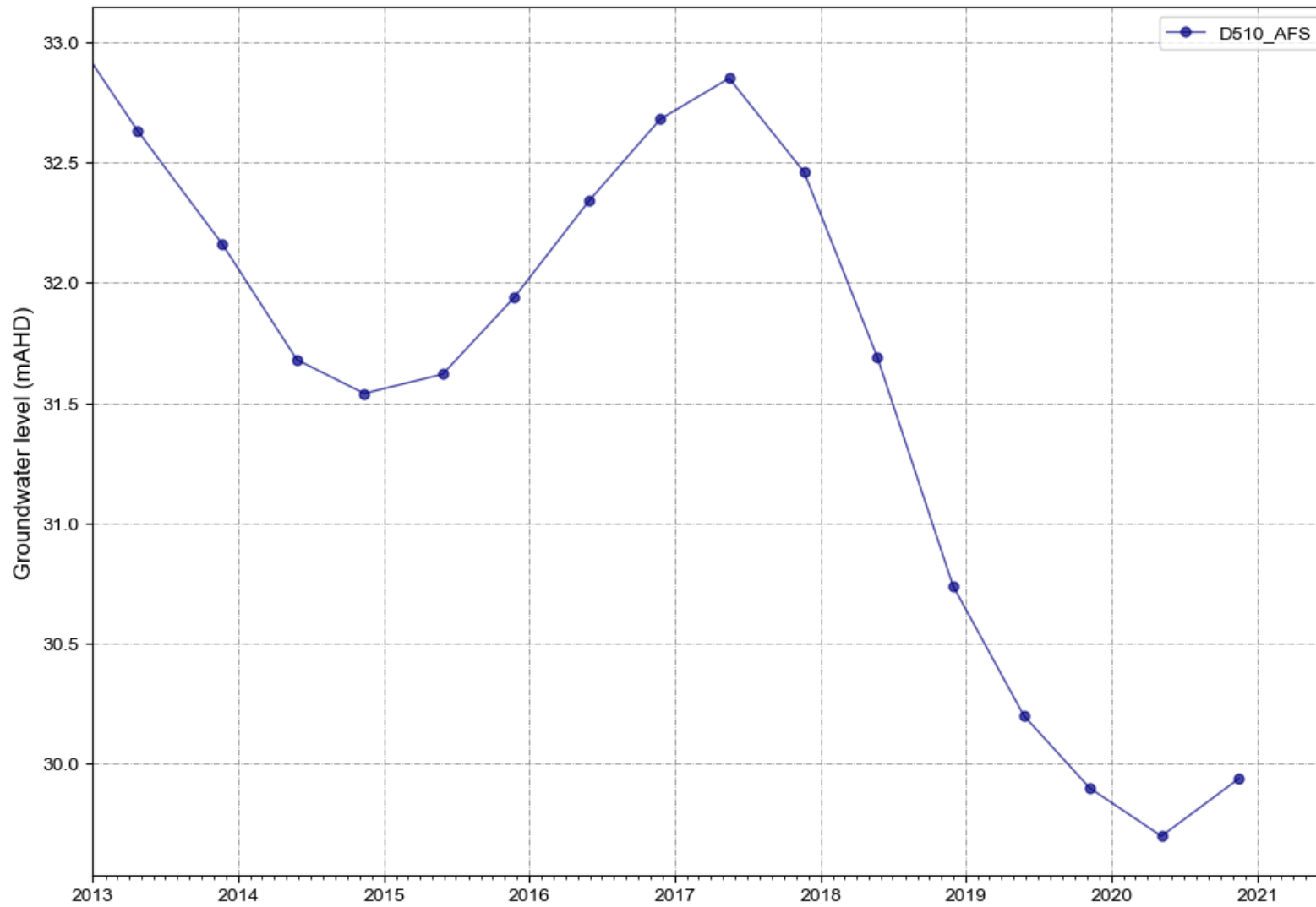
Figure A 34 D510_AFS water levels
