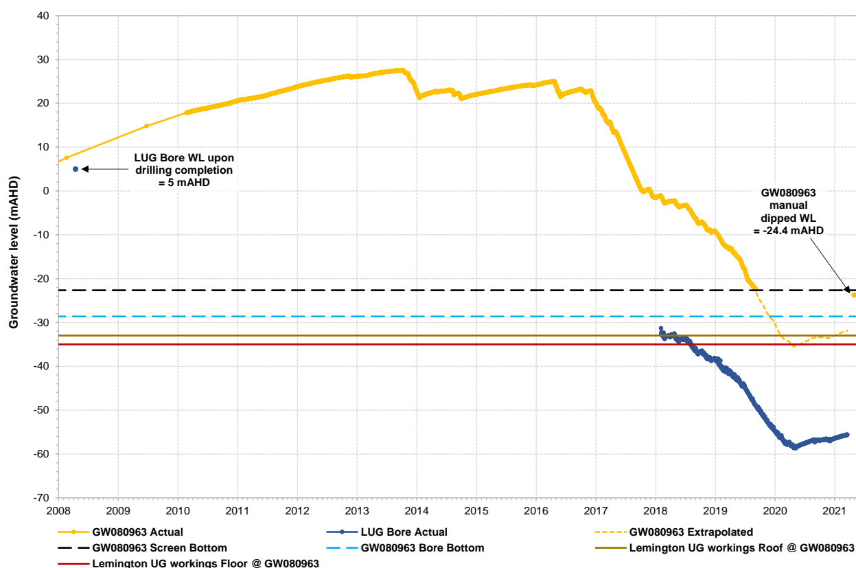
Figure 5.4 GW080963 extrapolated water levels with bore and workings' reference levels
