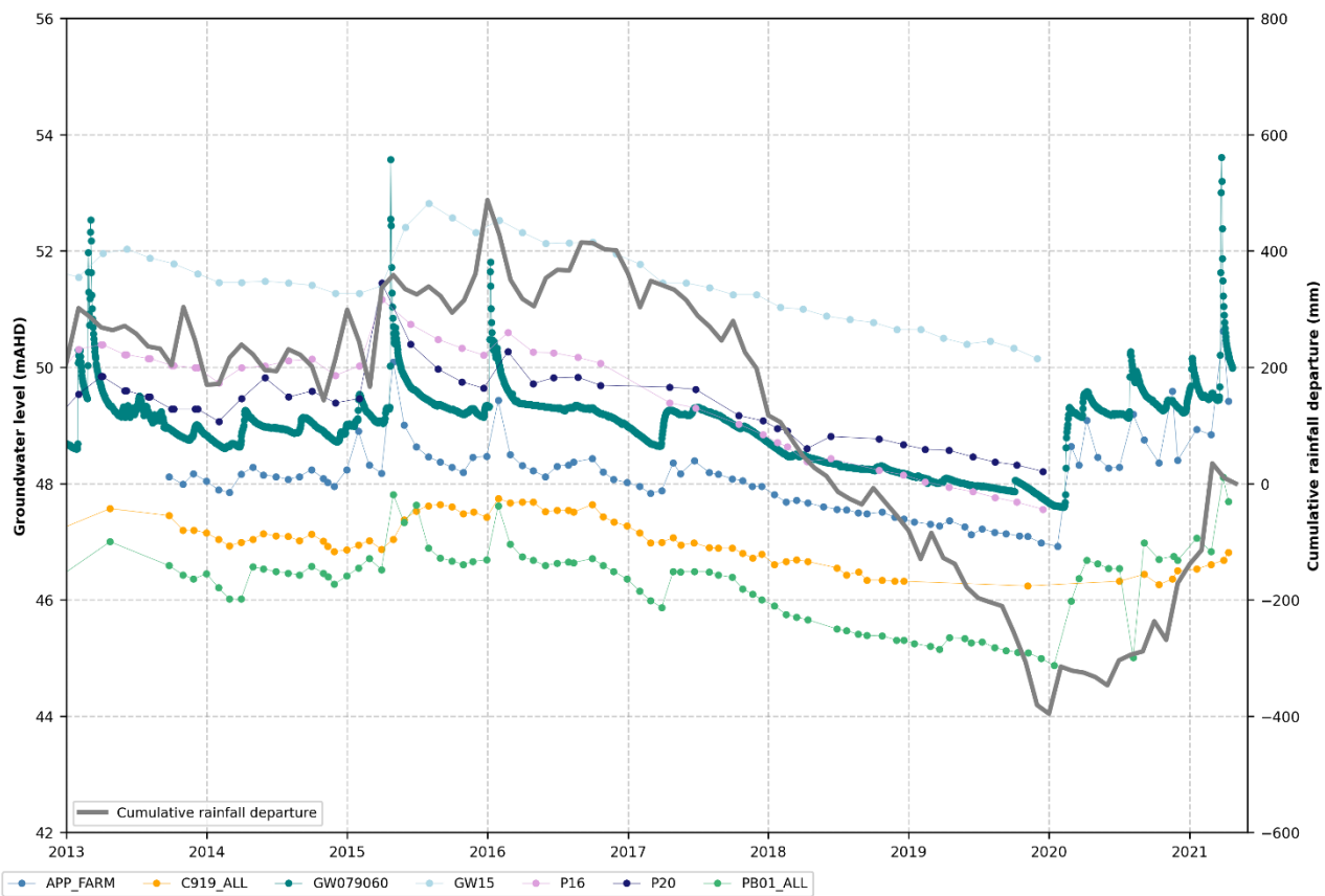
Figure 5.19 Wollombi Brook alluvium water levels compared to cumulative rainfall departure
