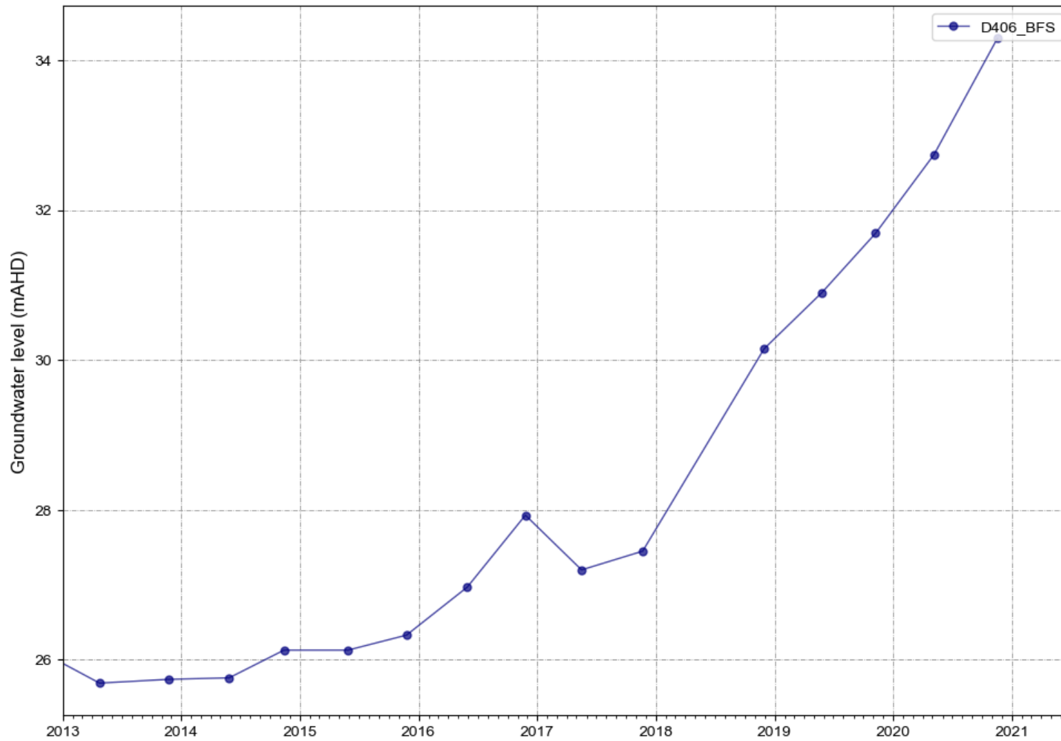
Figure A 28 D406_BFS water levels
