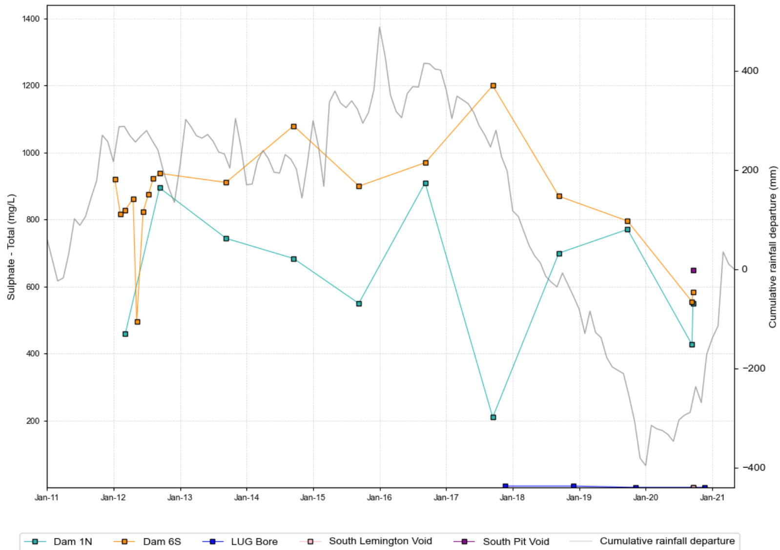
Figure B 12 MTW main surface water stores and LUG Bore, sulphate time series data
