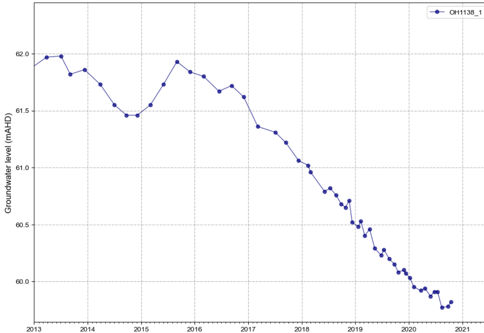
Figure A 14 OH1138_1 water levels
