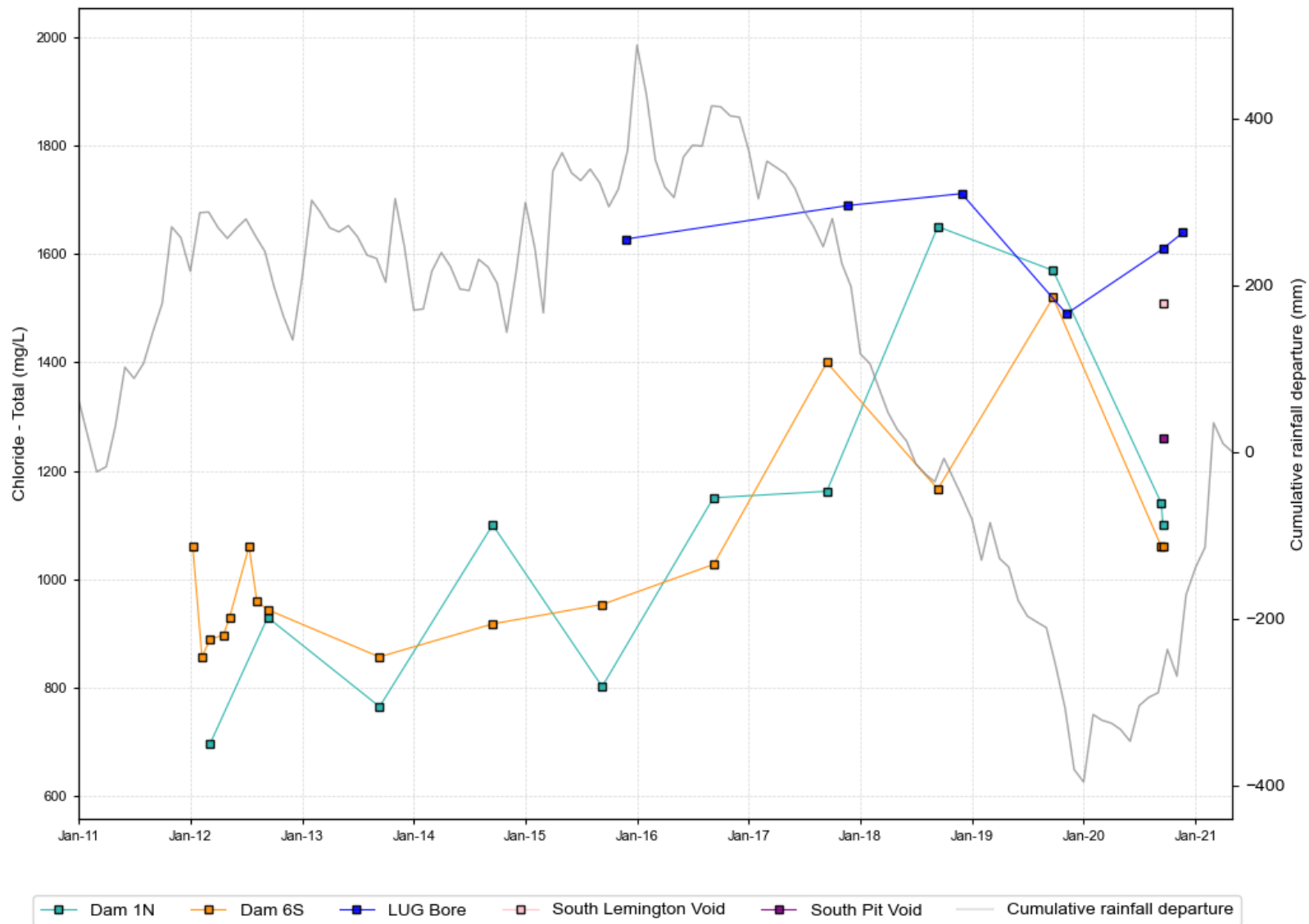
Figure B 5 MTW main surface water stores and LUG Bore, chloride time series data
