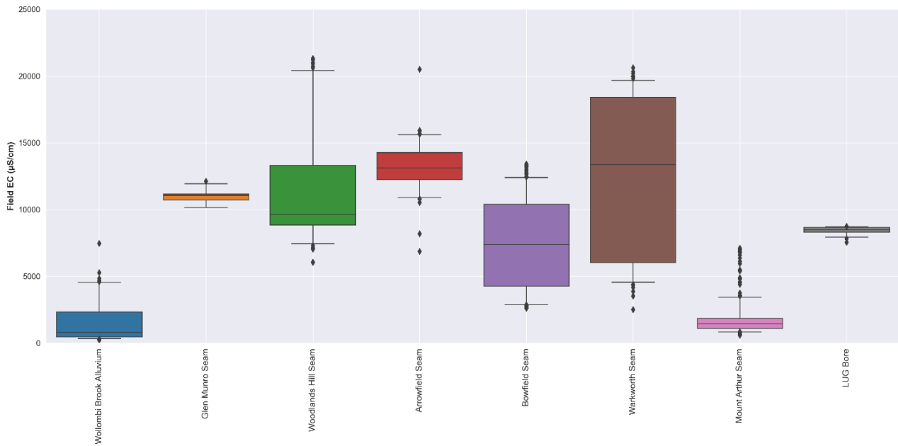
Figure 5.45 Box and whisker plot of EC for coal seams with data above Mount Arthur coal seam
