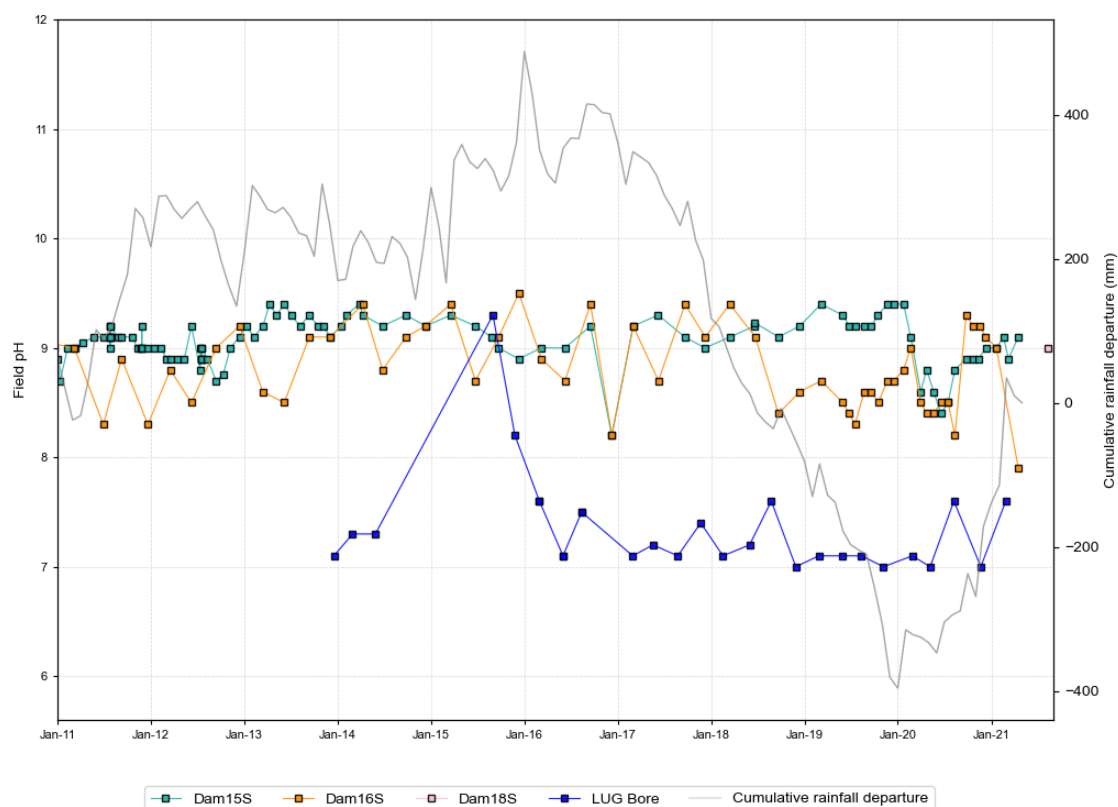
Figure 5.32 HVO main surface water stores and LUG Bore, pH time series data
