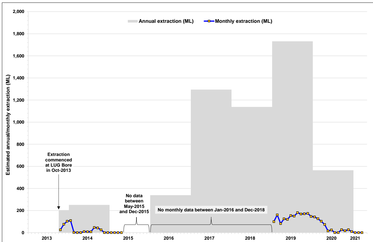
Figure 3.4 Total annual and monthly extraction at the LUG Bore
